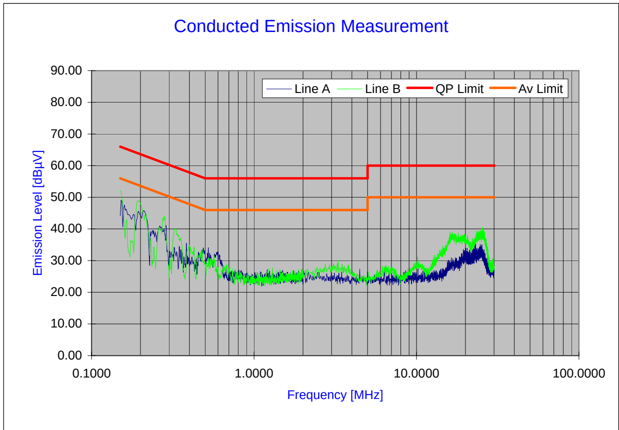
Plot 6-45. Line Conducted Plot with 802.11n (UNII Band III)
