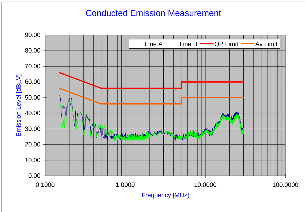
Plot 6-43. Line Conducted Plot with 802.11n (UNII Band I)
