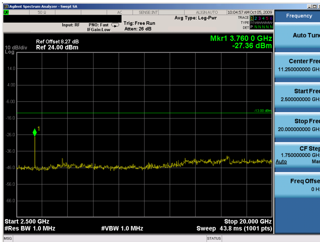
Plot 7-62. Conducted Spurious Plot (PCS CDMA Mode – Ch. 600)
