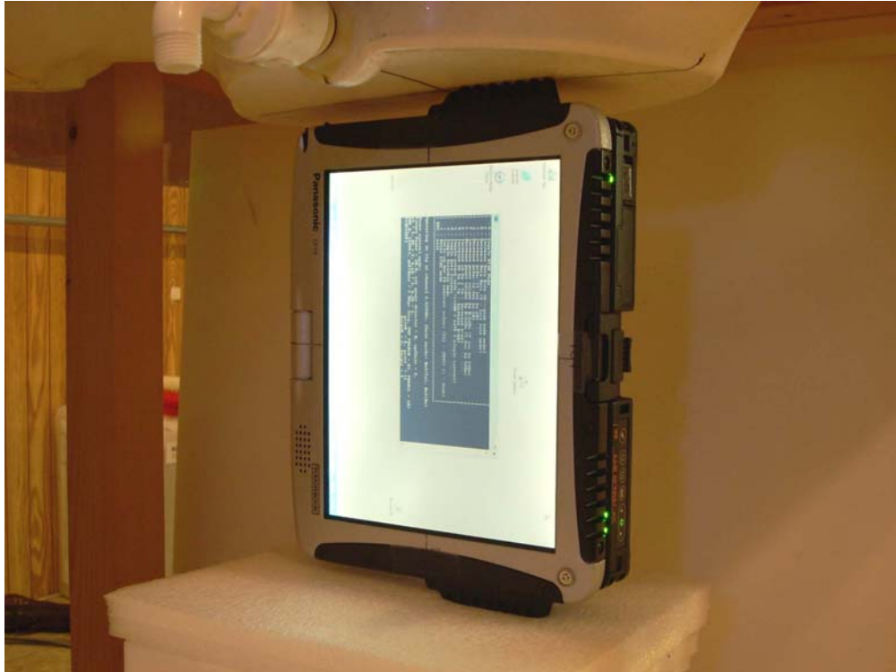
Figure 19-3 SAR Test Setup Photo 3 (Tablet Left)
