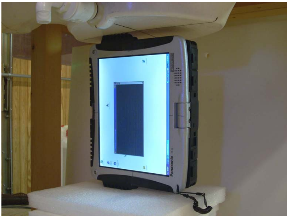
Figure 19-4 SAR Test Setup Photo 4 (Tablet Right)
