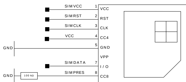
Figure 4 : SIM socket
