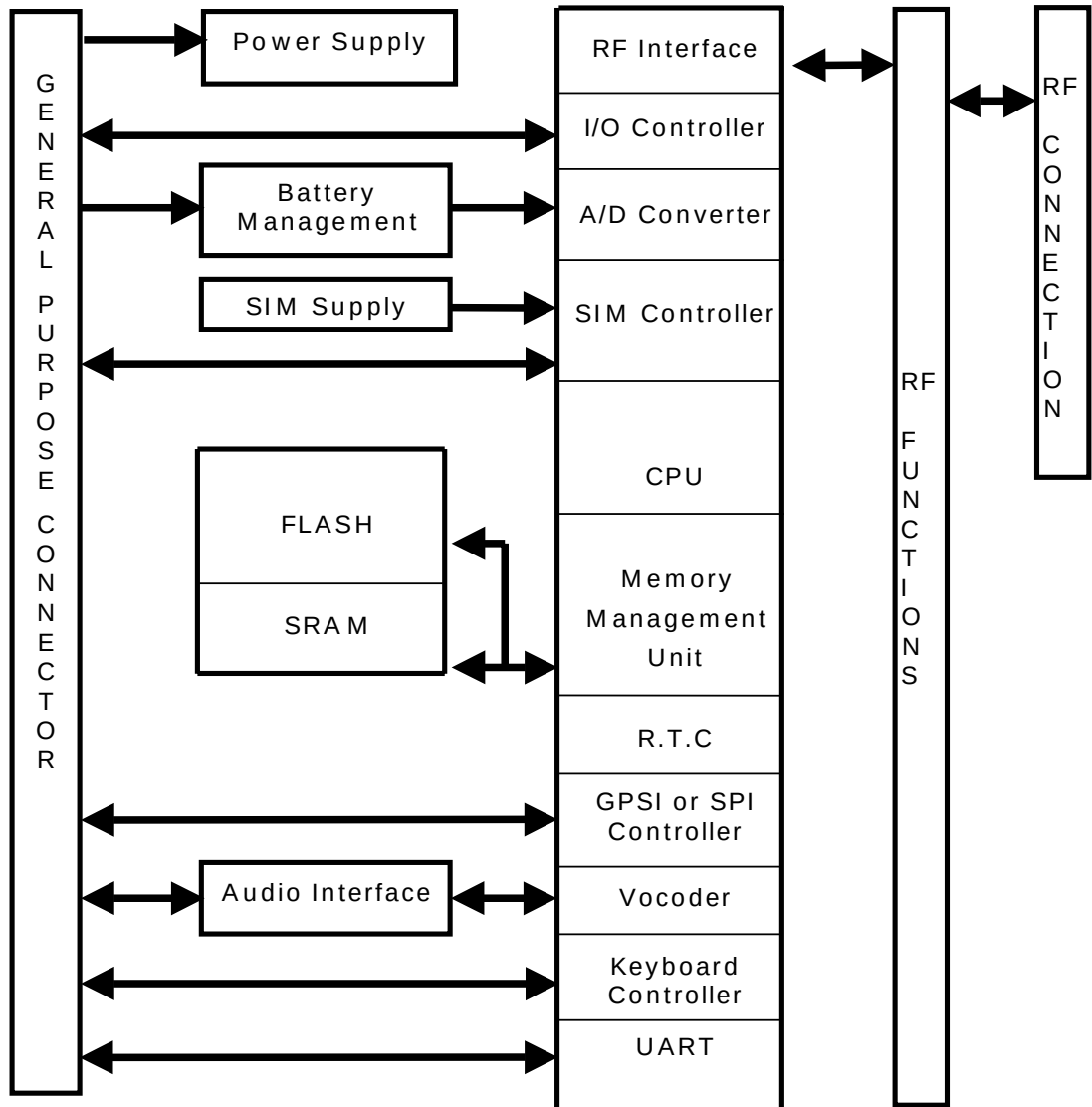
Figure 2 : Functional architecture
