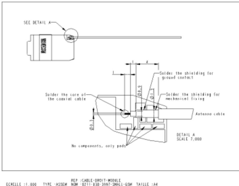
Figure 23 : antenna cable mounting guidelines
