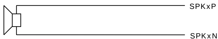
Figure 5 : SPK outputs (differential connection)
