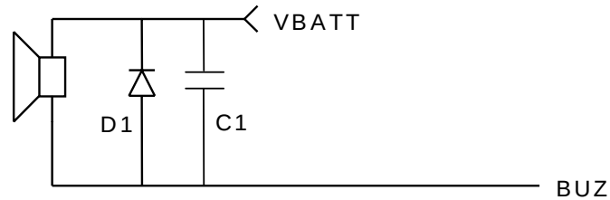
Figure 10 : Buzzer connection
