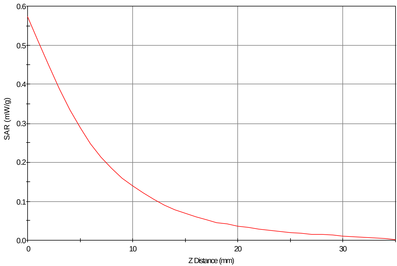
SAR - Z Axis at Hotspot x:46.0 y:-5.0
