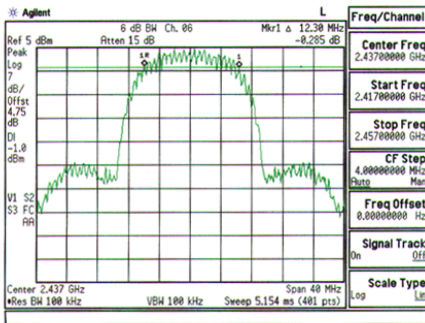
Plot A-2. 6dB Bandwidth Plot – Ch. 06
