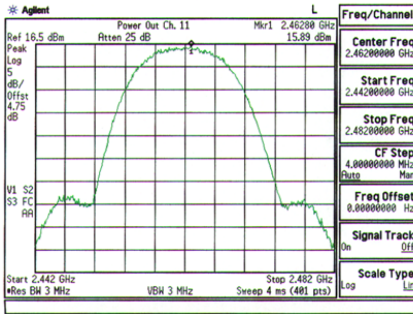
Plot A-6. Max. Output Power Plot – Ch. 11
