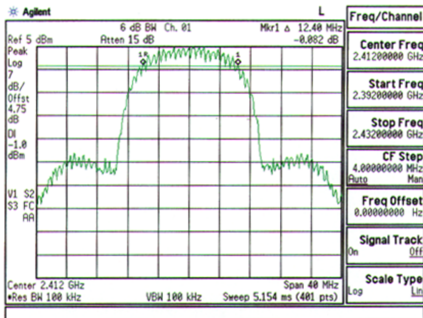
Plot A-1. 6dB Bandwidth Plot – Ch. 01
