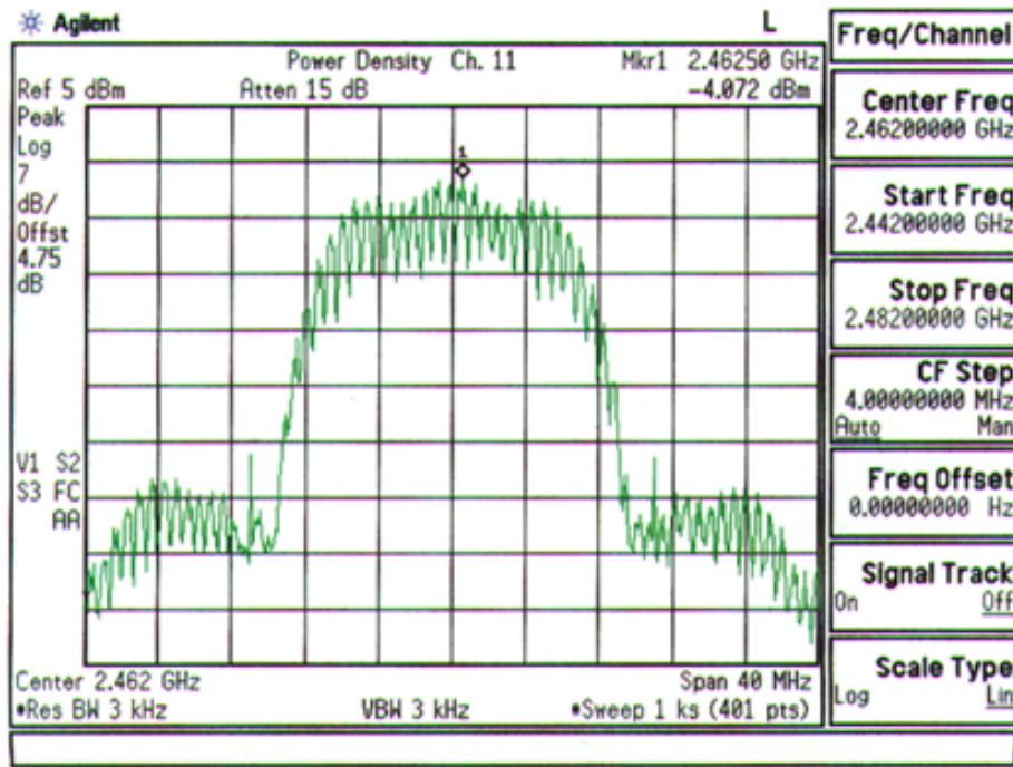
Plot A-9. Max. Power Density Plot – Ch. 11
