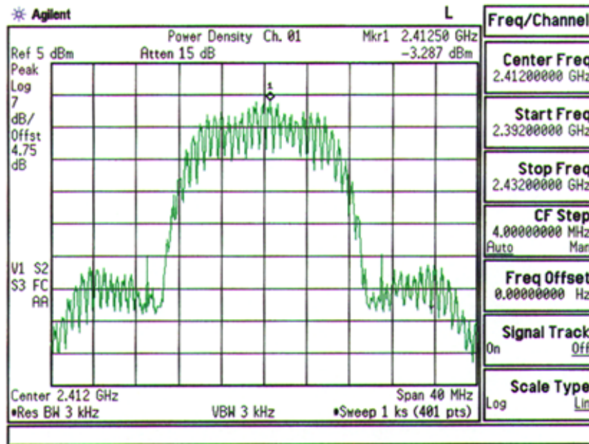
Plot A-7. Max. Power Density Plot – Ch. 01
