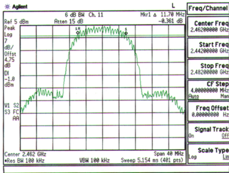
Plot A-3. 6dB Bandwidth Plot – Ch. 11
