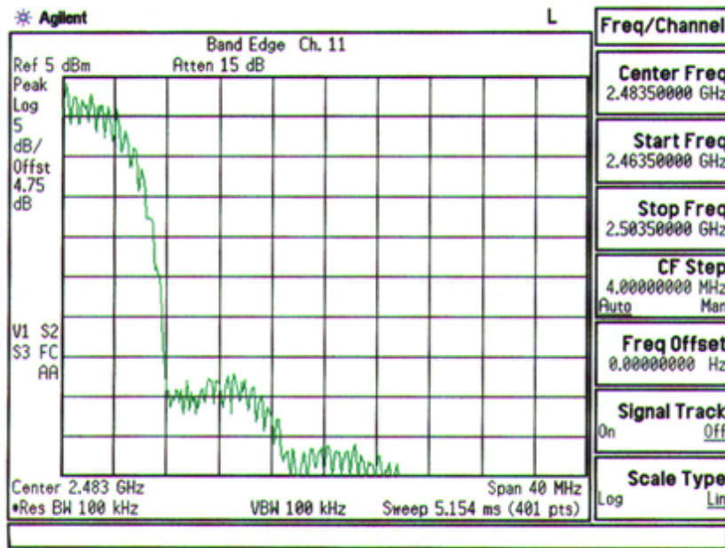
Plot A-11. Occupied Band Edge Plot – Ch. 11
