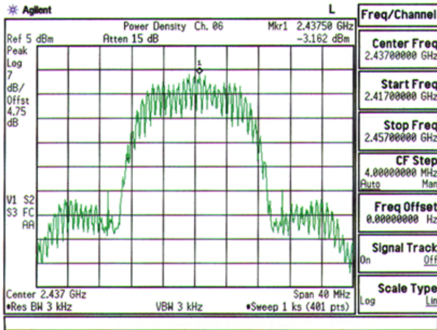
Plot A-8. Max. Power Density Plot – Ch. 06
