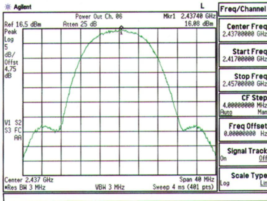
Plot A-5. Max. Output Power Plot – Ch. 06
