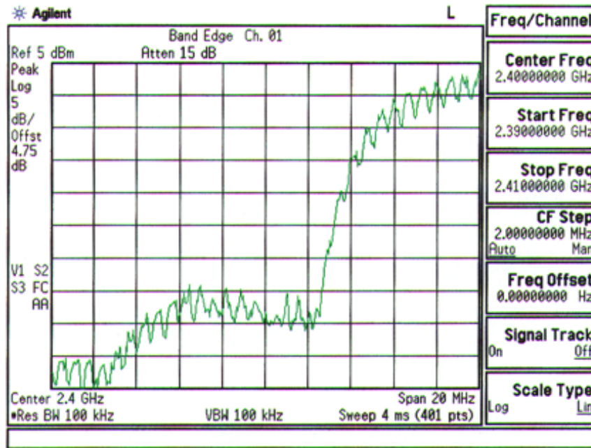
Plot A-10. Occupied Band Edge Plot – Ch. 01
