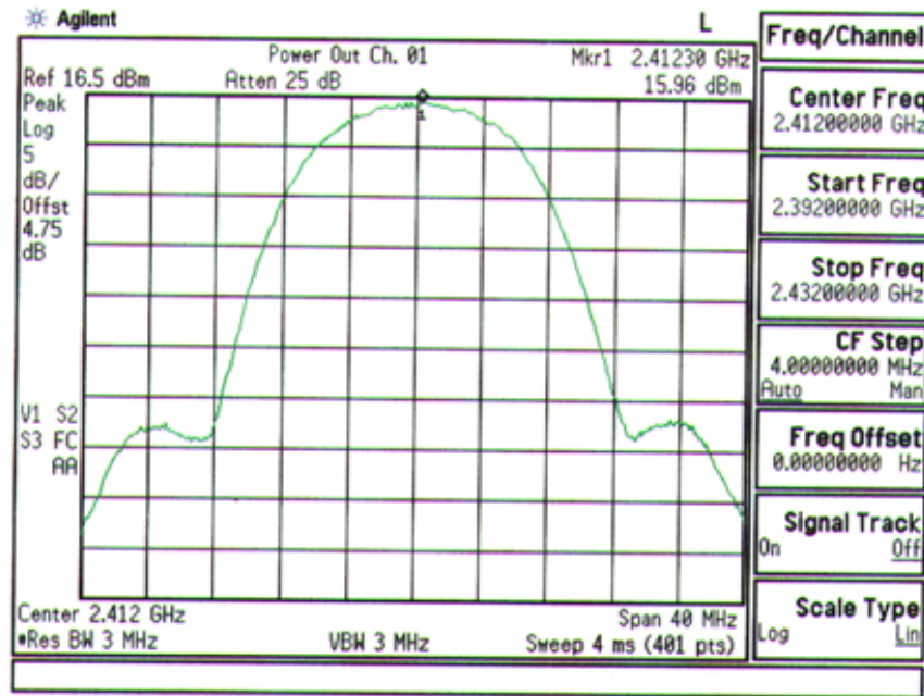
Plot A-4. Max. Output Power Plot – Ch. 01
