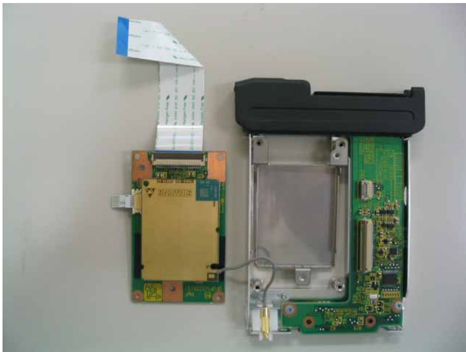
EGPRS Module Adapter View-2
