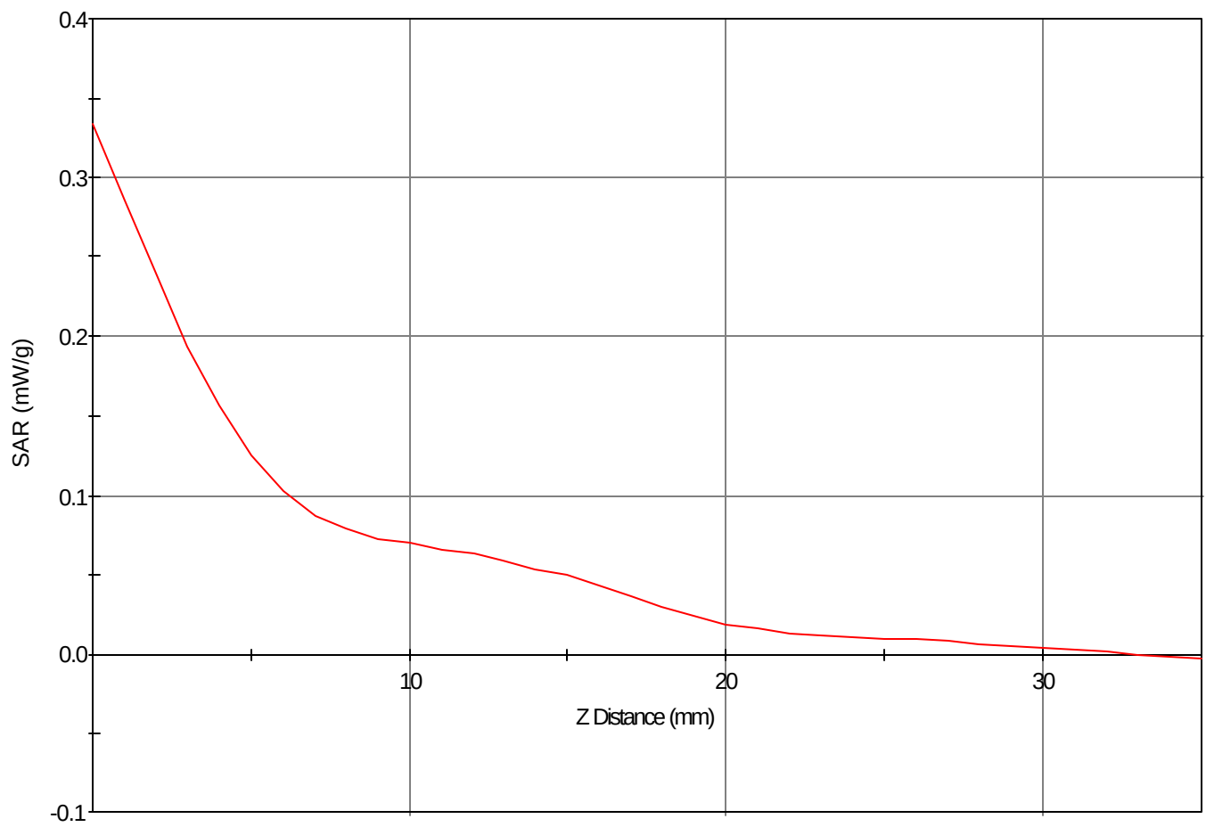
SAR - Z Axis at Hotspot x:-25.0 y:4.0
