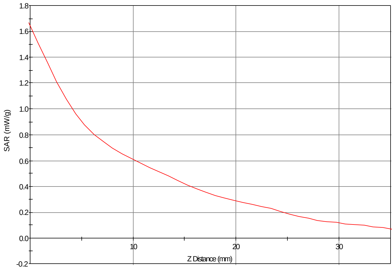
SAR - Z Axis at Hotspot x:-44.0 y:-11.0
