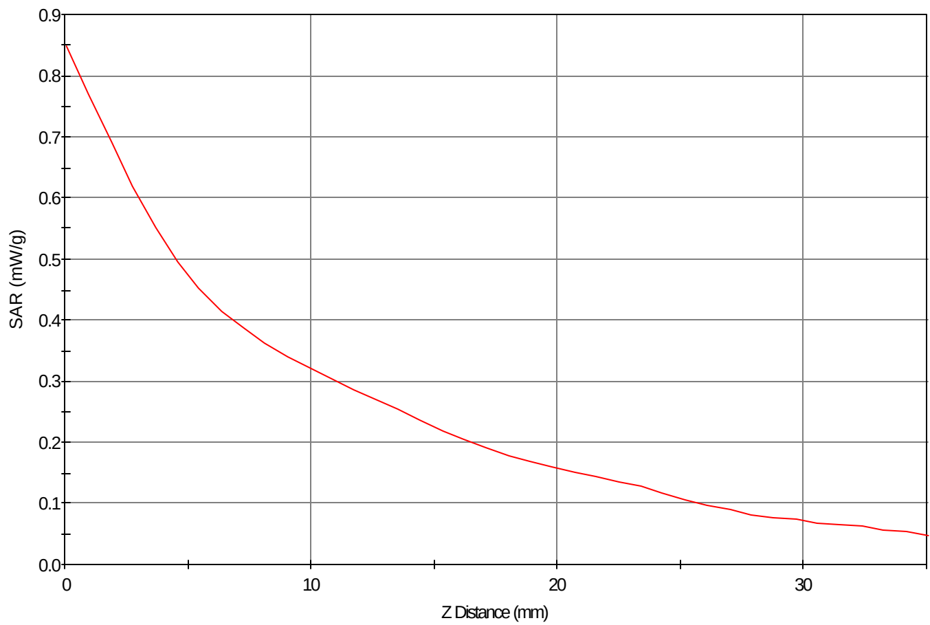
SAR - Z Axis at Hotspot x:-48.0 y:11.0
