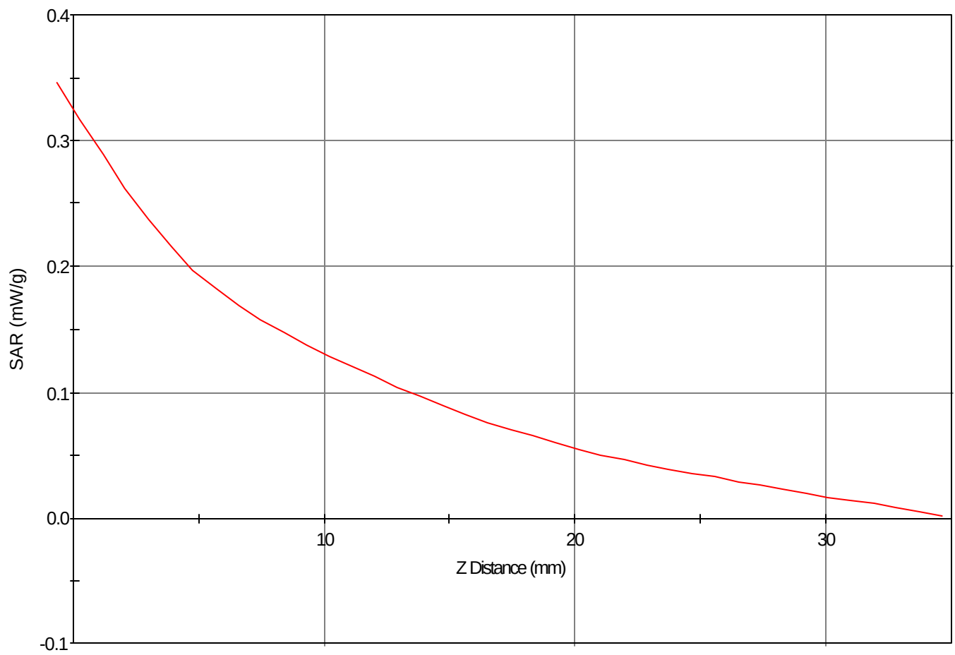
SAR - Z Axis at Hotspot x:-8.0 y:21.0
