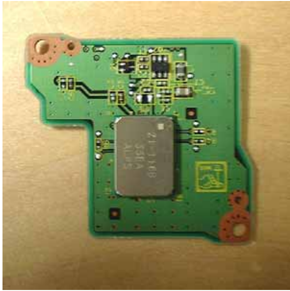
Top View of Bluetooth Module with Daughter-Board
