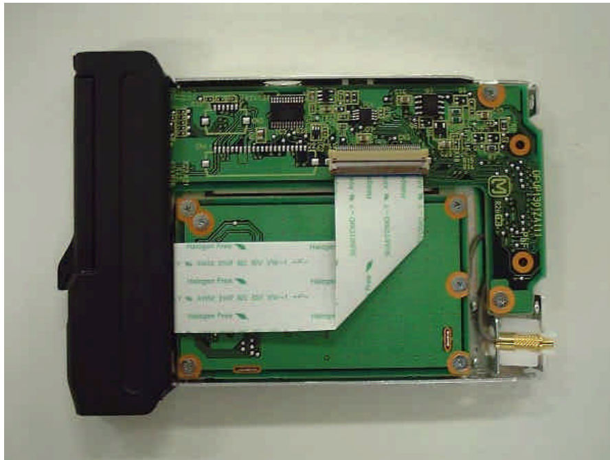
SB555 Module Adapter View-1
