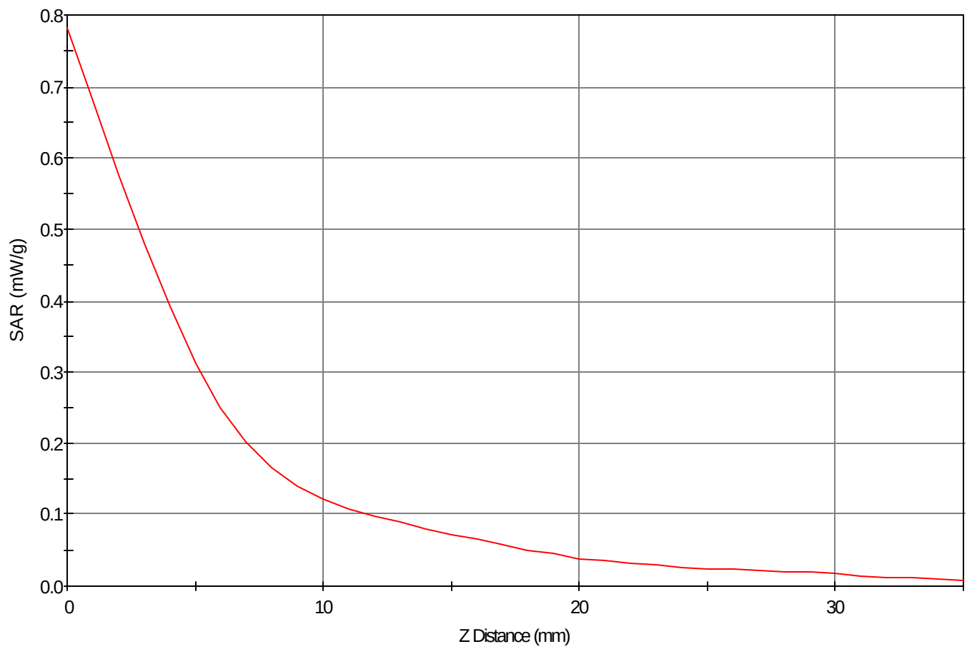
SAR - Z Axis at Hotspot x:-18.0 y:2.0
