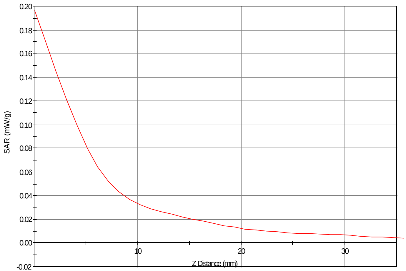
SAR - Z Axis at Hotspot x:29.0 y:-10.0
