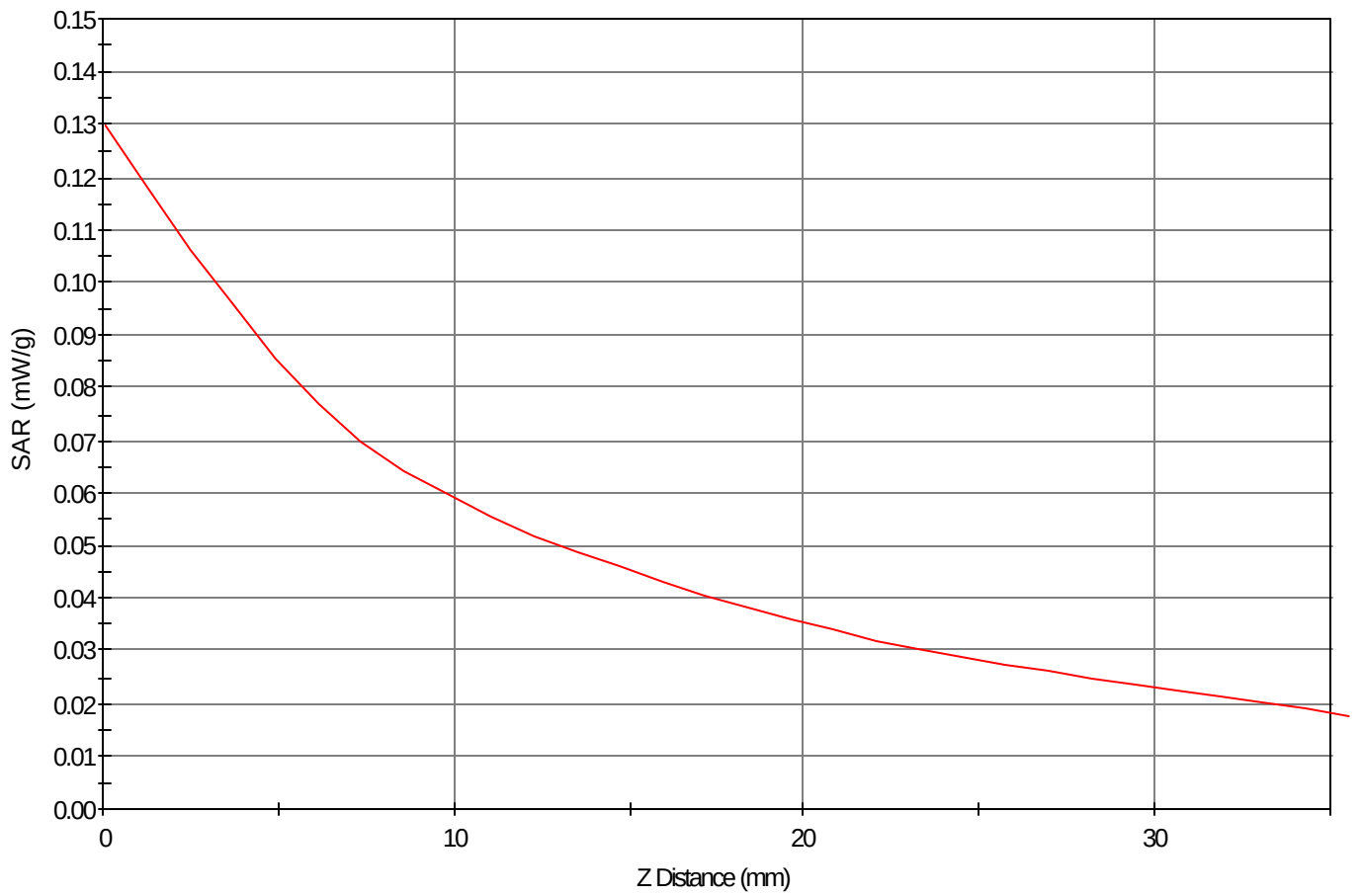
SAR - Z Axis at Hotspot x:-57.0 y:-37.0
