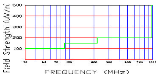
Figure A-8. Radiated limits at 3 meters.
