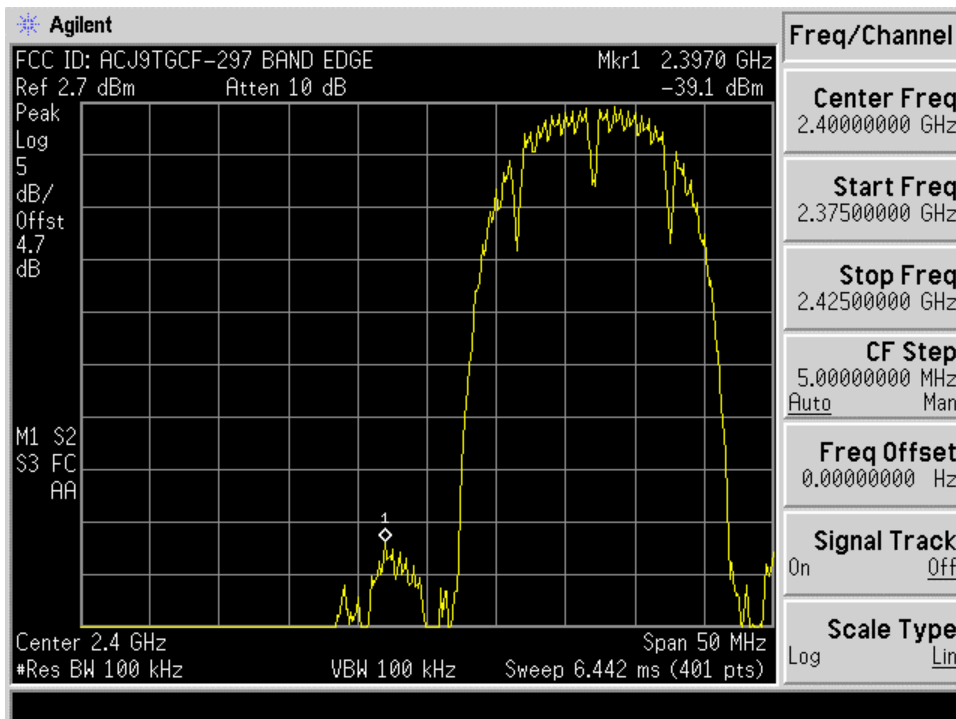
Plot A.1 Occupied Band Edge Ch. 01
