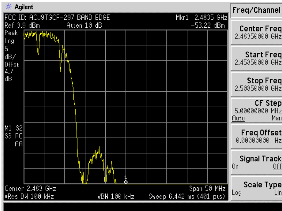
Plot A.2 Occupied Band Edge Ch. 11
