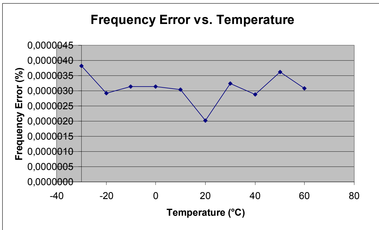
Diagram Frequency Error vs. Temperature
