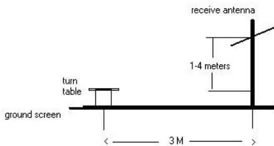
Figure 2. Diagram of 3-meter outdoor test range
