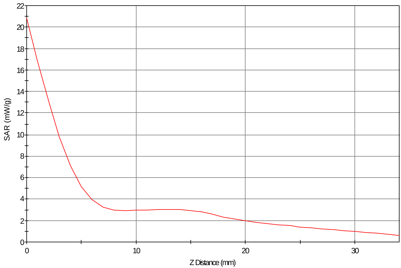
SAR - Z Axis at Hotspot x:33.0 y:14.0
