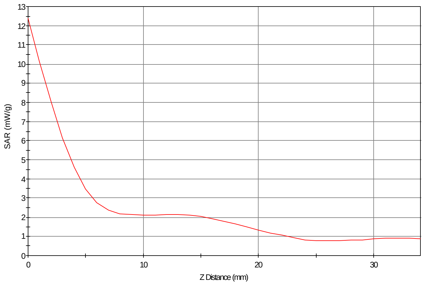
SAR - Z Axis at Hotspot x:-12.0 y:-10.0
