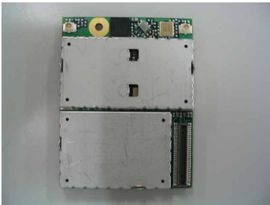
EM5625D module Bottom View
