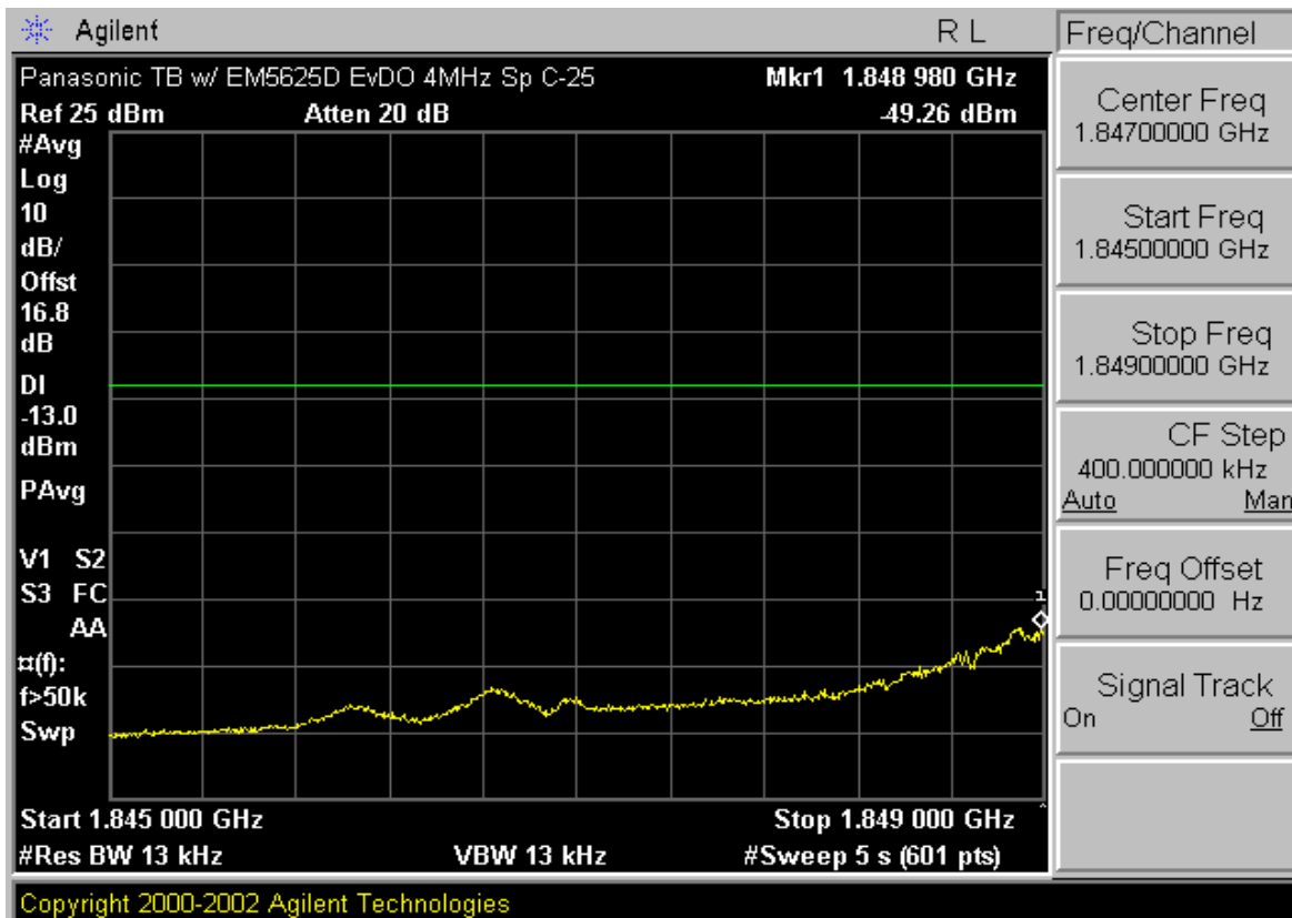
Plot A-16. 4MHz Span Plot (PCS CDMA EvDO Mode – Ch. 25)
