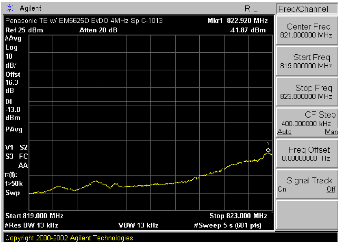
Plot A-4. 4MHz Span Plot (Cellular CDMA EvDO Mode – Ch. 1013)
