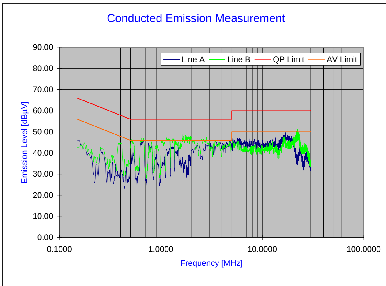
Plot 6-25. Line Conducted Plot with 802.11b
