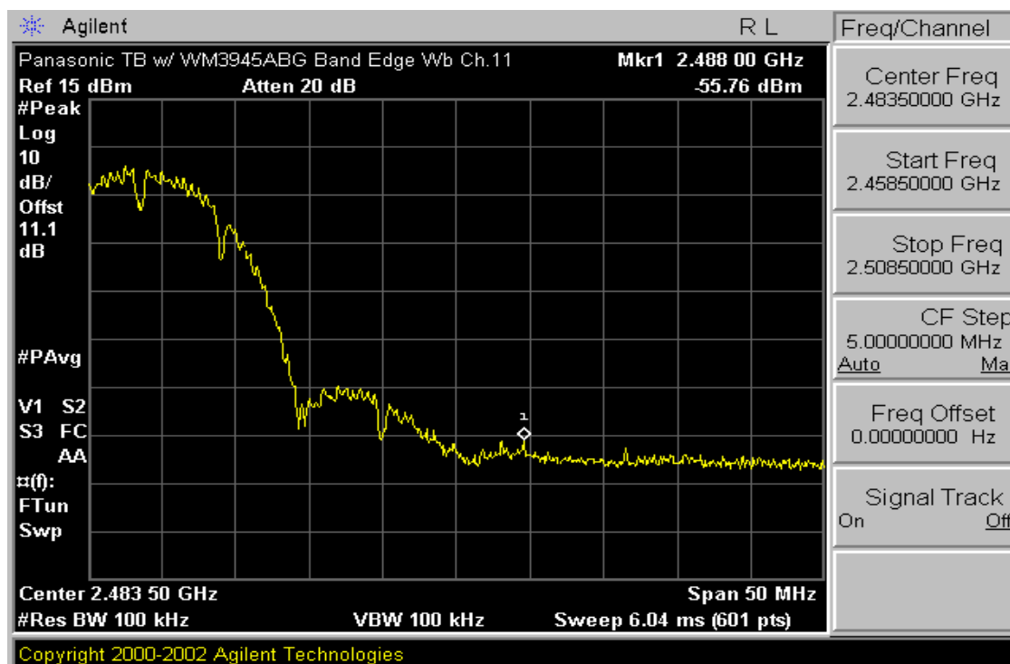
Plot 6-20. Band Edge Plot (802.11b – Ch. 11)
