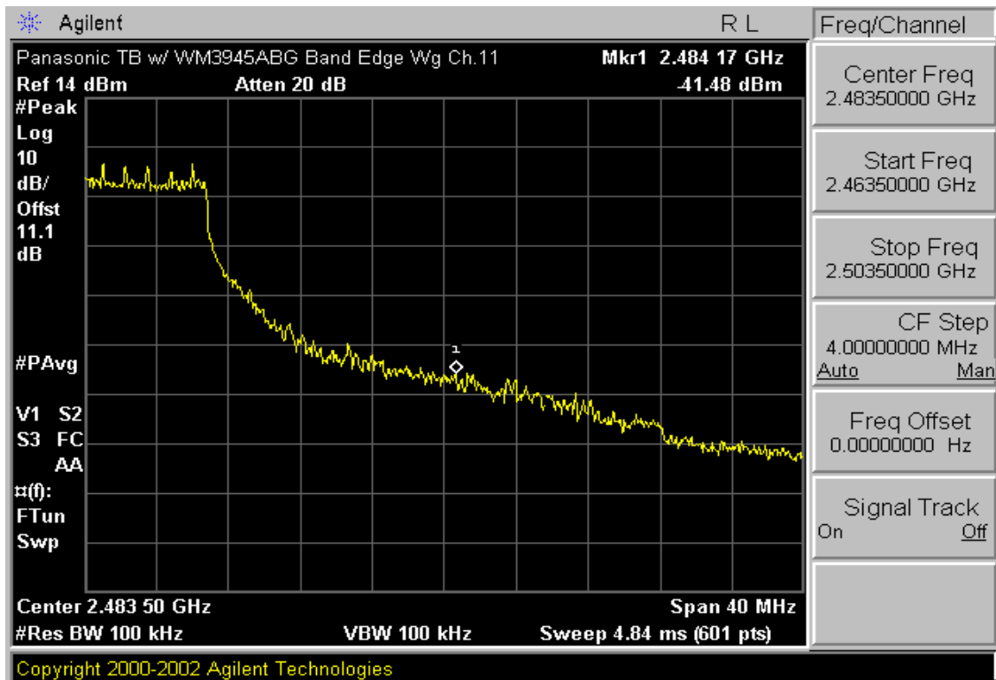
Plot 6-22. Band Edge Plot (802.11g - Ch. 11)
