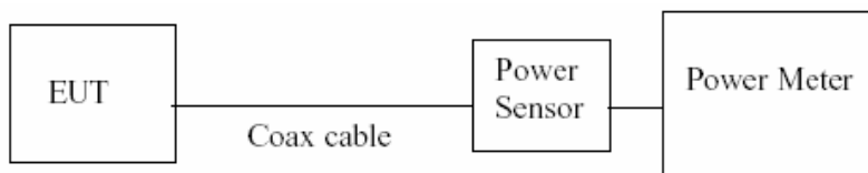
Figure 6-3. Test Instrument & Measurement Setup
