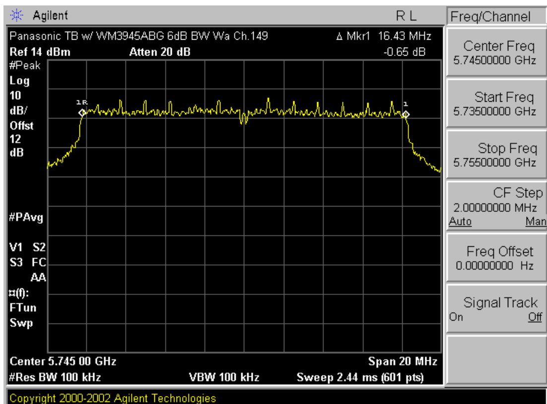
Plot 6-7. 6dB Bandwidth Plot (802.11a – Ch. 149)
