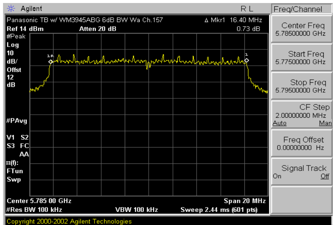
Plot 6-8. 6dB Bandwidth Plot (802.11a – Ch. 157)
