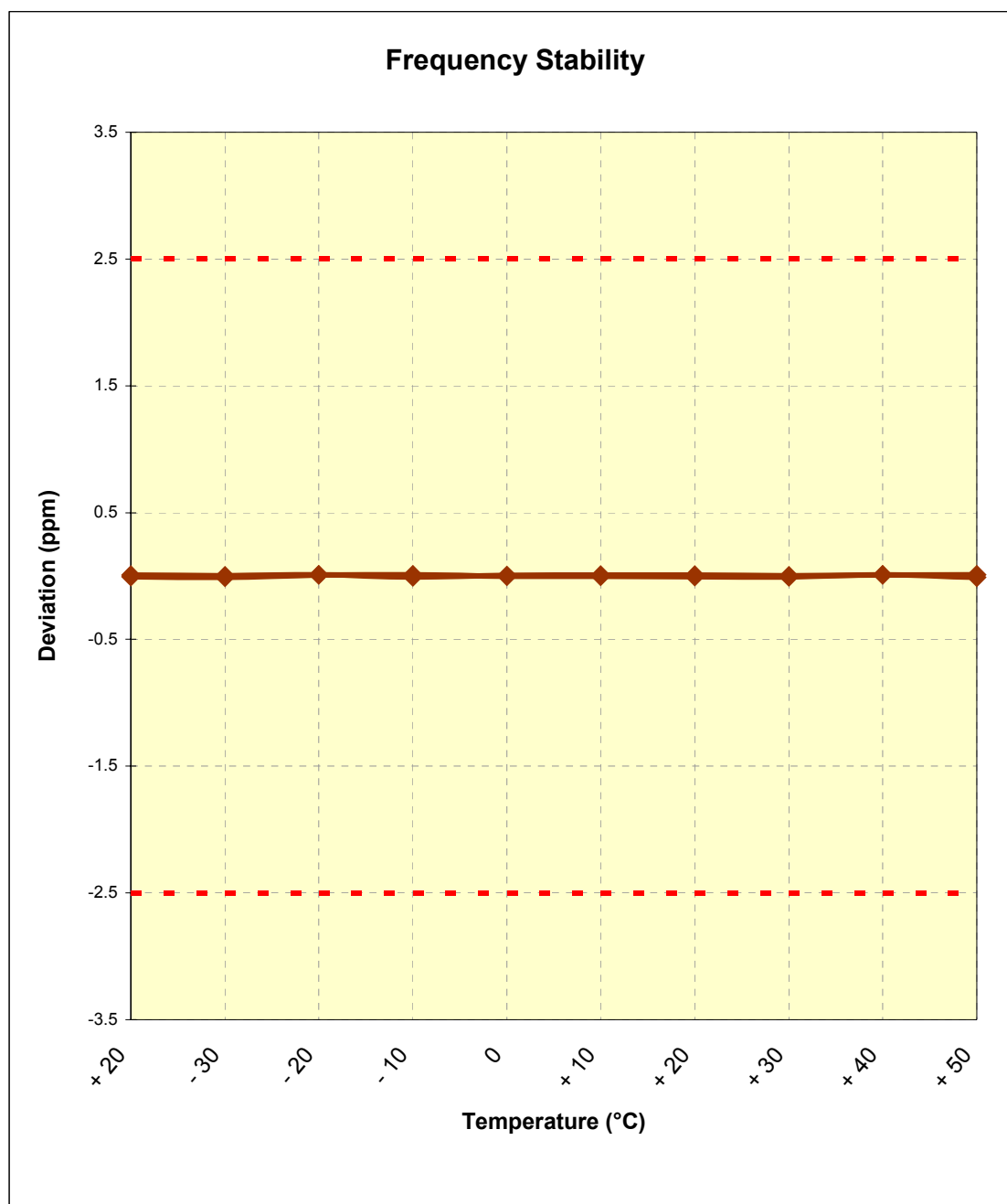
Figure 6-7. Frequency Stability Graph (PCS CDMA Mode – Ch. 600)
