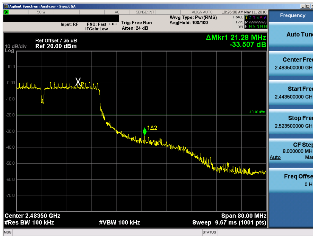
Plot 6-14. Band Edge Plot at 108/120Mbps (MCS5) (802.11n (40MHz) – Ch. 9)
