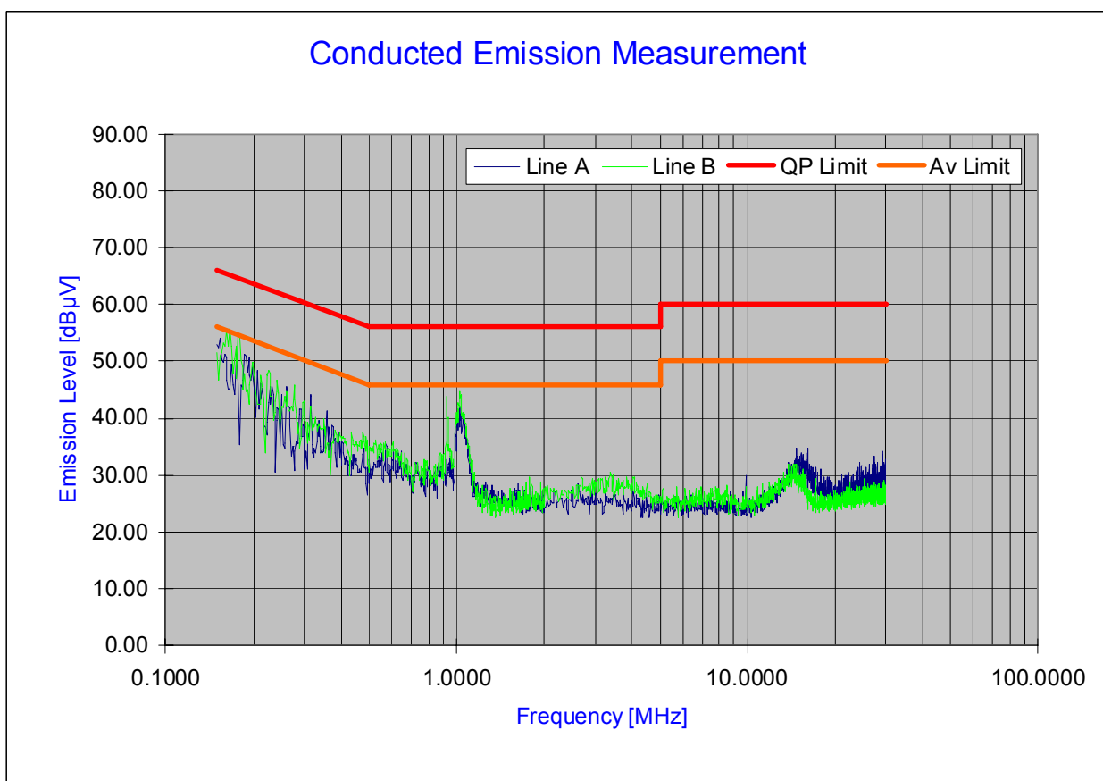
Plot 6-21. Line Conducted Plot with 802.11b
