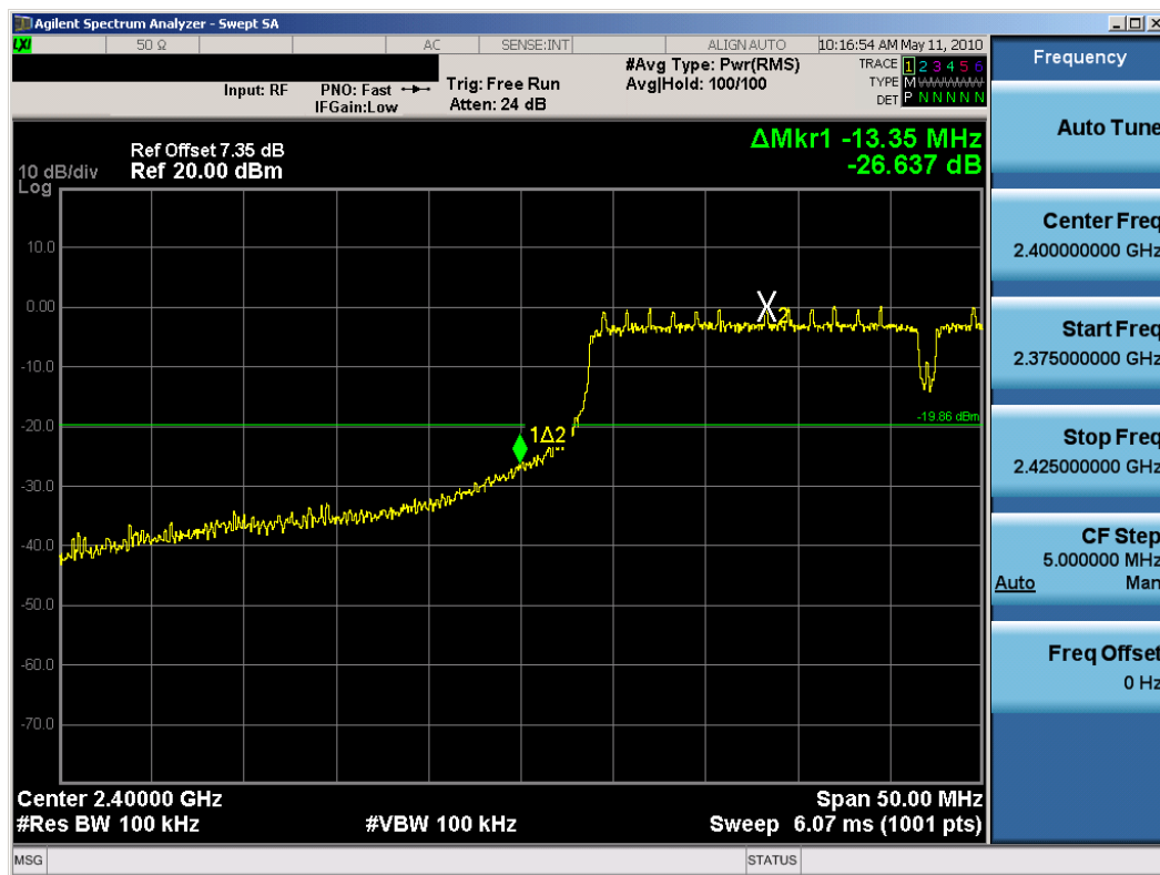
Plot 6-13. Band Edge Plot at 108/120Mbps (MCS5) (802.11n (40MHz) – Ch. 3)
