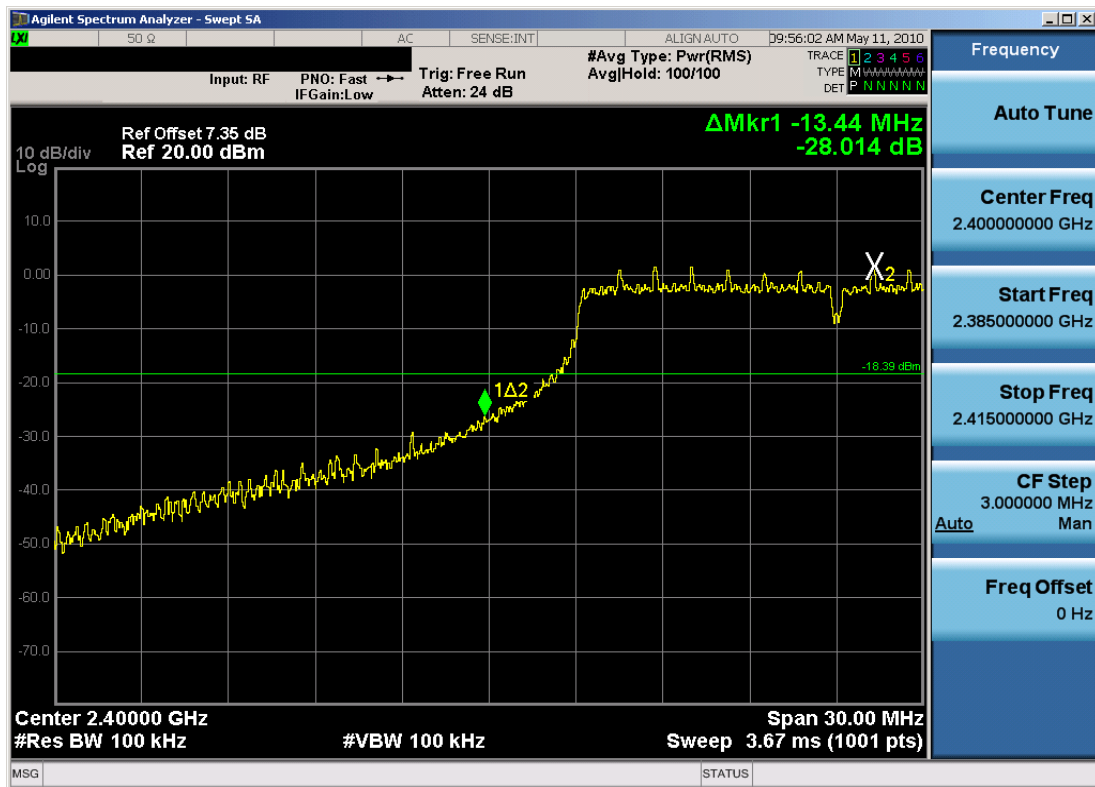
Plot 6-11. Band Edge Plot at 6.5/7.2Mbps (MCS0) (802.11n (20MHz) – Ch. 1)
