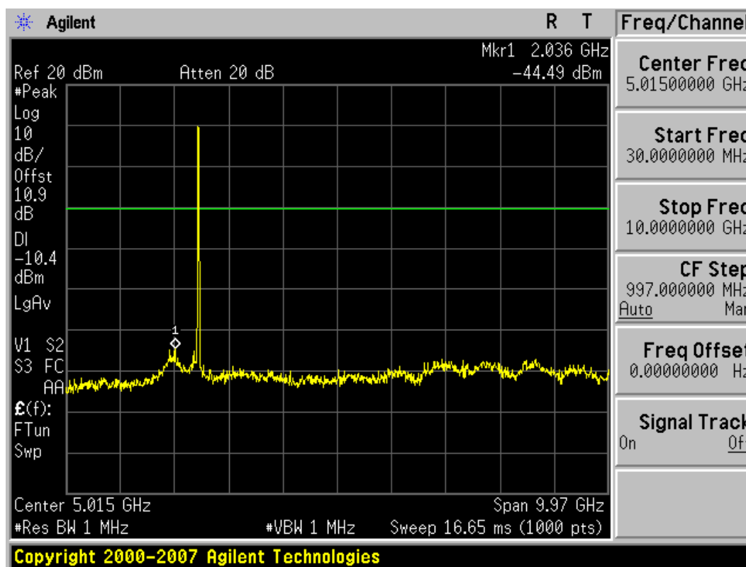
Plot 6-57. Conducted Spurious Plot (802.11b – Ch. 11) – Aux Antenna
