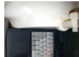
Figure 14.4 Body SAR Test Setup
