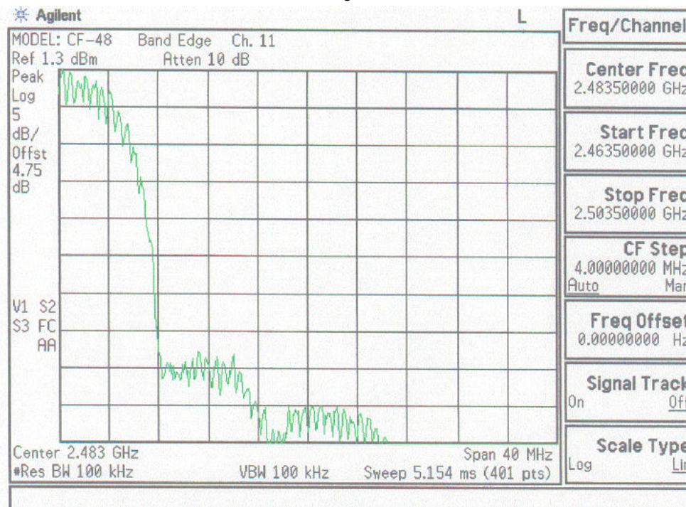
Plot A-12. BandEdge Plot – Ch.11
