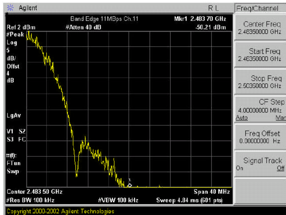
Plot A.X Occupied BandEdge 11 Mbps Ch. 11
