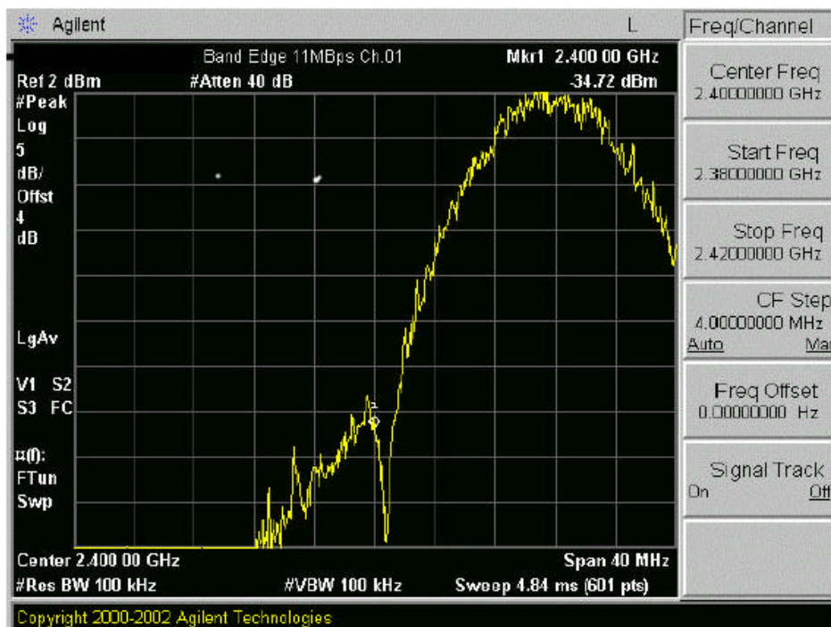
Plot A.X Occupied BandEdge 11 Mbps Ch. 01
