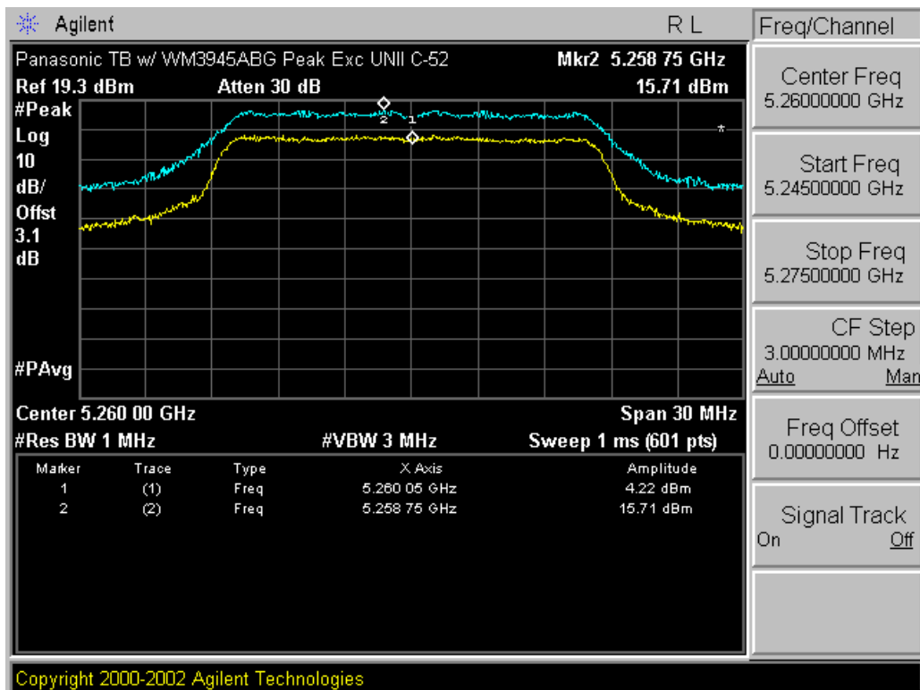
Plot A-16. Peak Excursion Ratio Plot – Ch. 52
