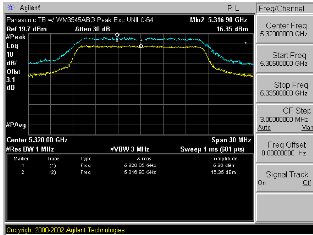
Plot A-17. Peak Excursion Ratio Plot – Ch. 64
