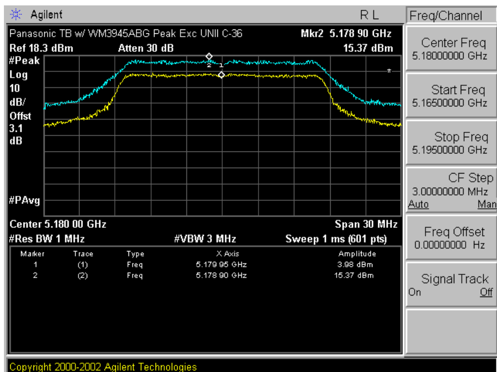
Plot A-15. Peak Excursion Ratio Plot – Ch. 36
