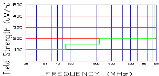
Figure A-11. Radiated limits at 3 meters.
