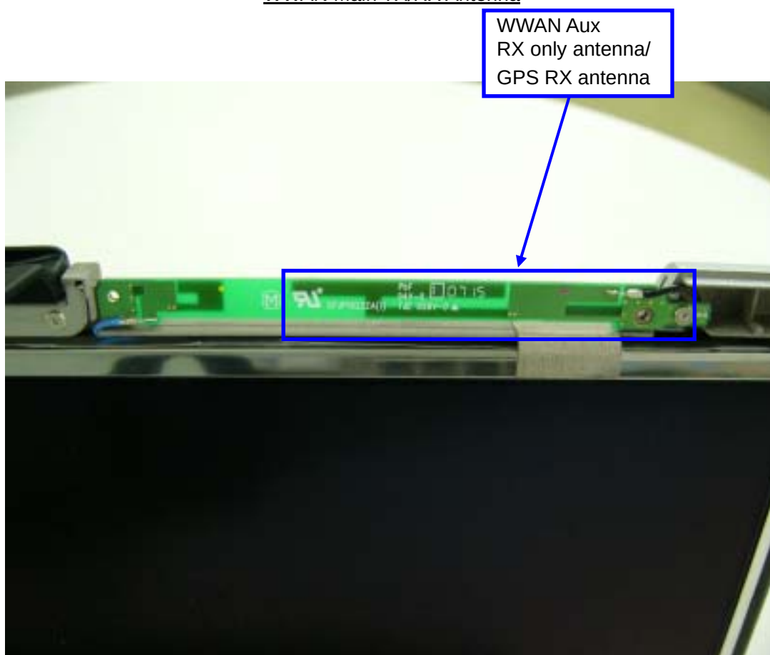
WWAN AUX RX only Antenna/GPS RX antenna
