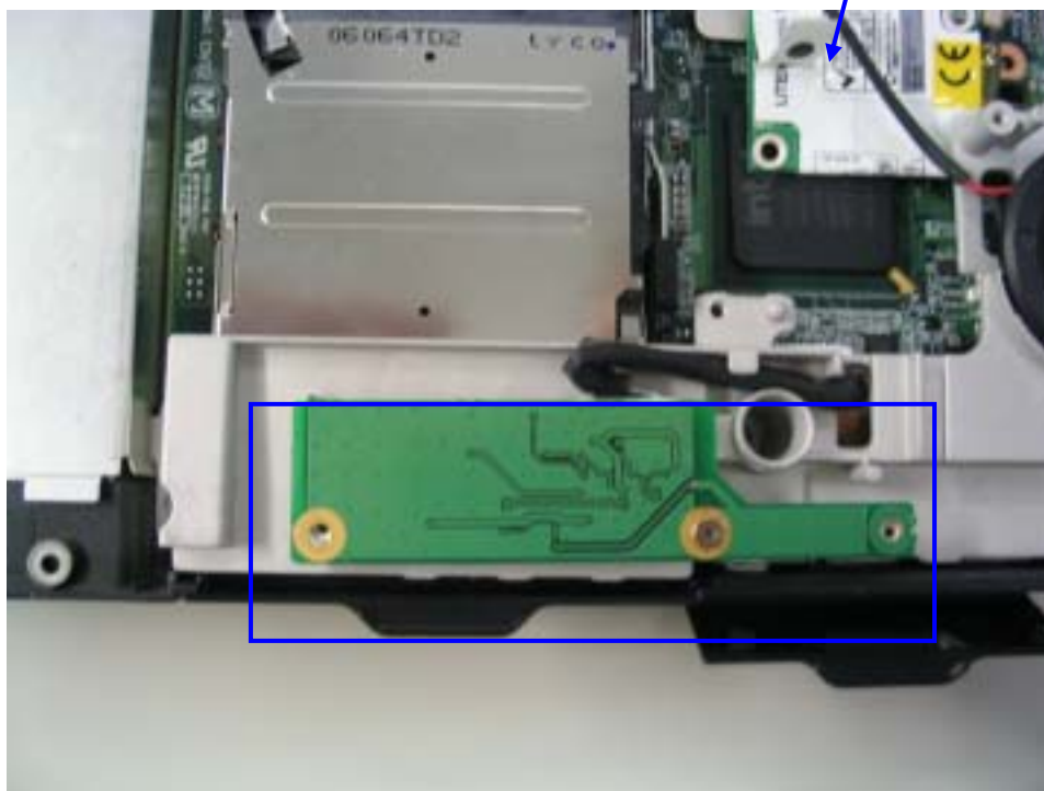
Bluetooth Card Magnified View (PWB removed)
