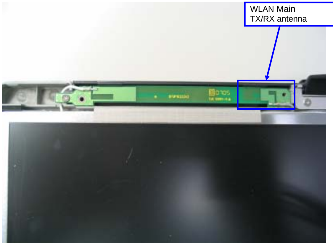
WLAN Main antenna magnified view
