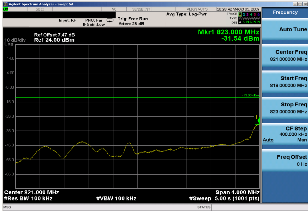
Plot 7-49. 4MHz Span Plot (Cellular CDMA Mode – Ch. 1013)
