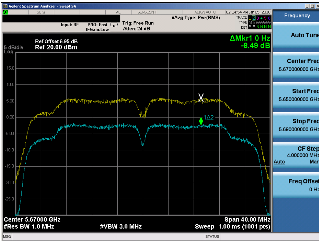
Plot 6-73. Peak Excursion Ratio Plot (802.11n (UNII) – Ch. 134) – Chain A
