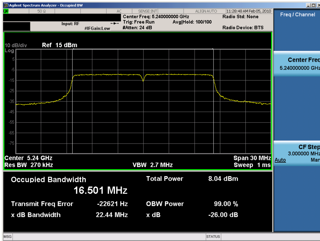
Plot 6-3. 26dB Bandwidth Plot (802.11a (UNII) – Ch. 48) – Chain A
