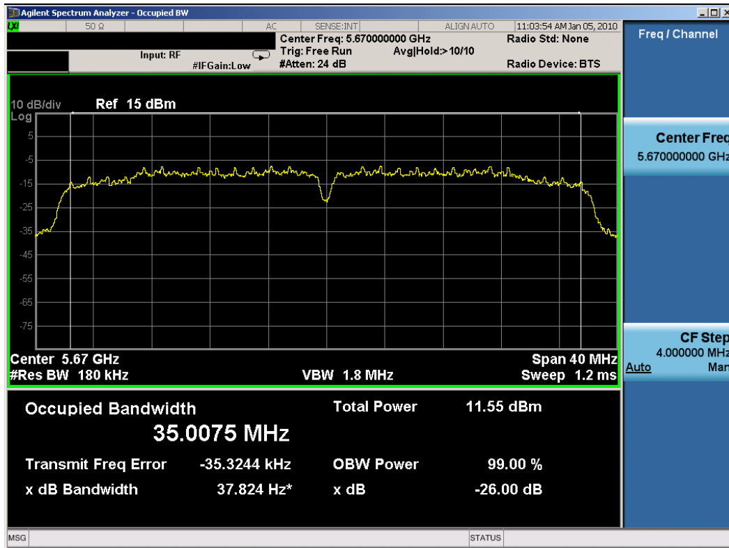
Plot 6-16. 26dB Bandwidth Plot (802.11n (UNII) – Ch. 134) - Chain A
