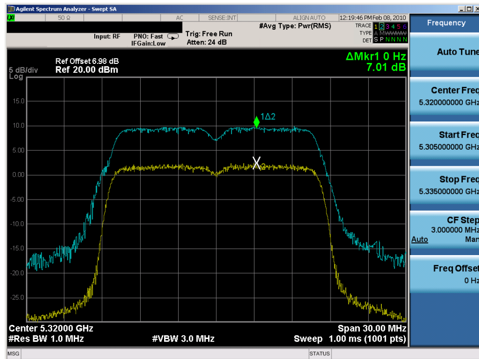
Plot 6-79. Peak Excursion Ratio Plot (802.11a (UNII) – Ch. 64) – Chain B
