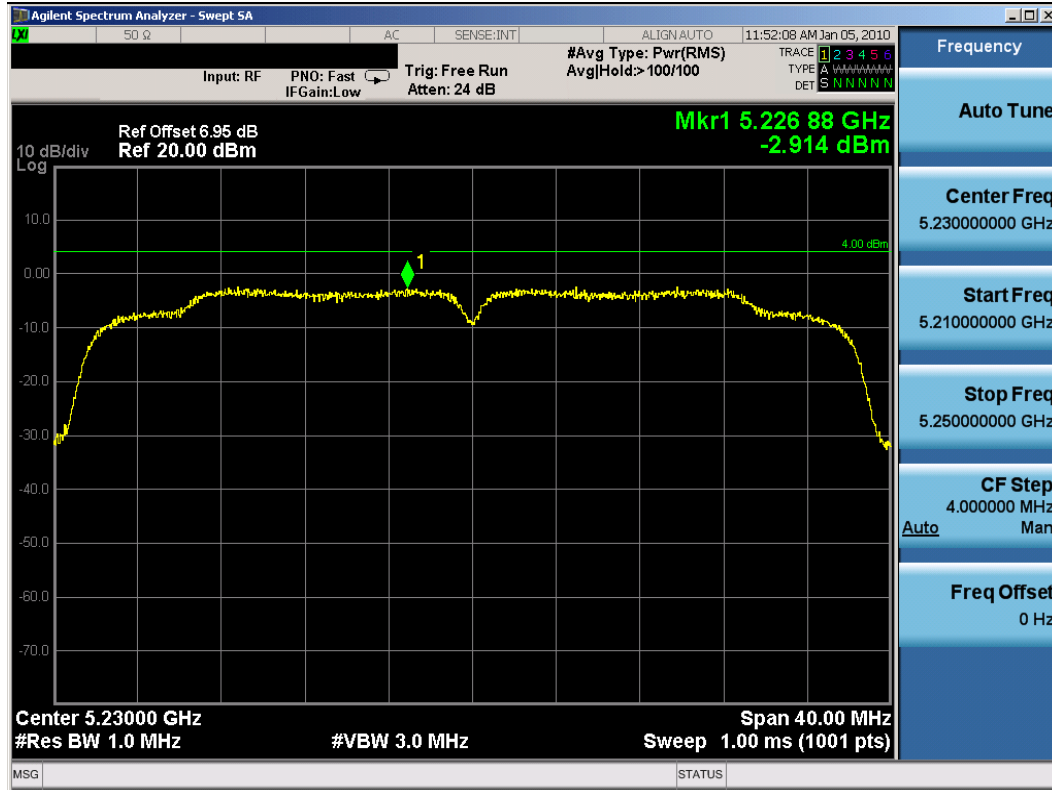
Plot 6-43. Peak Power Spectral Density Plot (802.11n (UNII) – Ch. 46) – Chain A
