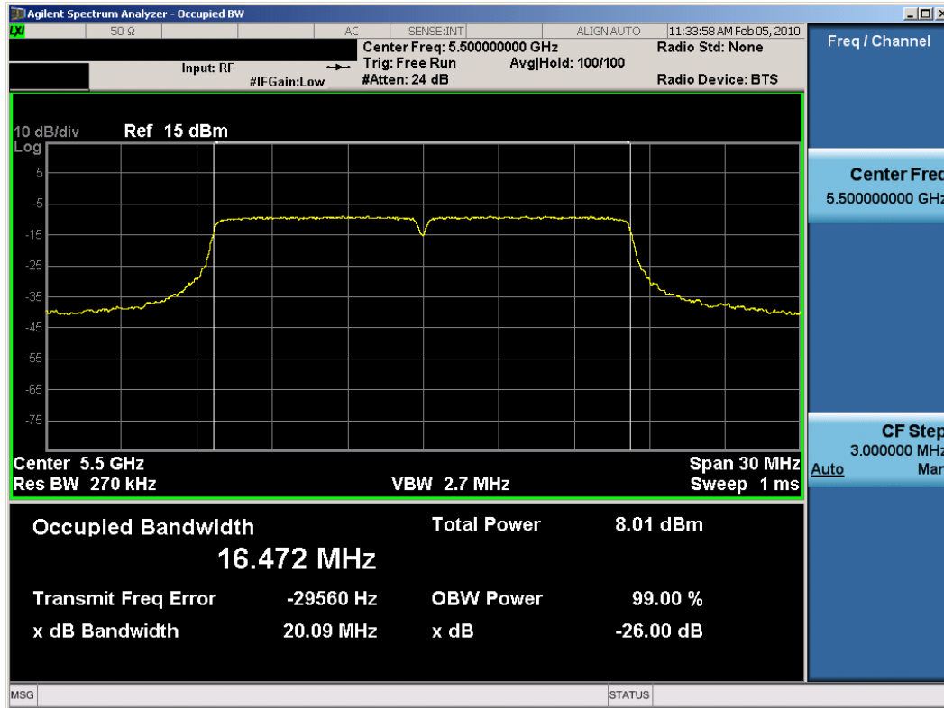
Plot 6-7. 26dB Bandwidth Plot (802.11a (UNII) – Ch. 100) – Chain A
