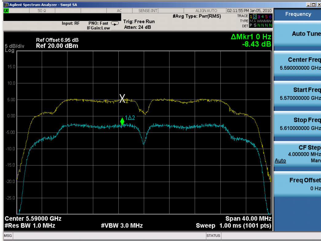
Plot 6-72. Peak Excursion Ratio Plot (802.11n (UNII) – Ch. 118) – Chain A
