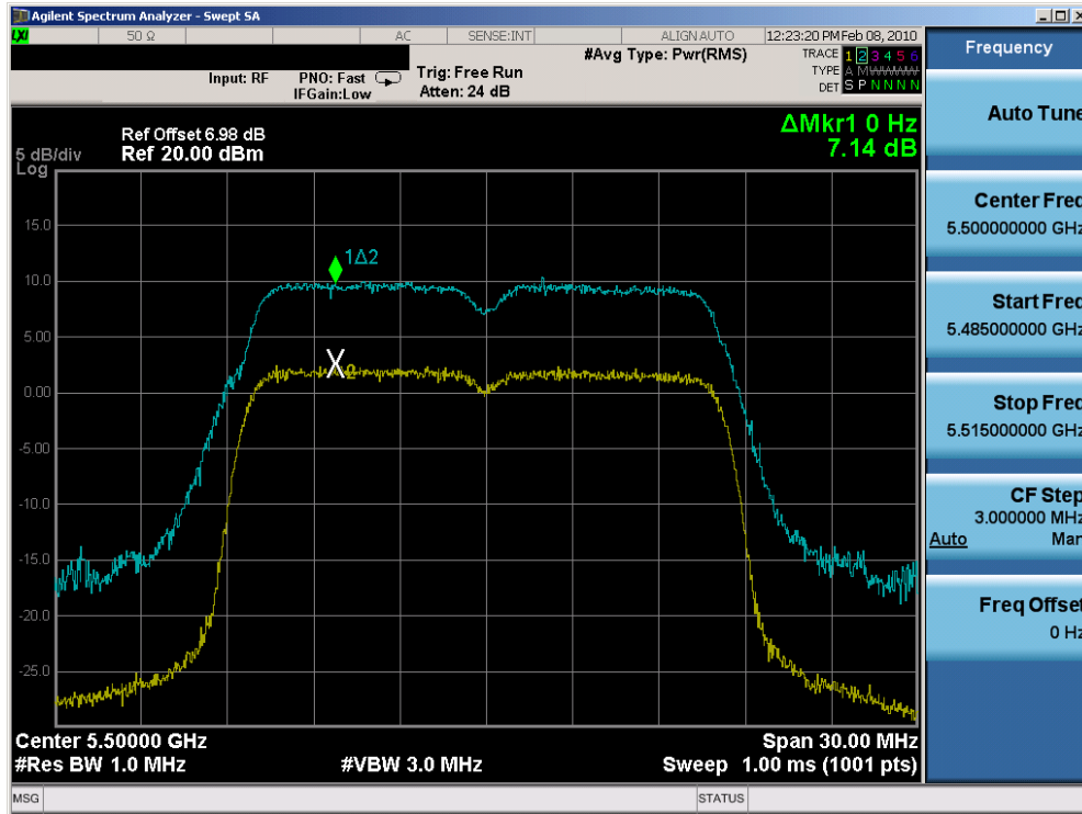
Plot 6-80. Peak Excursion Ratio Plot (802.11a (UNII) – Ch. 100) – Chain B
