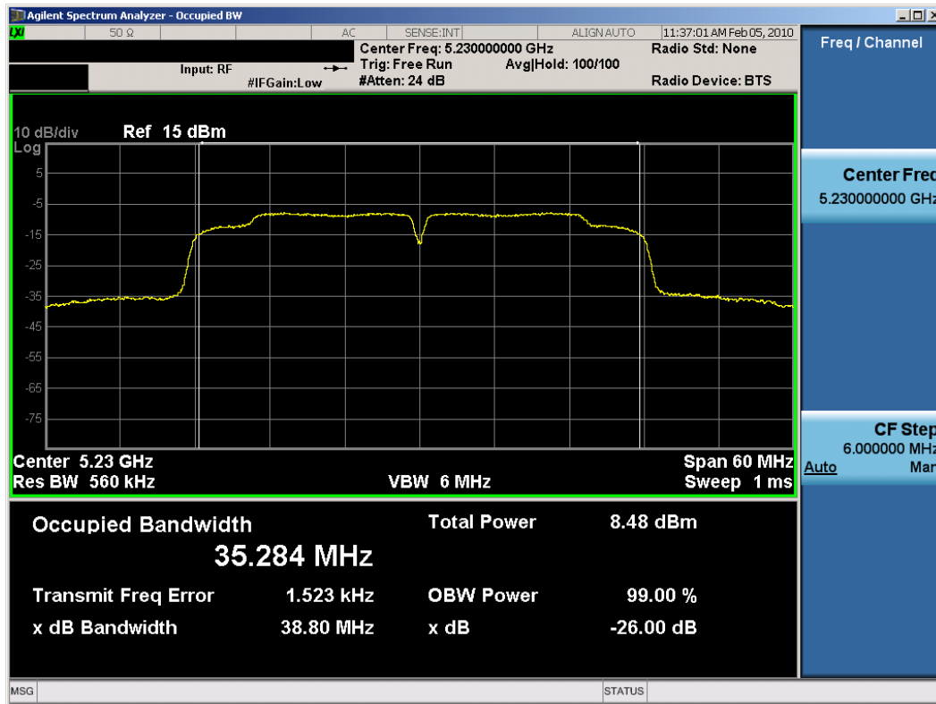
Plot 6-11. 26dB Bandwidth Plot (802.11n (UNII) – Ch. 46) – Chain A
