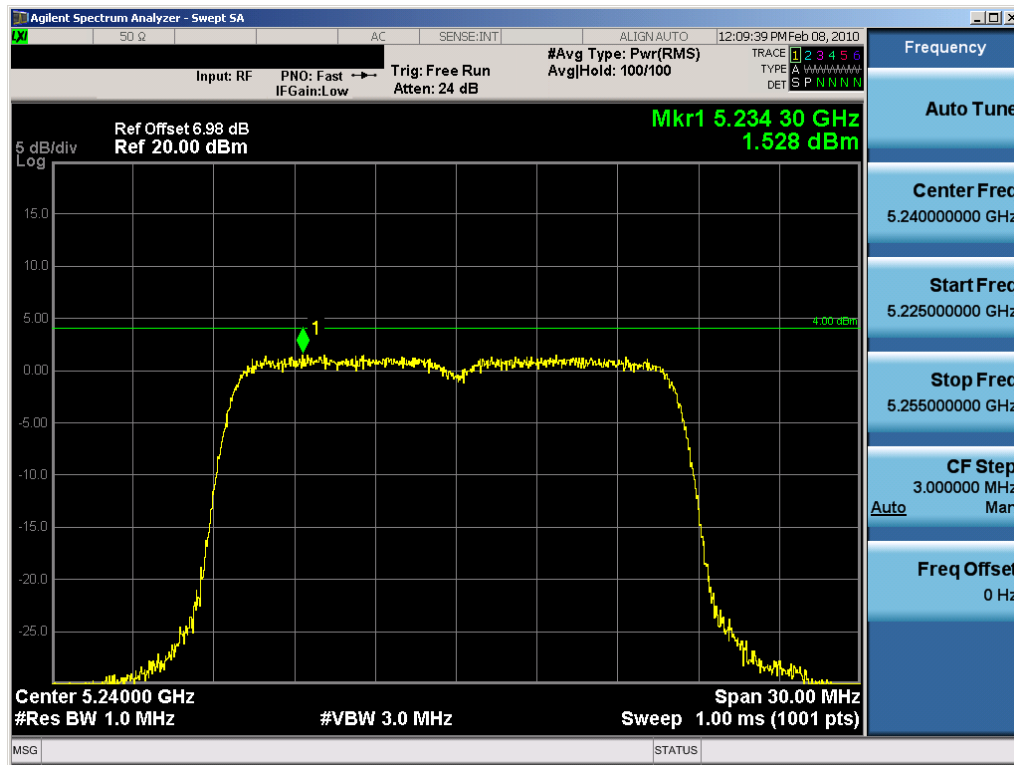
Plot 6-51. Peak Power Spectral Density Plot (802.11a (UNII) – Ch. 48) – Chain B
