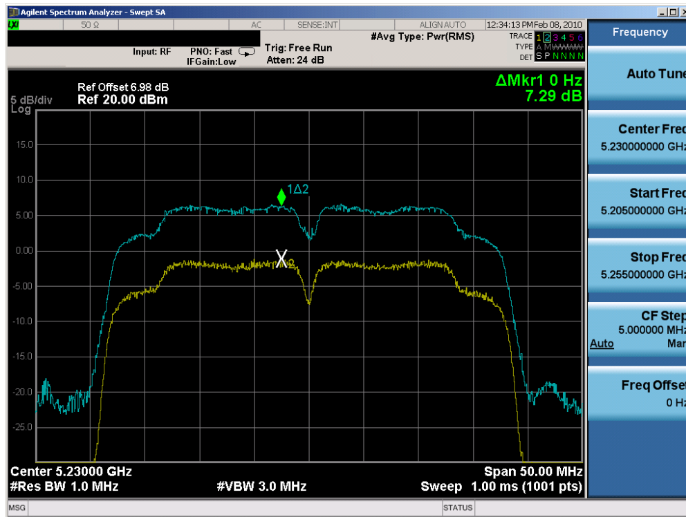
Plot 6-84. Peak Excursion Ratio Plot (802.11n (UNII) – Ch. 46) – Chain B
