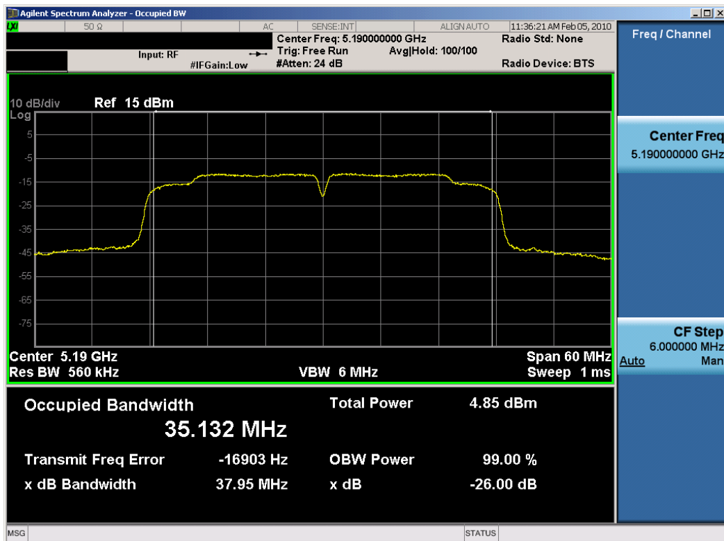
Plot 6-10. 26dB Bandwidth Plot (802.11n (UNII) – Ch. 38) – Chain A
