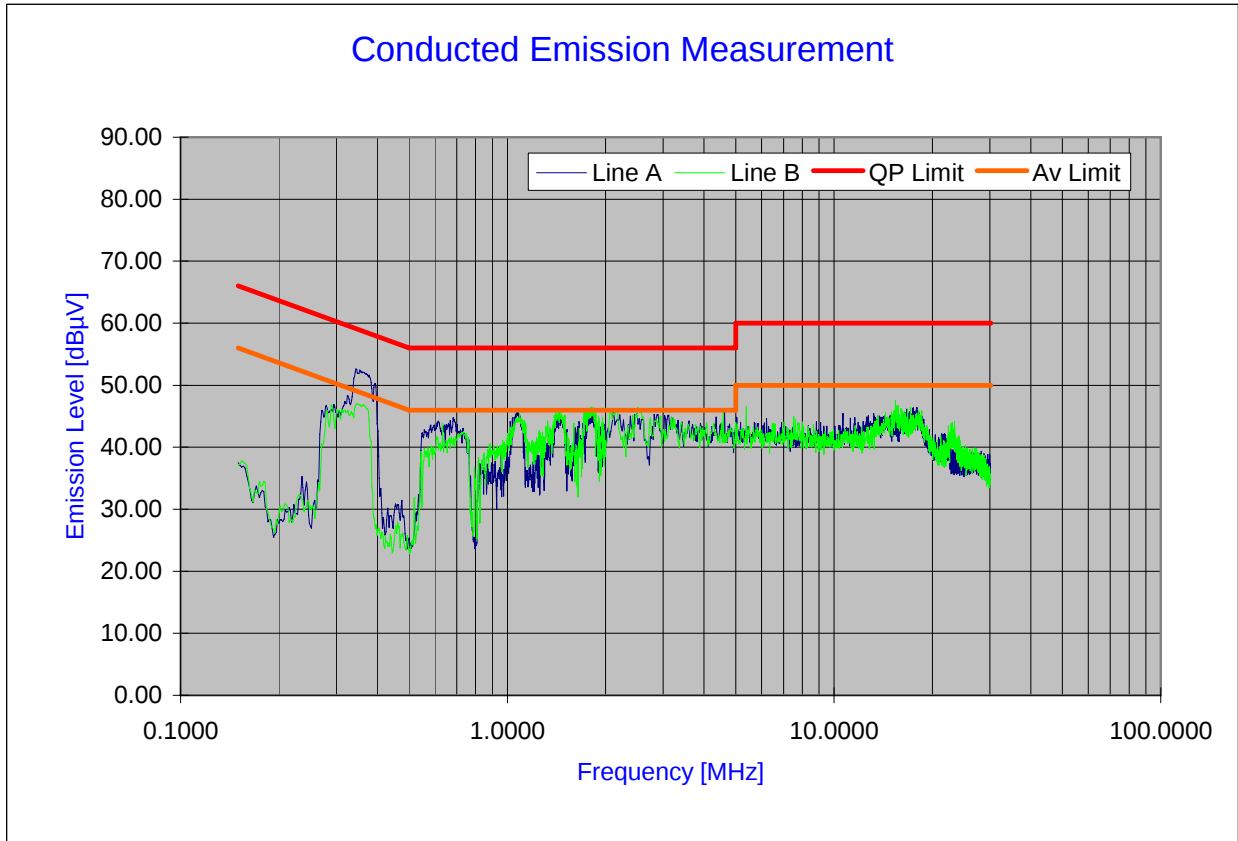
Plot 6-90. Line Conducted Plot with 802.11a (UNII Band I)
