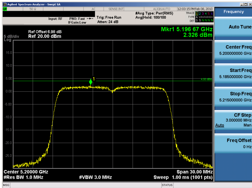
Plot 6-50. Peak Power Spectral Density Plot (802.11a (UNII) – Ch. 40) – Chain B
