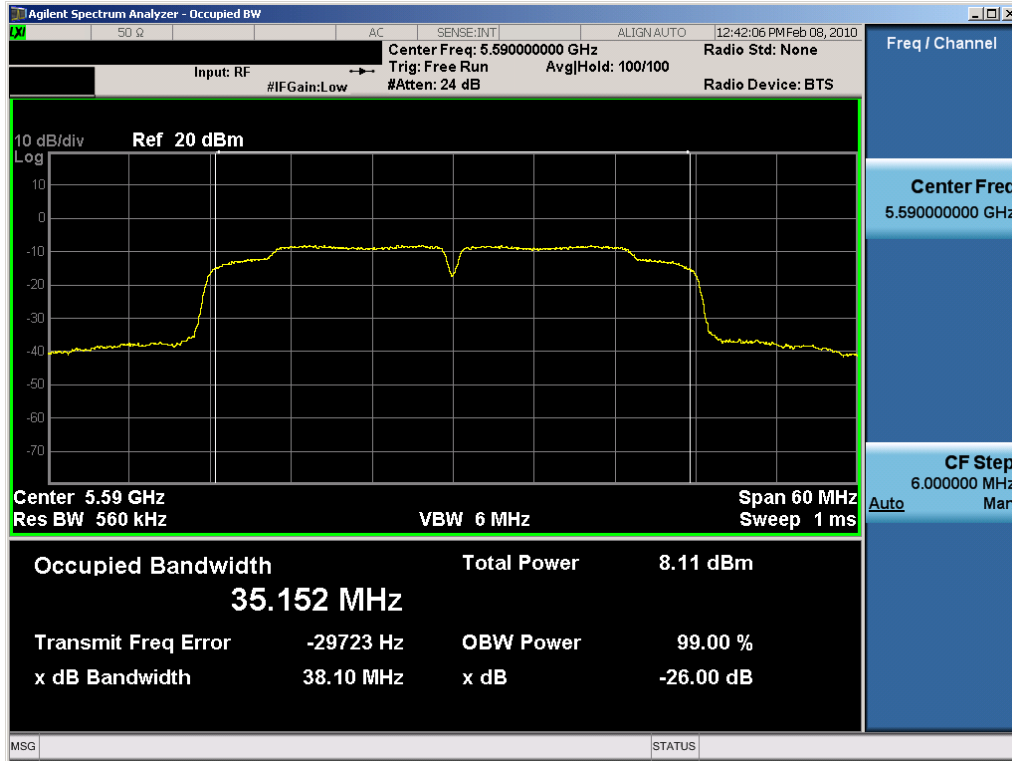
Plot 6-31. 26dB Bandwidth Plot (802.11n (UNII) – Ch. 118) – Chain B
