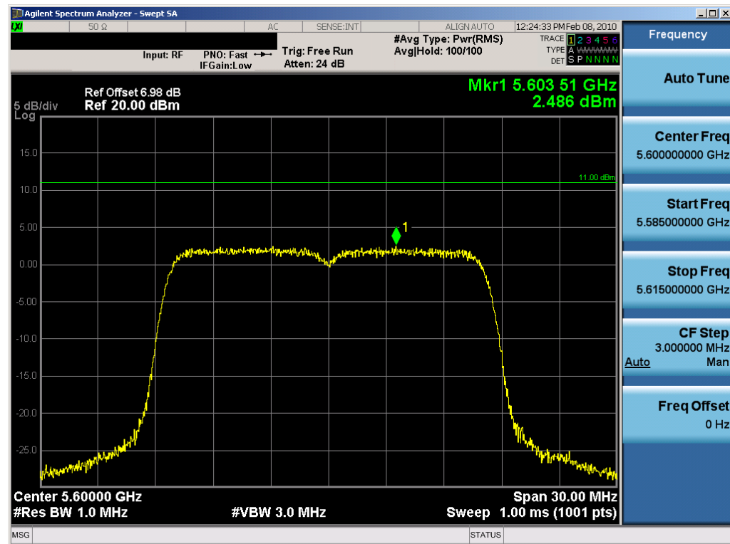
Plot 6-56. Peak Power Spectral Density Plot (802.11a (UNII) – Ch. 120) – Chain B
