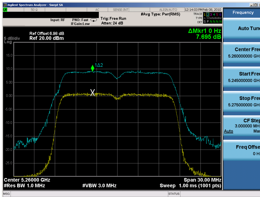
Plot 6-77. Peak Excursion Ratio Plot (802.11a (UNII) – Ch. 52) – Chain B
