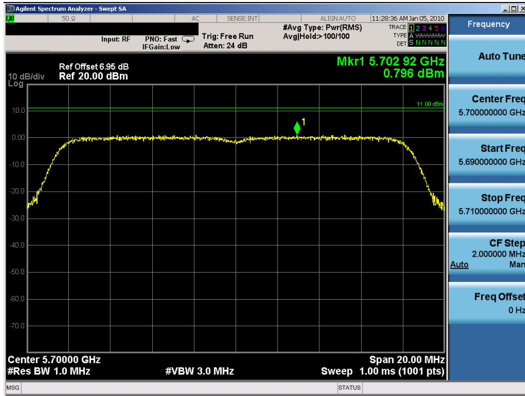
Plot 6-41. Peak Power Spectral Density Plot (802.11a (UNII) – Ch. 140) – Chain A
