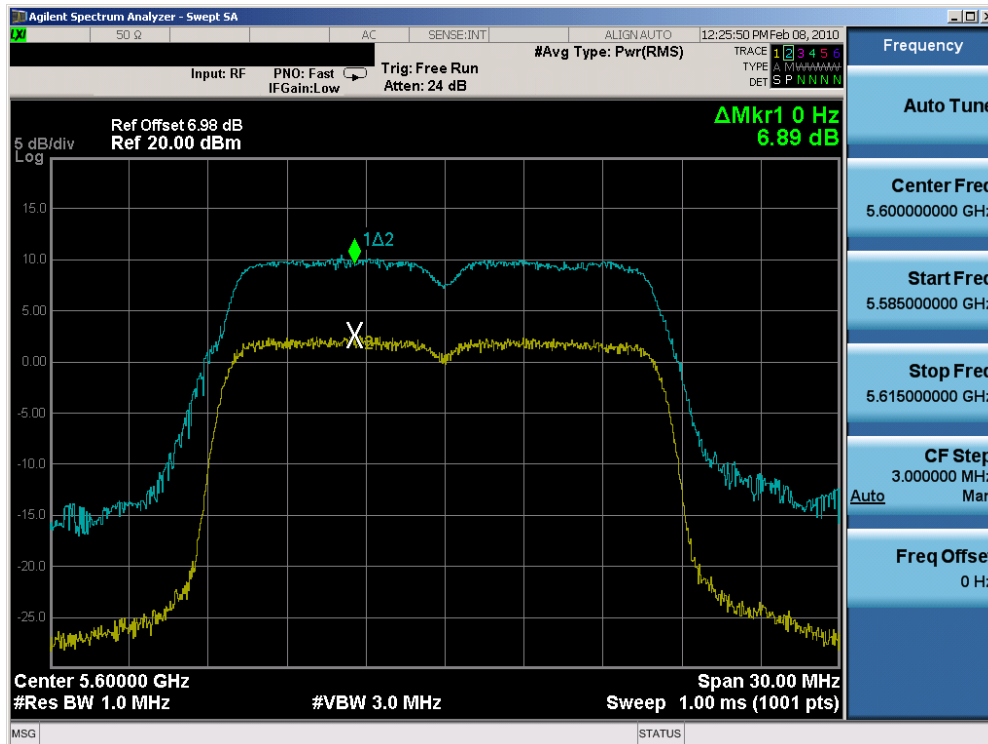
Plot 6-81. Peak Excursion Ratio Plot (802.11a (UNII) – Ch. 120) – Chain B
