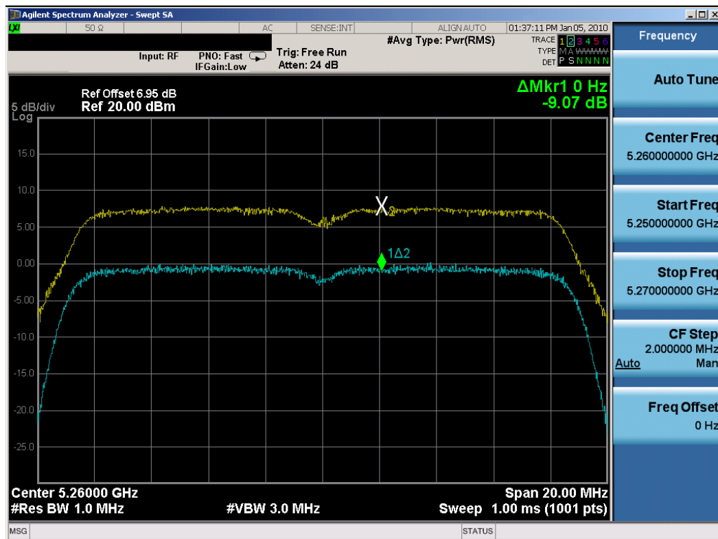
Plot 6-61. Peak Excursion Ratio Plot (802.11a (UNII) – Ch. 52) – Chain A
