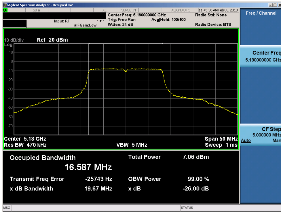
Plot 6-17. 26dB Bandwidth Plot (802.11a (UNII) – Ch. 36) – Chain B
