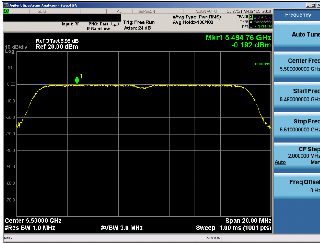
Plot 6-39. Peak Power Spectral Density Plot (802.11a (UNII) – Ch. 100) – Chain A
