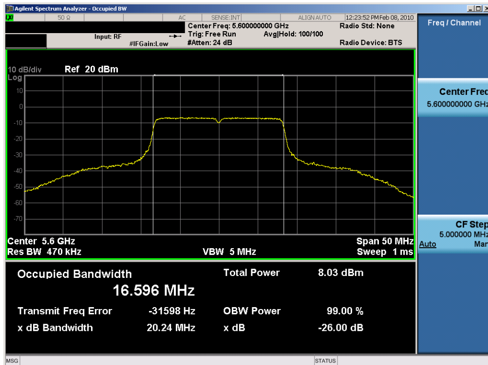
Plot 6-24. 26dB Bandwidth Plot (802.11a (UNII) – Ch. 120) – Chain B
