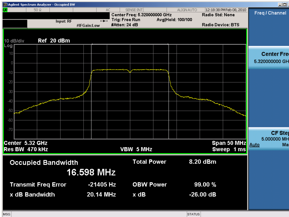
Plot 6-22. 26dB Bandwidth Plot (802.11a (UNII) – Ch. 64) – Chain B
