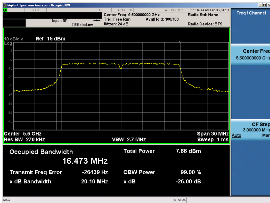
Plot 6-8. 26dB Bandwidth Plot (802.11a (UNII) – Ch. 120) – Chain A
