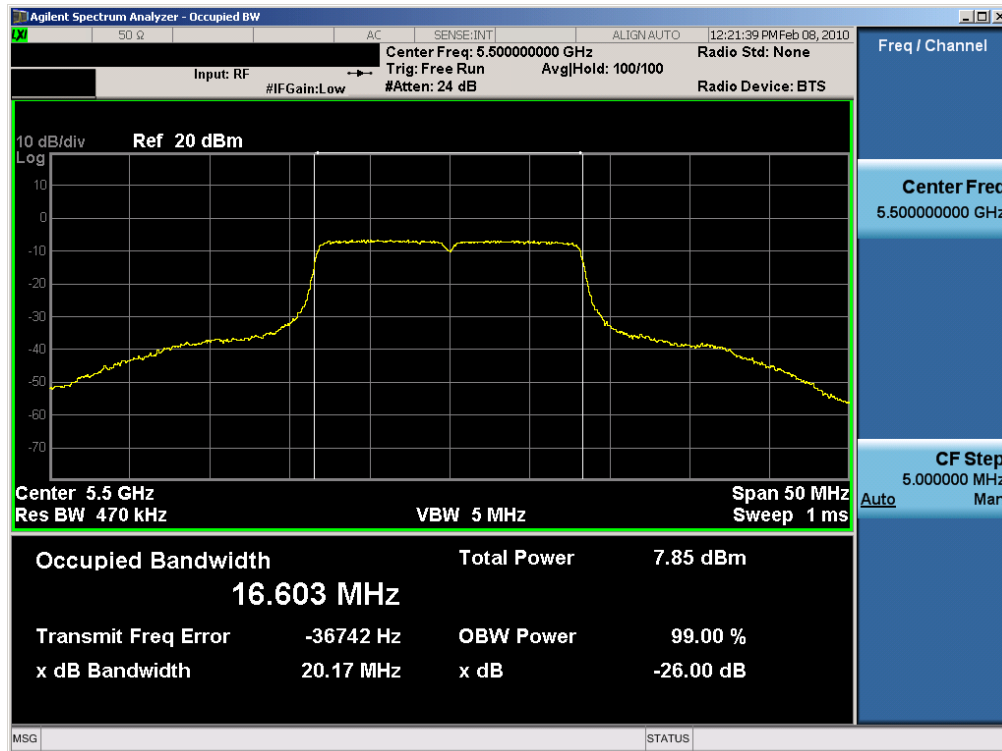
Plot 6-23. 26dB Bandwidth Plot (802.11a (UNII) – Ch. 100) – Chain B
