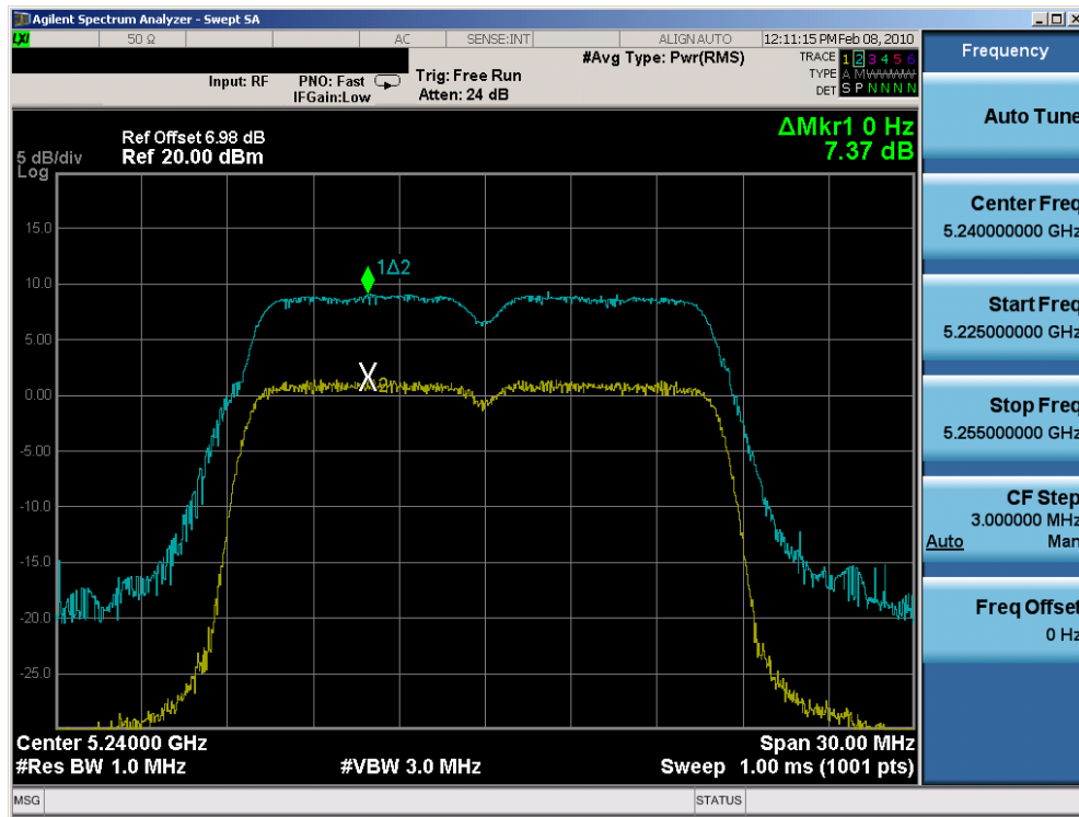
Plot 6-76. Peak Excursion Ratio Plot (802.11a (UNII) – Ch. 48) – Chain B
