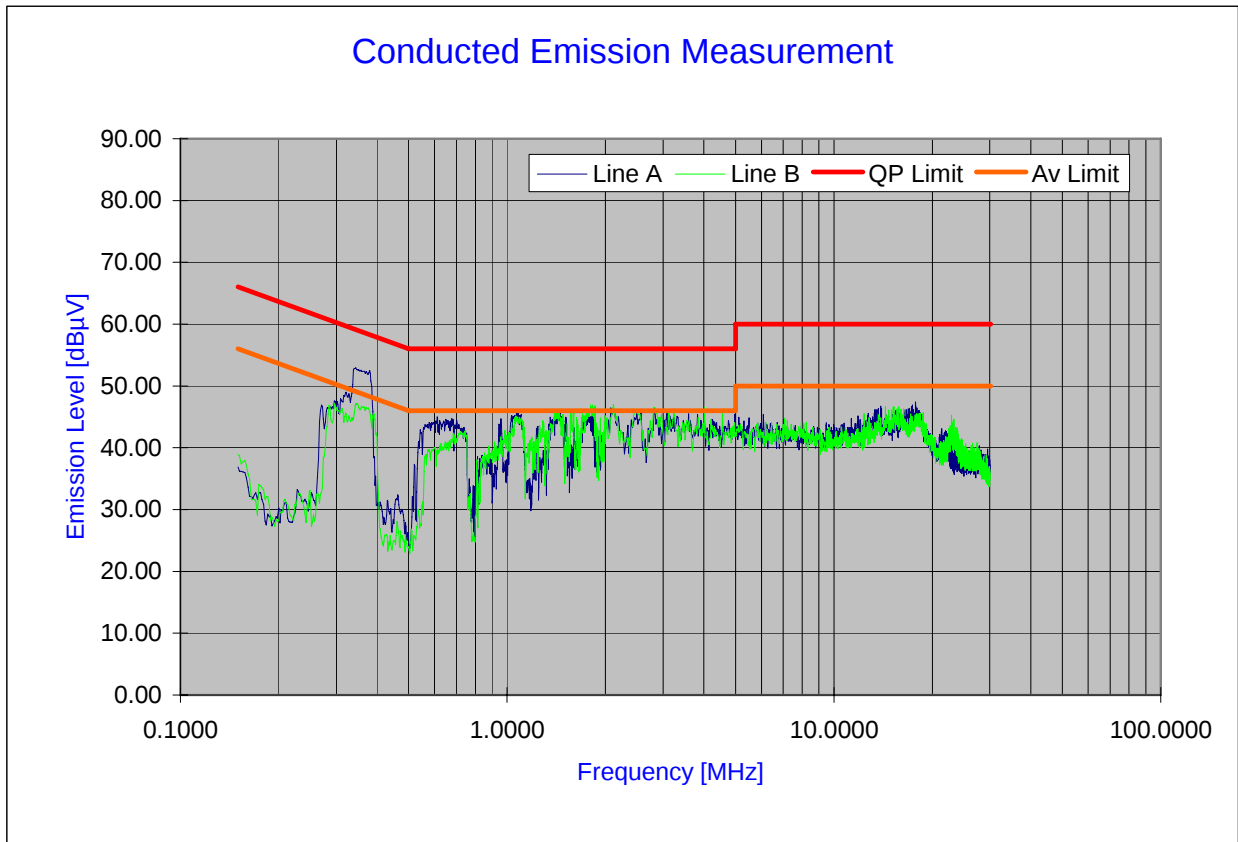
Plot 6-92. Line Conducted Plot with 802.11a (UNII Band III)
