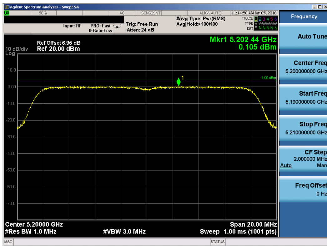
Plot 6-34. Peak Power Spectral Density Plot (802.11a (UNII) – Ch. 40) – Chain A
