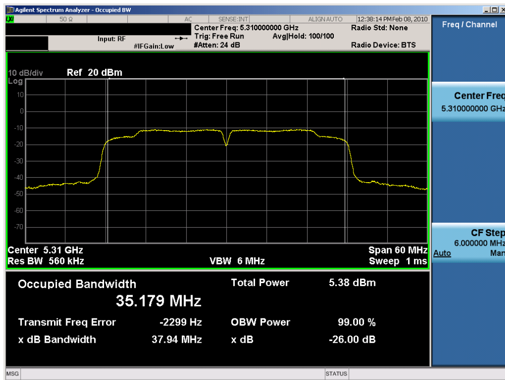
Plot 6-29. 26dB Bandwidth Plot (802.11n (UNII) – Ch. 62) – Chain B
