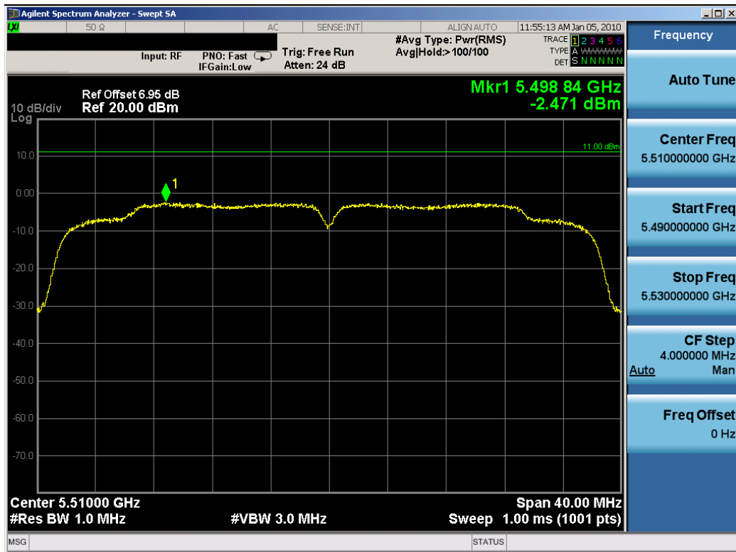
Plot 6-46. Peak Power Spectral Density Plot (802.11n (UNII) – Ch. 102) – Chain A
