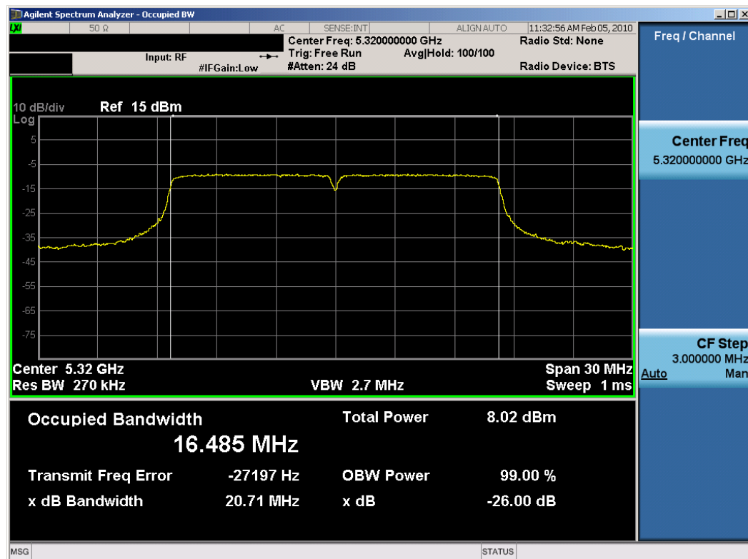
Plot 6-6. 26dB Bandwidth Plot (802.11a (UNII) – Ch. 64) – Chain A
