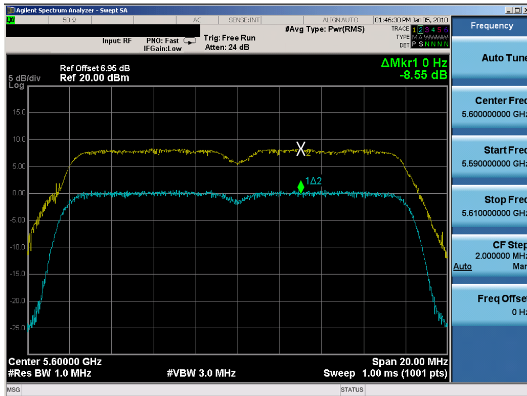
Plot 6-65. Peak Excursion Ratio Plot (802.11a (UNII) – Ch. 120) – Chain A
