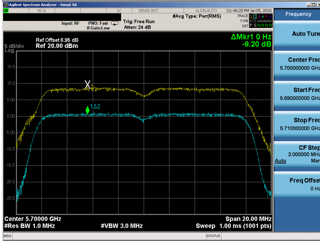
Plot 6-66. Peak Excursion Ratio Plot (802.11a (UNII) – Ch. 140) – Chain A
