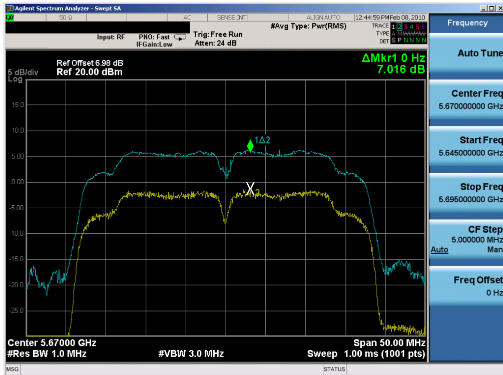
Plot 6-89. Peak Excursion Ratio Plot (802.11n (UNII) - Ch. 134) - Chain B
