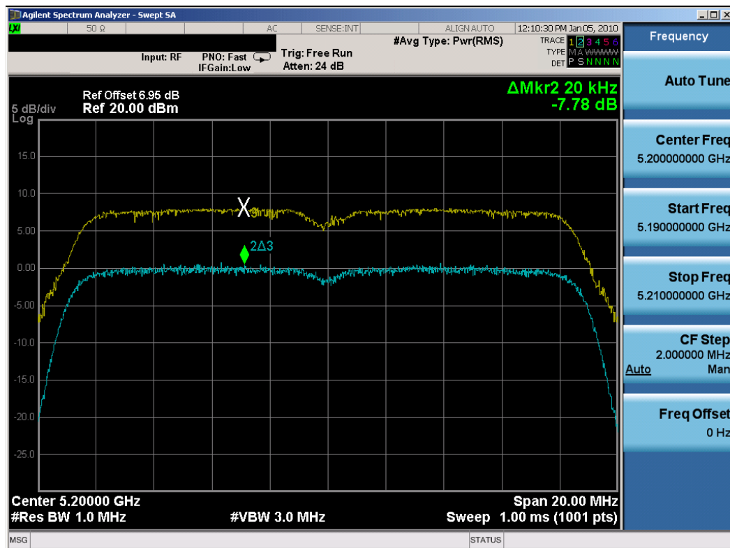
Plot 6-59. Peak Excursion Ratio Plot (802.11a (UNII) – Ch. 40) – Chain A
