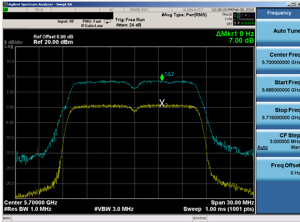
Plot 6-82. Peak Excursion Ratio Plot (802.11a (UNII) – Ch. 140) – Chain B
