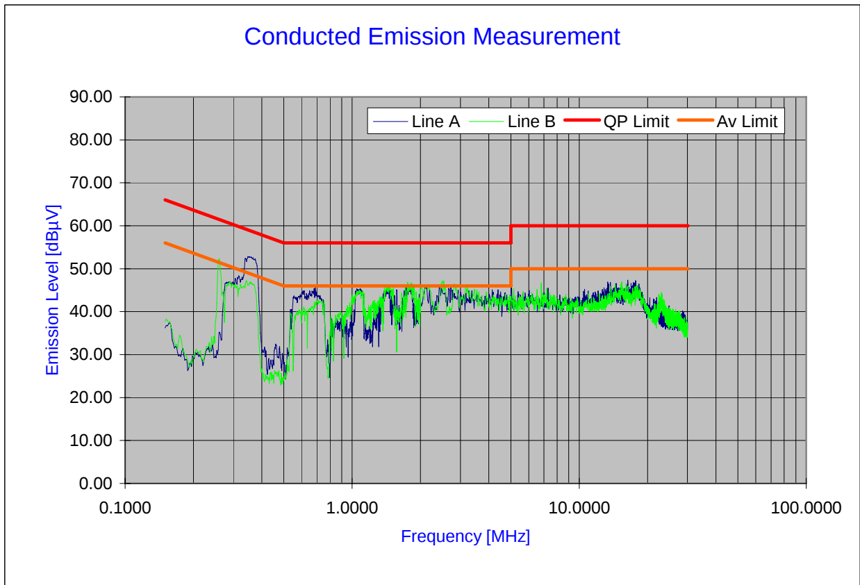
Plot 6-95. Line Conducted Plot with 802.11n (UNII Band III)
