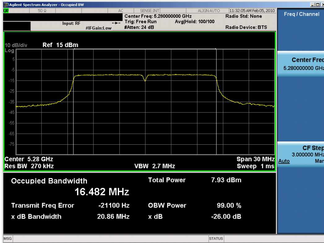
Plot 6-5. 26dB Bandwidth Plot (802.11a (UNII) – Ch. 56) – Chain A
