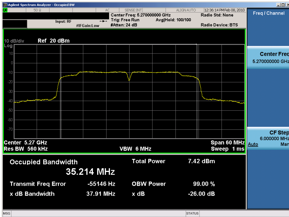
Plot 6-28. 26dB Bandwidth Plot (802.11n (UNII) – Ch. 54) – Chain B
