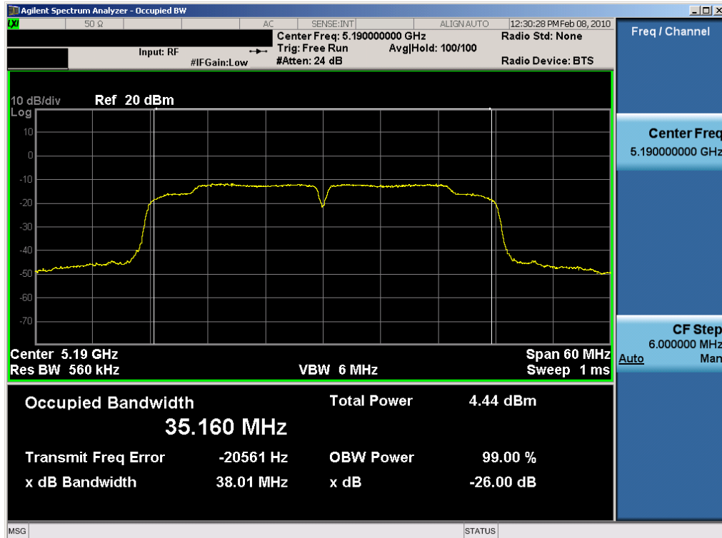
Plot 6-26. 26dB Bandwidth Plot (802.11n (UNII) – Ch. 38) – Chain B
