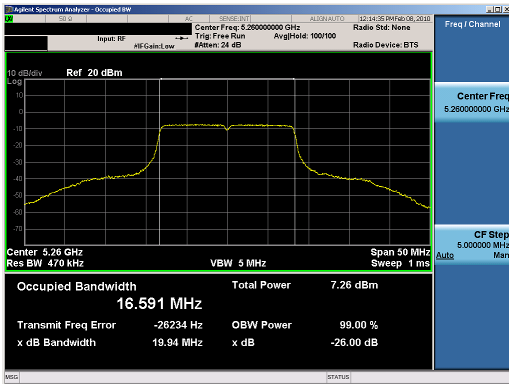
Plot 6-20. 26dB Bandwidth Plot (802.11a (UNII) – Ch. 52) – Chain B
