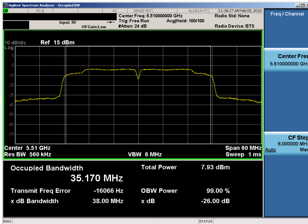
Plot 6-14. 26dB Bandwidth Plot (802.11n (UNII) – Ch. 102) – Chain A
