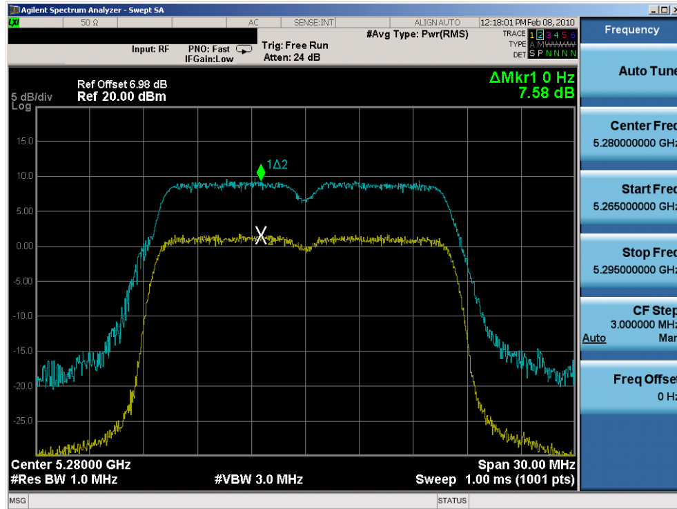
Plot 6-78. Peak Excursion Ratio Plot (802.11a (UNII) – Ch. 56) – Chain B
