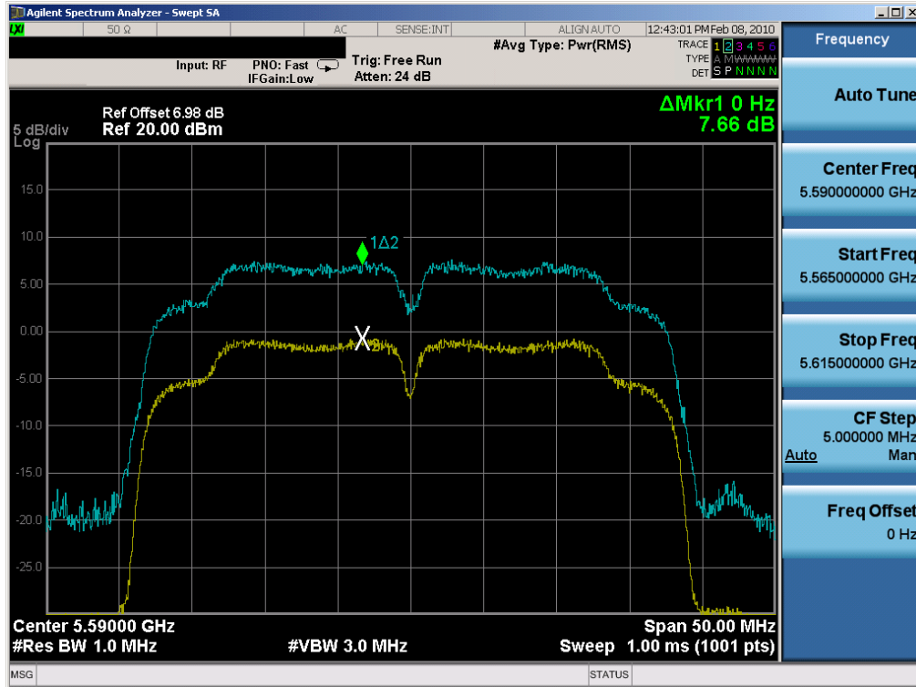
Plot 6-88. Peak Excursion Ratio Plot (802.11n (UNII) - Ch. 118) - Chain B
