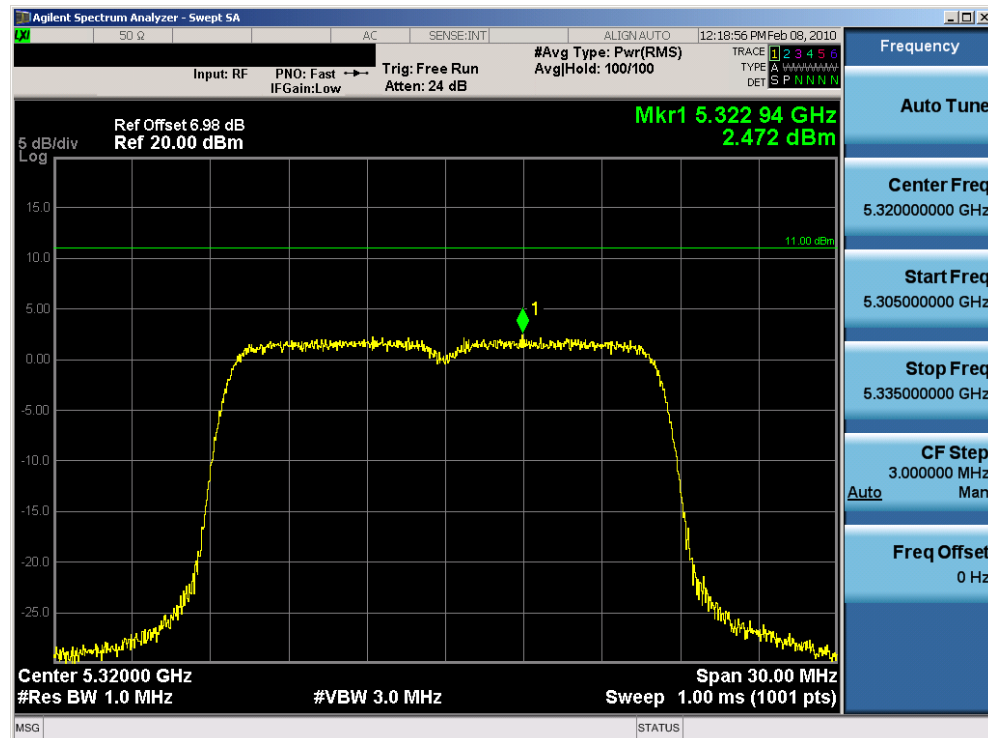
Plot 6-54. Peak Power Spectral Density Plot (802.11a (UNII) – Ch. 64) – Chain B
