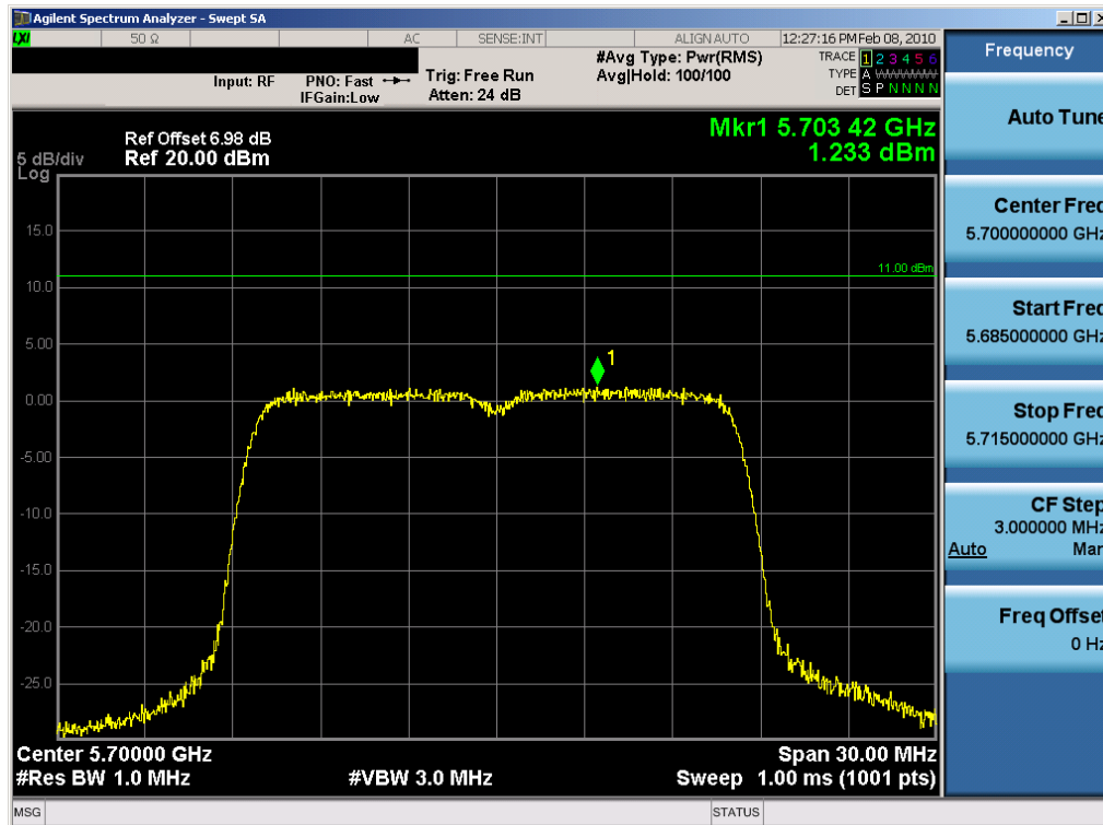
Plot 6-57. Peak Power Spectral Density Plot (802.11a (UNII) – Ch. 140) – Chain B
