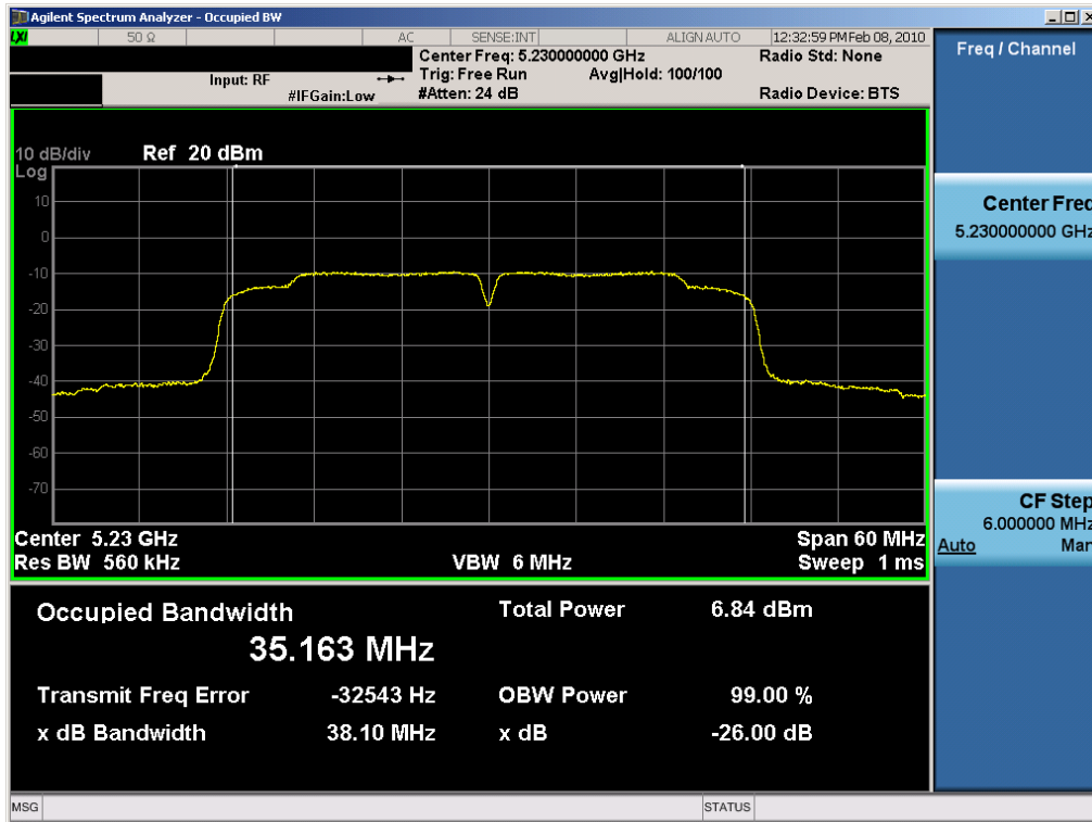
Plot 6-27. 26dB Bandwidth Plot (802.11n (UNII) – Ch. 46) – Chain B
