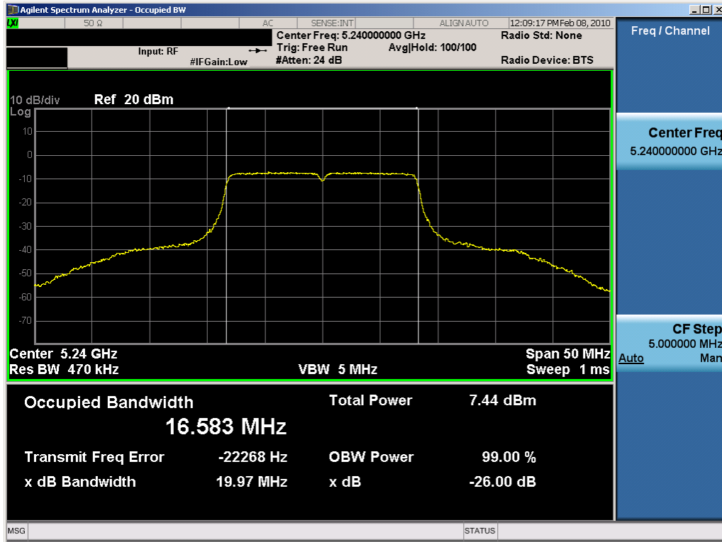
Plot 6-19. 26dB Bandwidth Plot (802.11a (UNII) – Ch. 48) – Chain B
