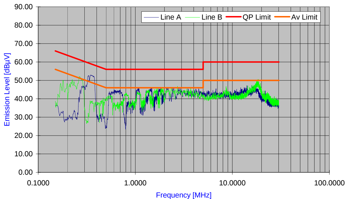
Plot 6-93. Line Conducted Plot with 802.11n (UNII Band I)
