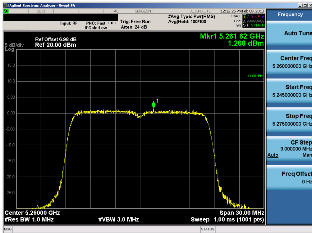
Plot 6-52. Peak Power Spectral Density Plot (802.11a (UNII) – Ch. 52) – Chain B
