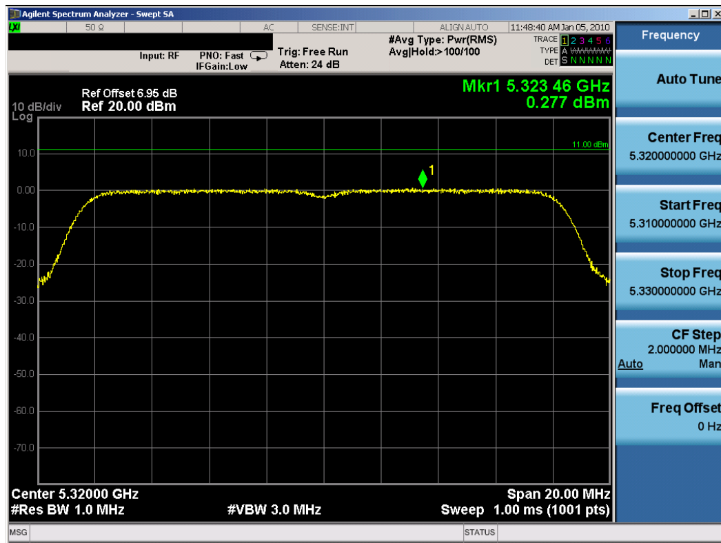
Plot 6-38. Peak Power Spectral Density Plot (802.11a (UNII) – Ch. 64) – Chain A
