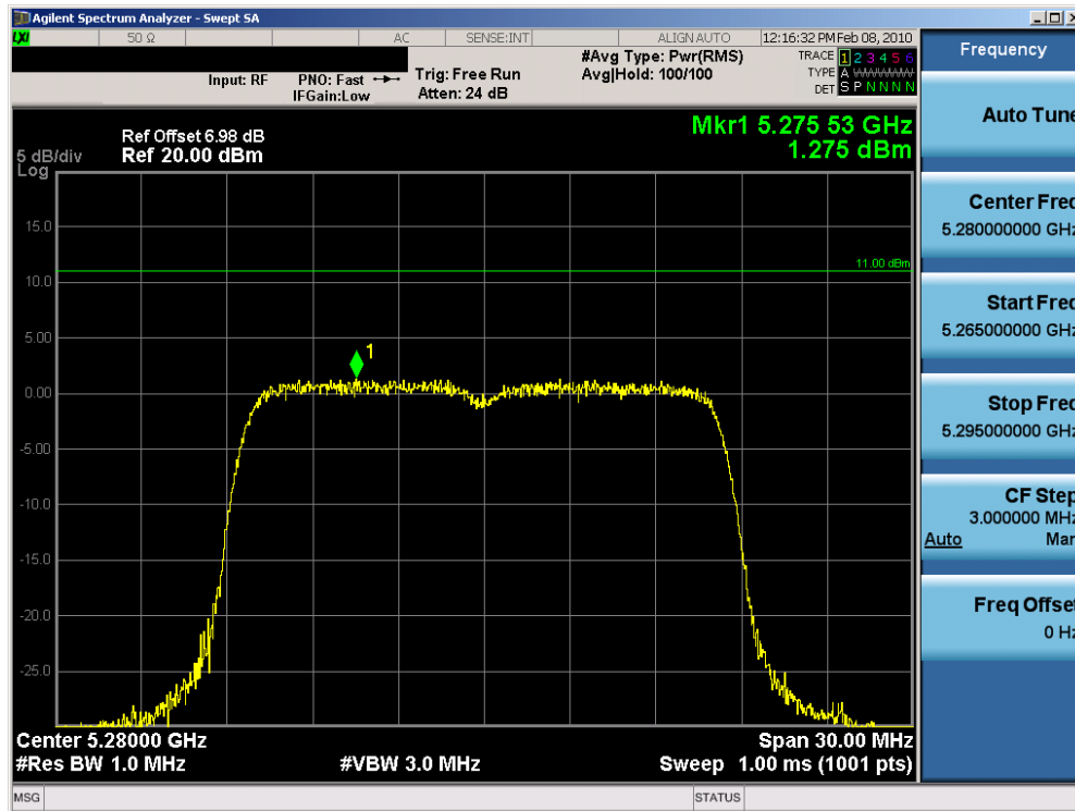
Plot 6-53. Peak Power Spectral Density Plot (802.11a (UNII) – Ch. 56) – Chain B
