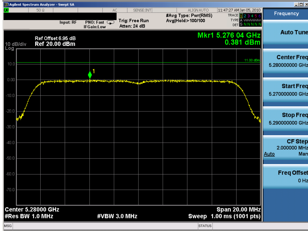
Plot 6-37. Peak Power Spectral Density Plot (802.11a (UNII) – Ch. 56) – Chain A
