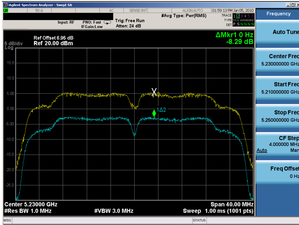
Plot 6-68. Peak Excursion Ratio Plot (802.11n (UNII) – Ch. 46) – Chain A
