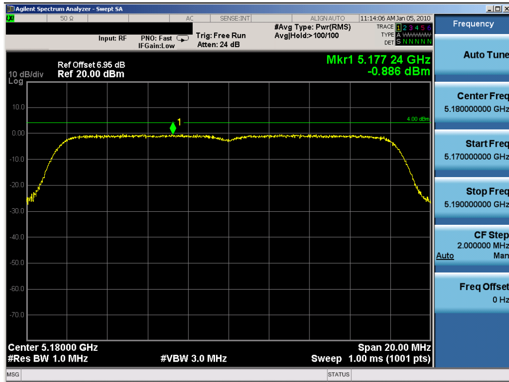
Plot 6-33. Peak Power Spectral Density Plot (802.11a (UNII) – Ch. 36) – Chain A
