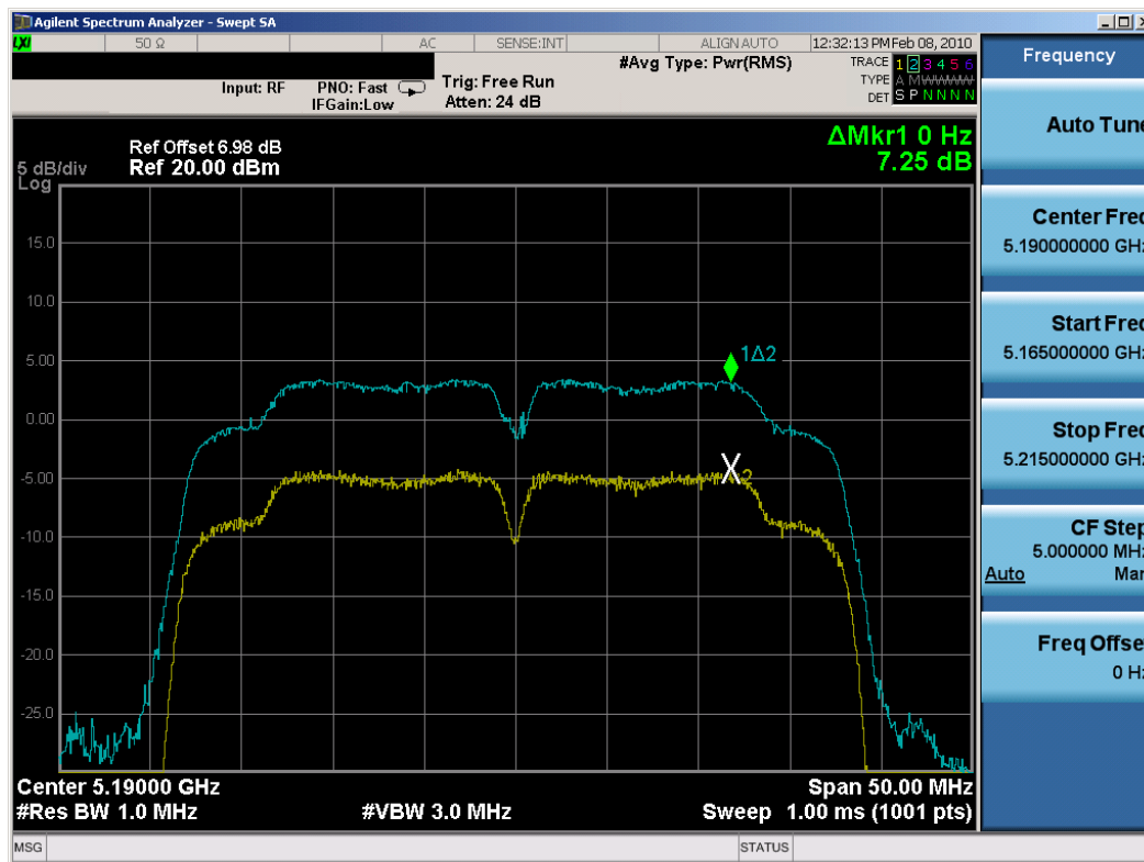
Plot 6-83. Peak Excursion Ratio Plot (802.11n (UNII) – Ch. 38) – Chain B
