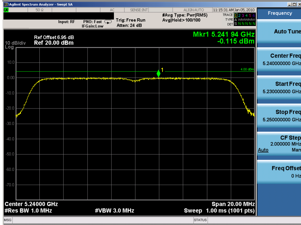
Plot 6-35. Peak Power Spectral Density Plot (802.11a (UNII) – Ch. 48) – Chain A
