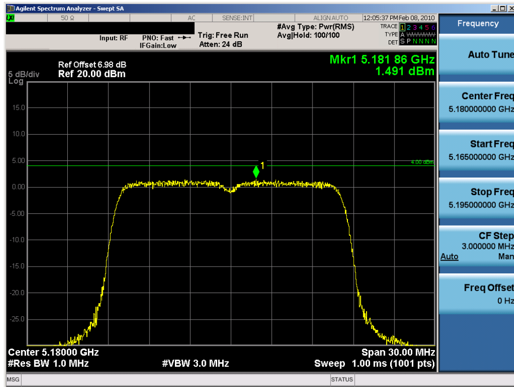
Plot 6-49. Peak Power Spectral Density Plot (802.11a (UNII) – Ch. 36) – Chain B
