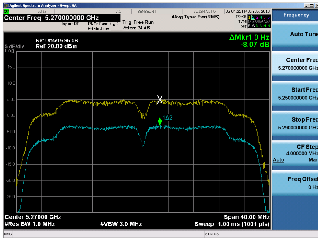
Plot 6-69. Peak Excursion Ratio Plot (802.11n (UNII) – Ch. 54) – Chain A
