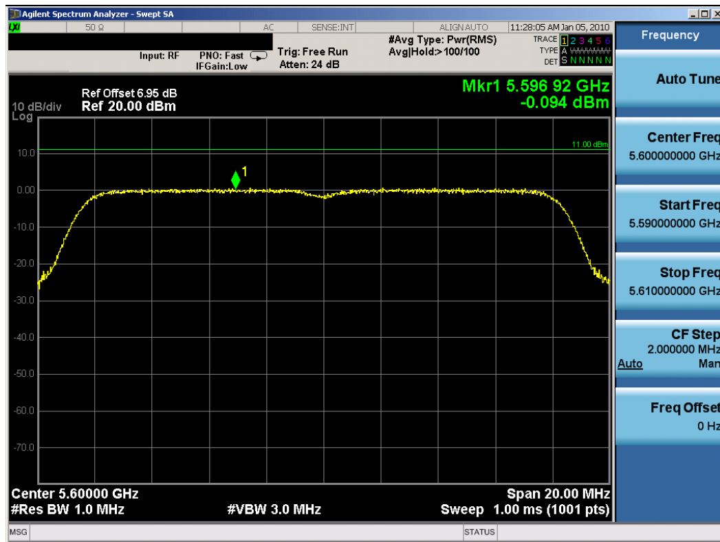
Plot 6-40. Peak Power Spectral Density Plot (802.11a (UNII) – Ch. 120) – Chain A
