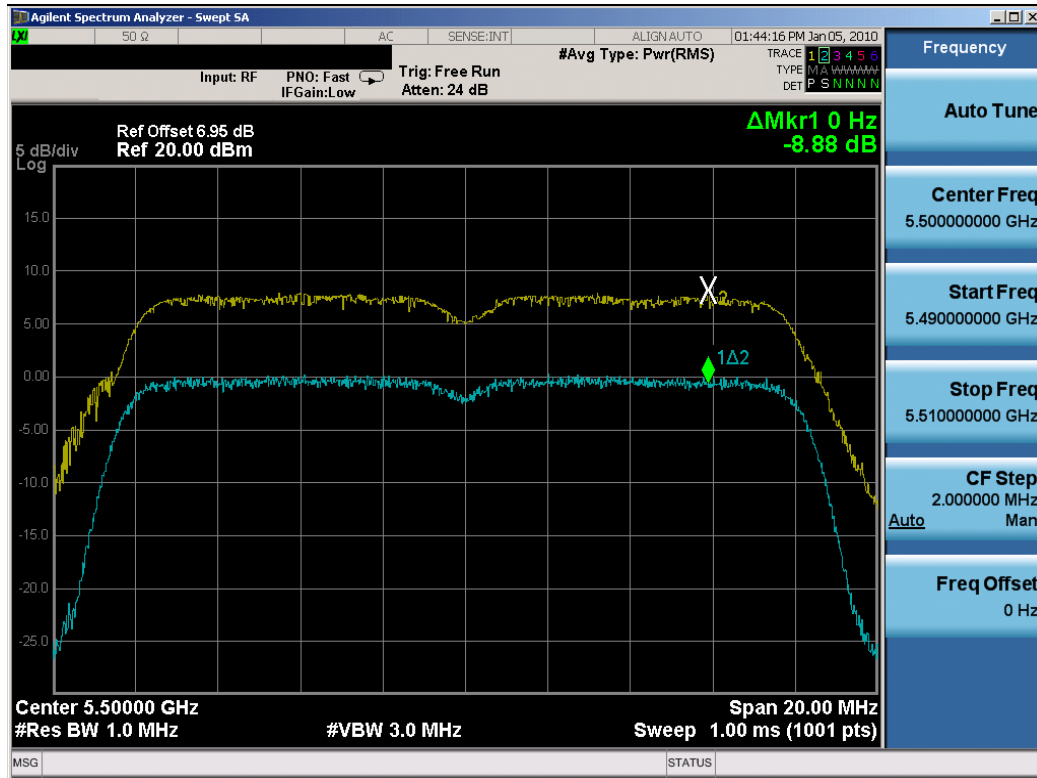
Plot 6-64. Peak Excursion Ratio Plot (802.11a (UNII) – Ch. 100) – Chain A
