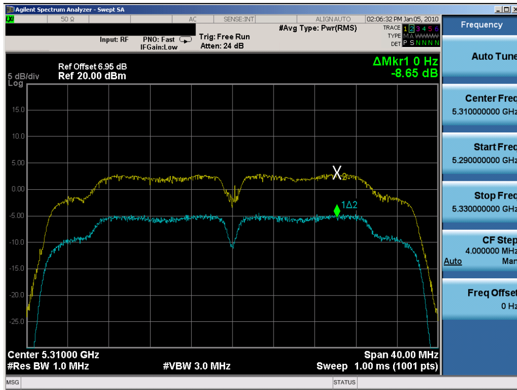
Plot 6-70. Peak Excursion Ratio Plot (802.11n (UNII) - Ch. 62) - Chain A
