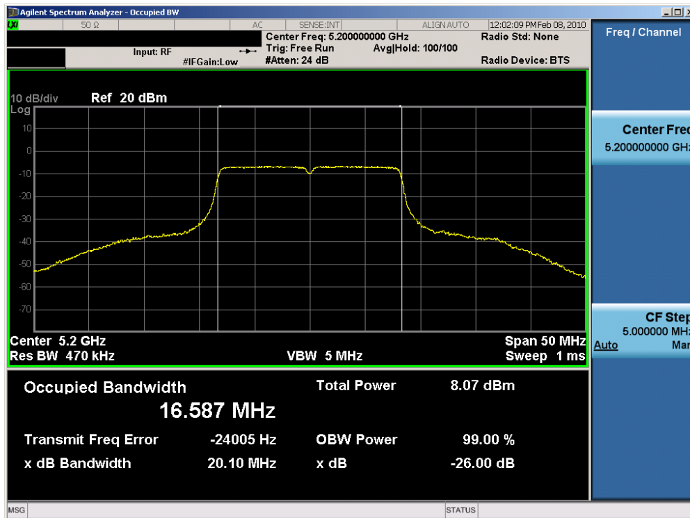
Plot 6-18. 26dB Bandwidth Plot (802.11a (UNII) – Ch. 40) – Chain B
