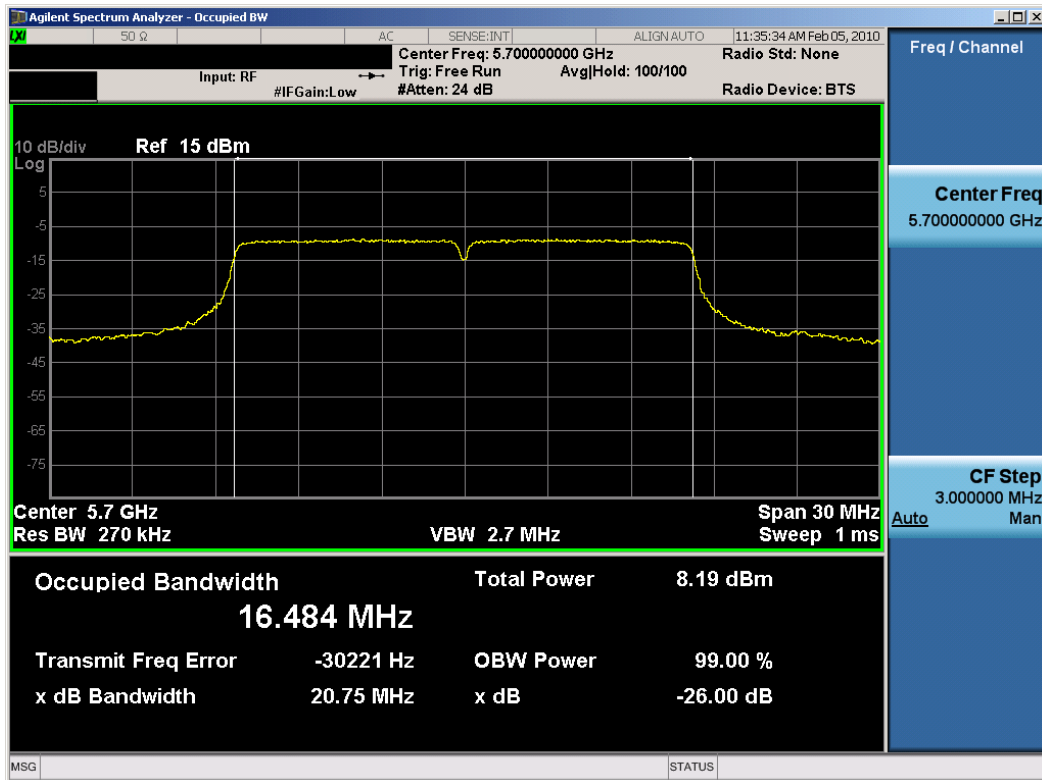
Plot 6-9. 26dB Bandwidth Plot (802.11a (UNII) – Ch. 140) – Chain A
