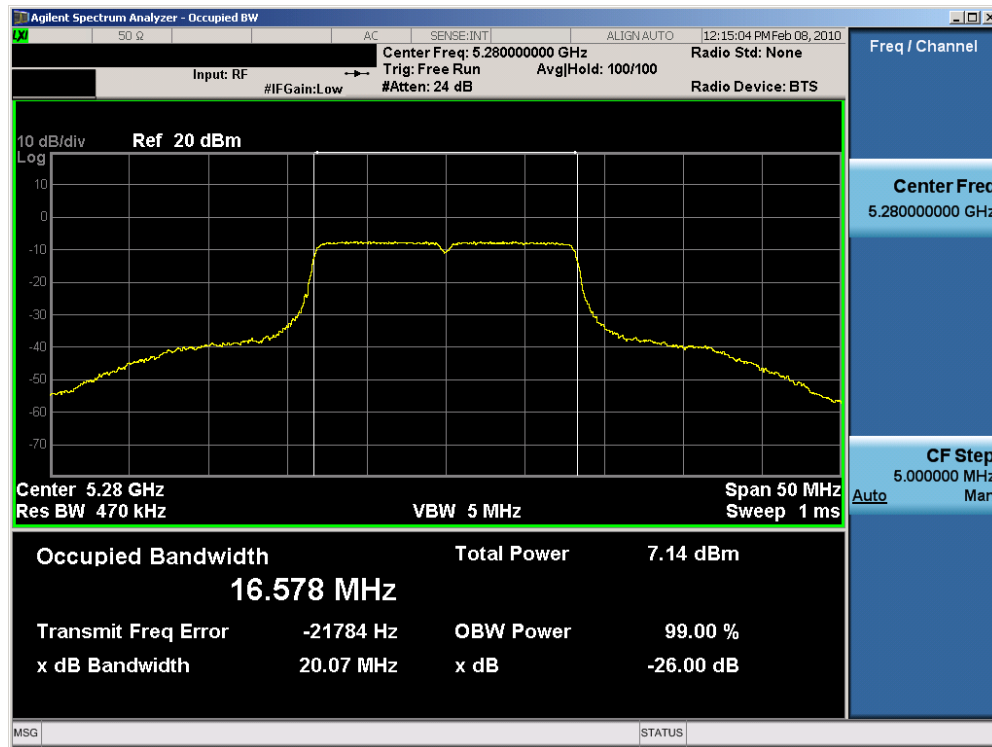
Plot 6-21. 26dB Bandwidth Plot (802.11a (UNII) – Ch. 56) – Chain B
