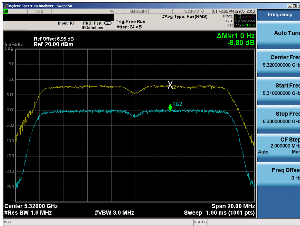
Plot 6-63. Peak Excursion Ratio Plot (802.11a (UNII) – Ch. 64) – Chain A
