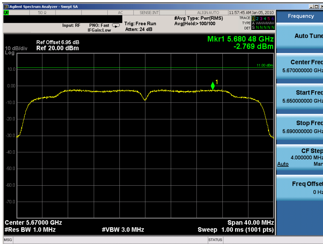
Plot 6-48. Peak Power Spectral Density Plot (802.11n (UNII) – Ch. 134) - Chain A
