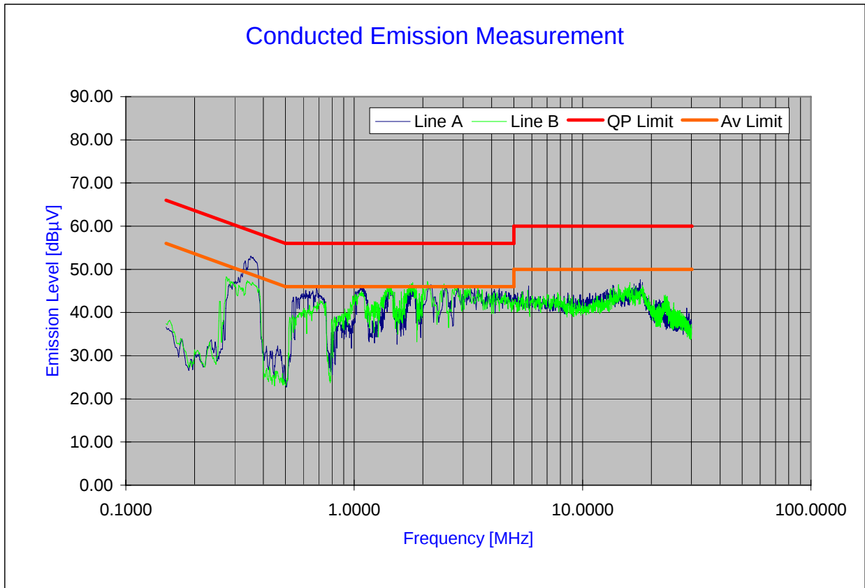
Plot 6-94. Line Conducted Plot with 802.11n (UNII Band II)
