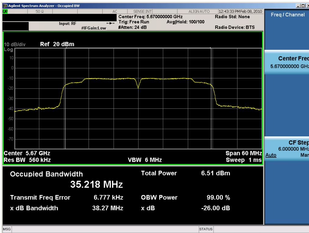
Plot 6-32. 26dB Bandwidth Plot (802.11n (UNII) – Ch. 134) - Chain B
