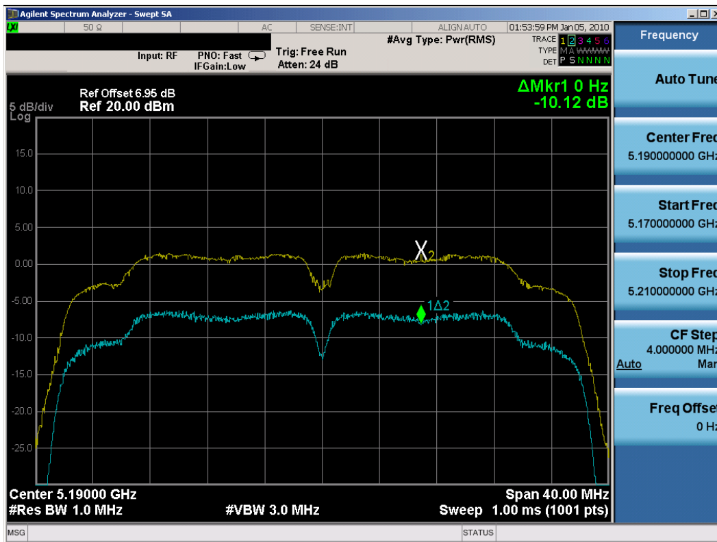
Plot 6-67. Peak Excursion Ratio Plot (802.11n (UNII) – Ch. 38) – Chain A
