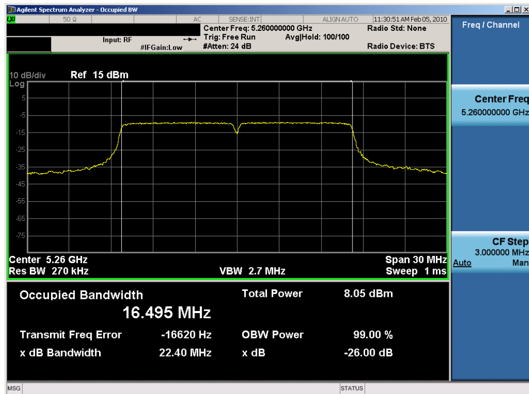
Plot 6-4. 26dB Bandwidth Plot (802.11a (UNII) – Ch. 52) – Chain A
