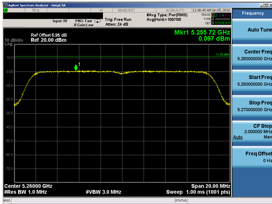
Plot 6-36. Peak Power Spectral Density Plot (802.11a (UNII) – Ch. 52) – Chain A
