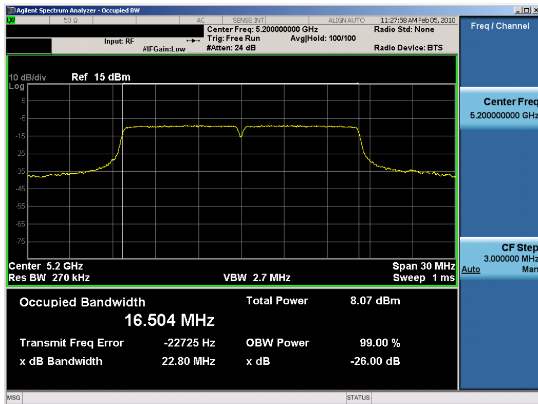
Plot 6-2. 26dB Bandwidth Plot (802.11a (UNII) – Ch. 40) – Chain A
