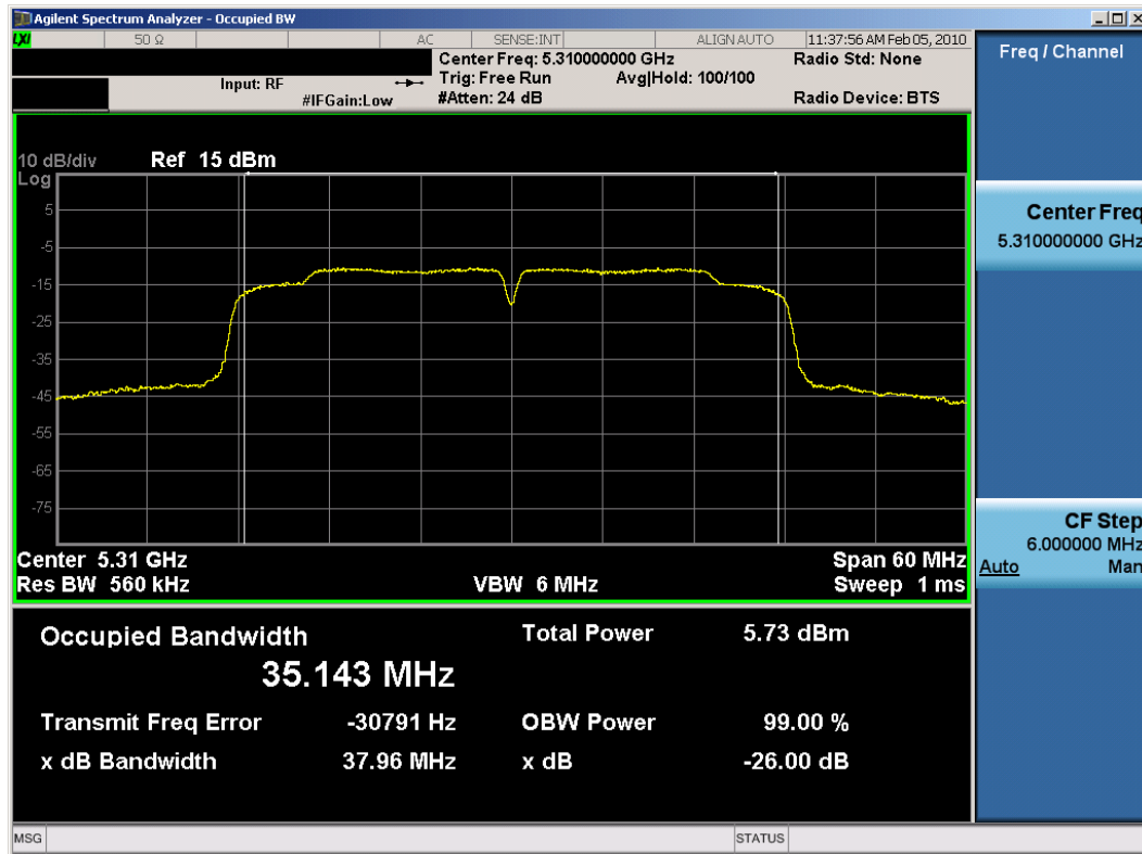
Plot 6-13. 26dB Bandwidth Plot (802.11n (UNII) – Ch. 62) – Chain A
