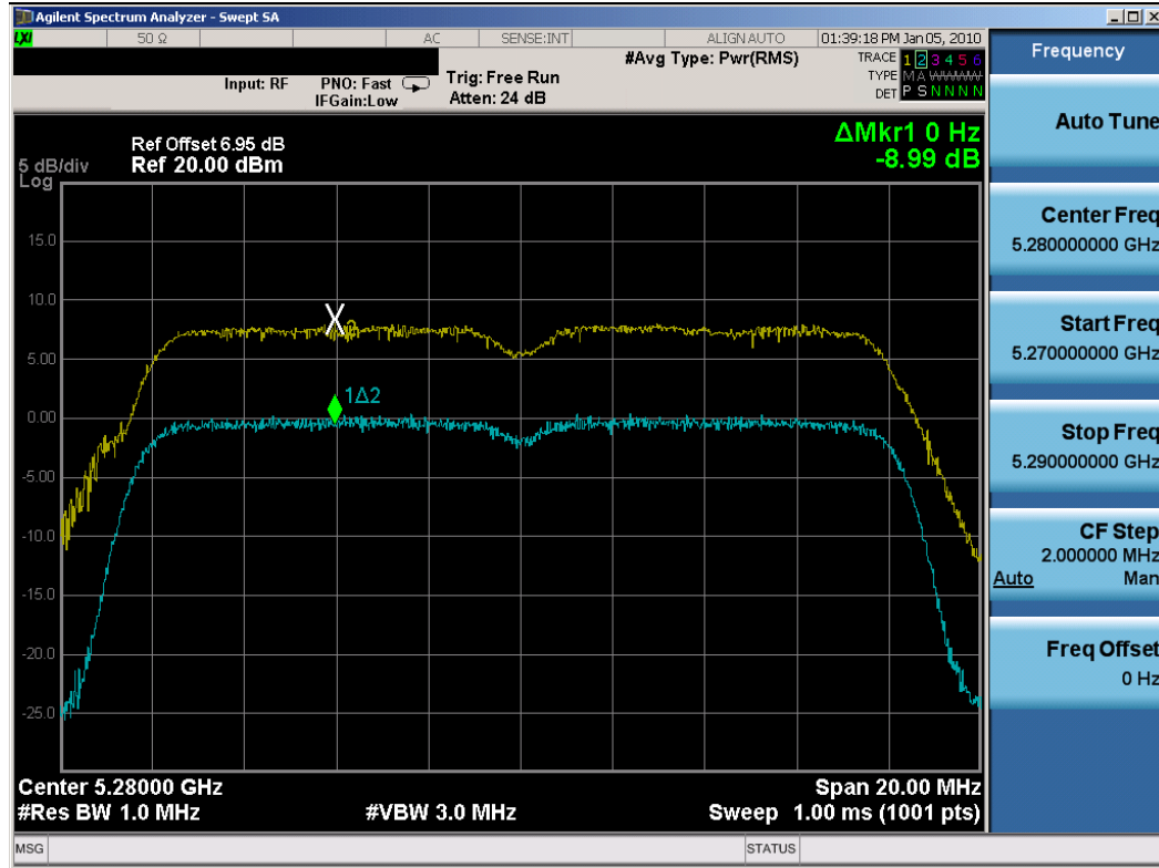
Plot 6-62. Peak Excursion Ratio Plot (802.11a (UNII) – Ch. 56) – Chain A
