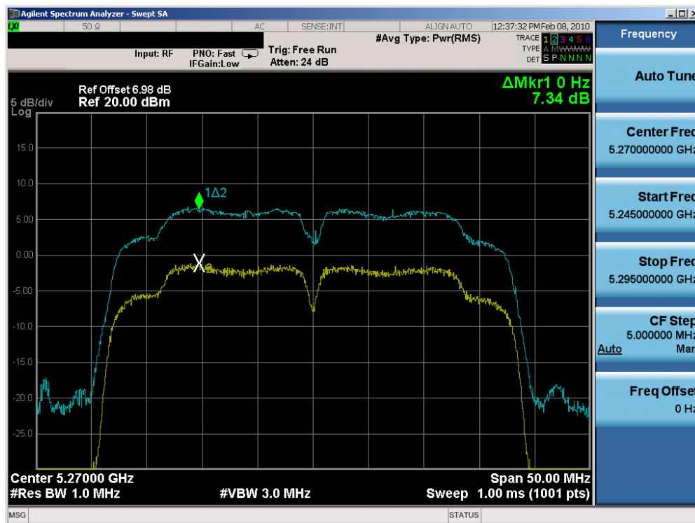
Plot 6-85. Peak Excursion Ratio Plot (802.11n (UNII) – Ch. 54) – Chain B
