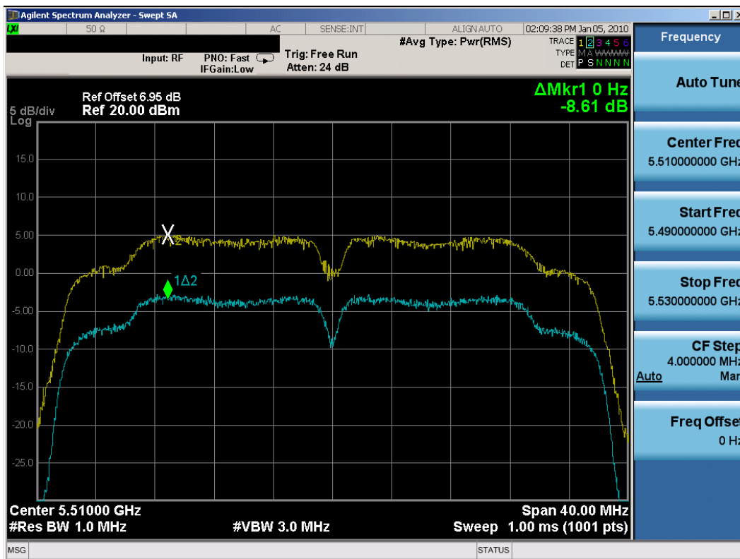
Plot 6-71. Peak Excursion Ratio Plot (802.11n (UNII) - Ch. 102) - Chain A
