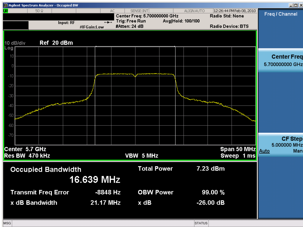
Plot 6-25. 26dB Bandwidth Plot (802.11a (UNII) – Ch. 140) – Chain B
