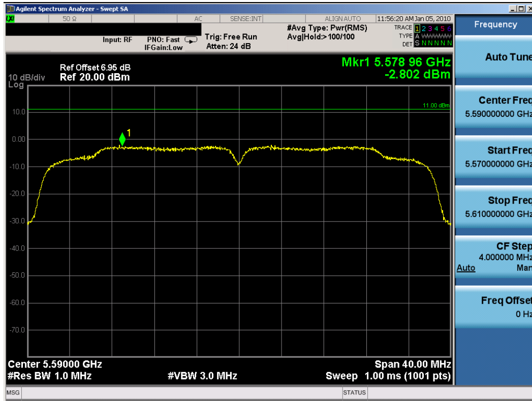
Plot 6-47. Peak Power Spectral Density Plot (802.11n (UNII) – Ch. 118) – Chain A
