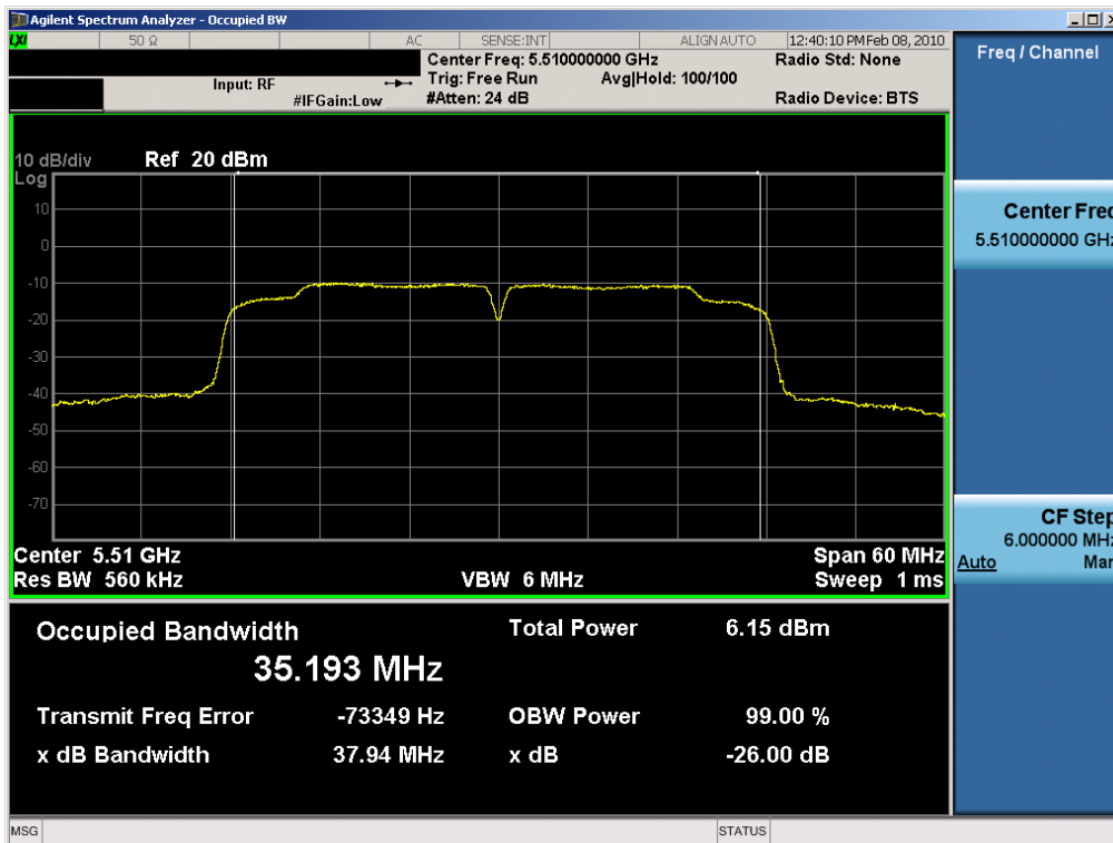
Plot 6-30. 26dB Bandwidth Plot (802.11n (UNII) – Ch. 102) – Chain B
