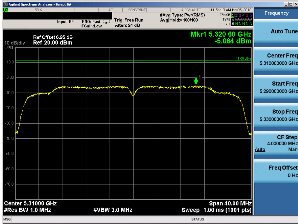
Plot 6-45. Peak Power Spectral Density Plot (802.11n (UNII) – Ch. 62) – Chain A
