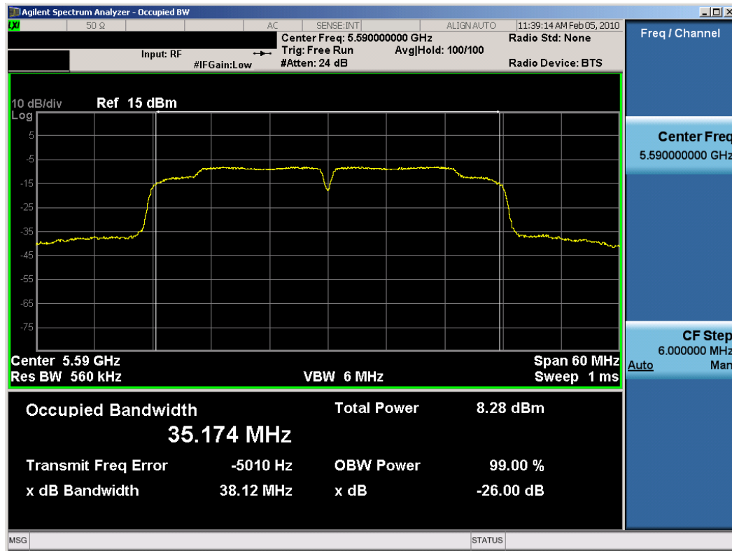
Plot 6-15. 26dB Bandwidth Plot (802.11n (UNII) – Ch. 118) – Chain A
