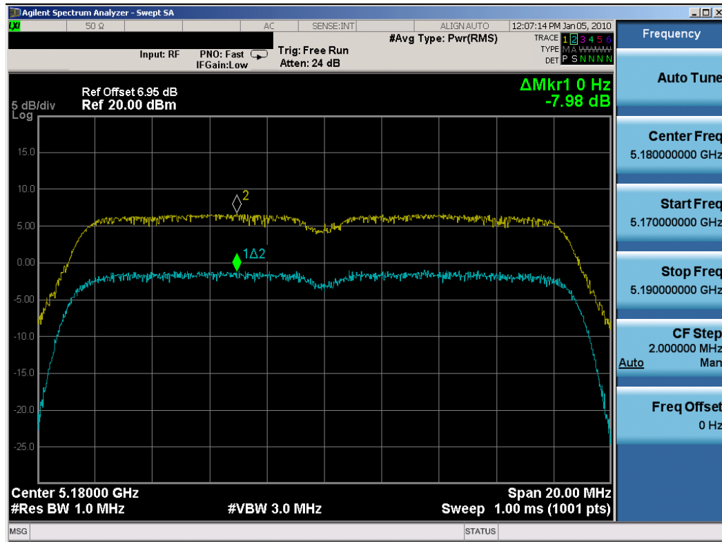
Plot 6-58. Peak Excursion Ratio Plot (802.11a (UNII) – Ch. 36) – Chain A
