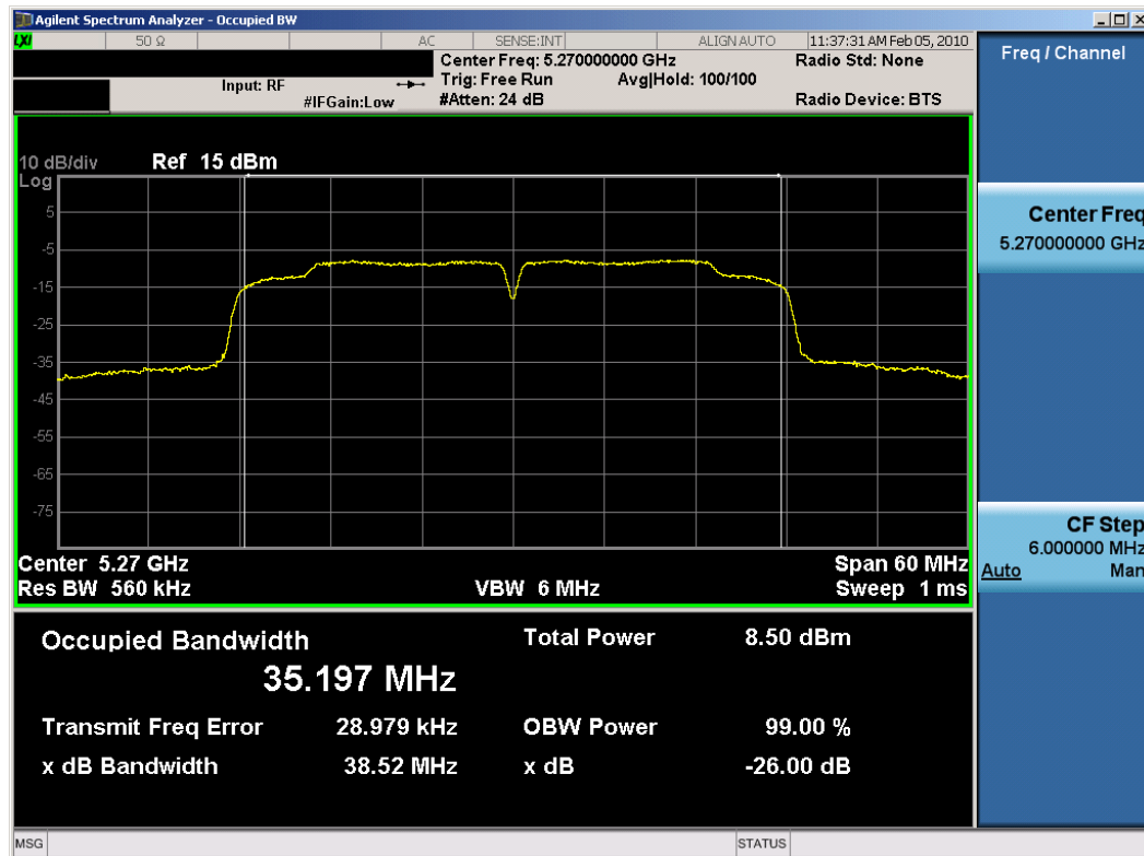
Plot 6-12. 26dB Bandwidth Plot (802.11n (UNII) – Ch. 54) – Chain A
