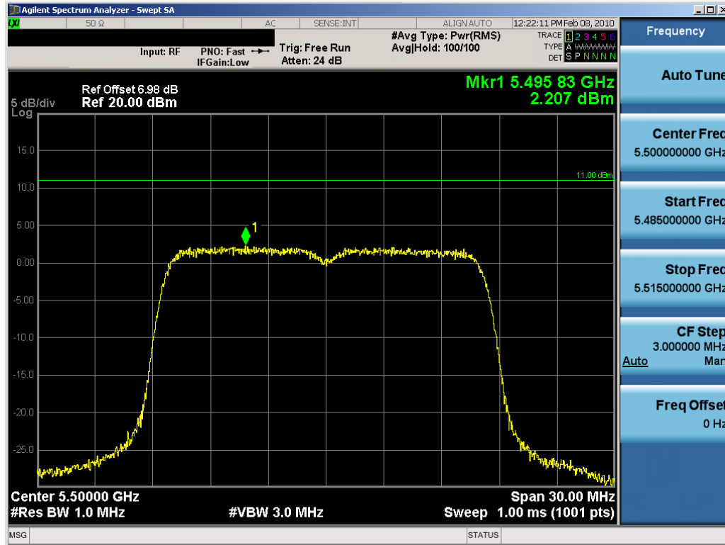
Plot 6-55. Peak Power Spectral Density Plot (802.11a (UNII) – Ch. 100) – Chain B
