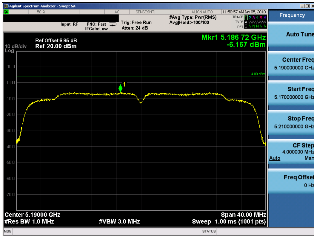
Plot 6-42. Peak Power Spectral Density Plot (802.11n (UNII) – Ch. 38) – Chain A
