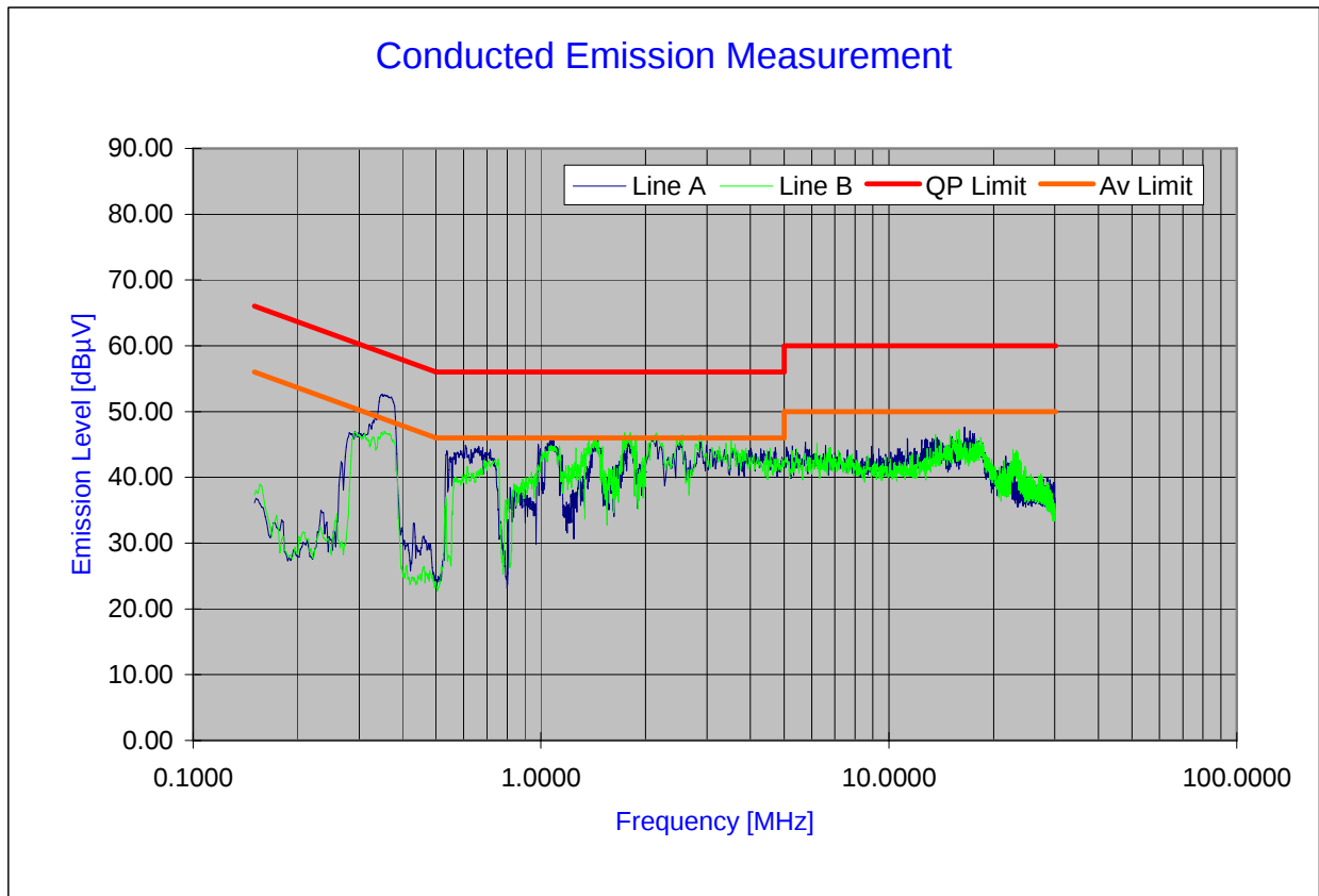
Plot 6-91. Line Conducted Plot with 802.11a (UNII Band II)
