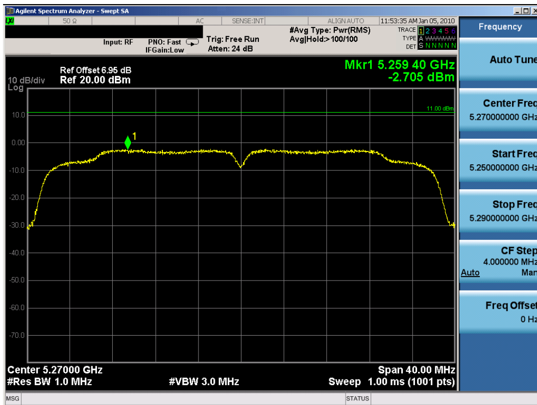
Plot 6-44. Peak Power Spectral Density Plot (802.11n (UNII) – Ch. 54) – Chain A
