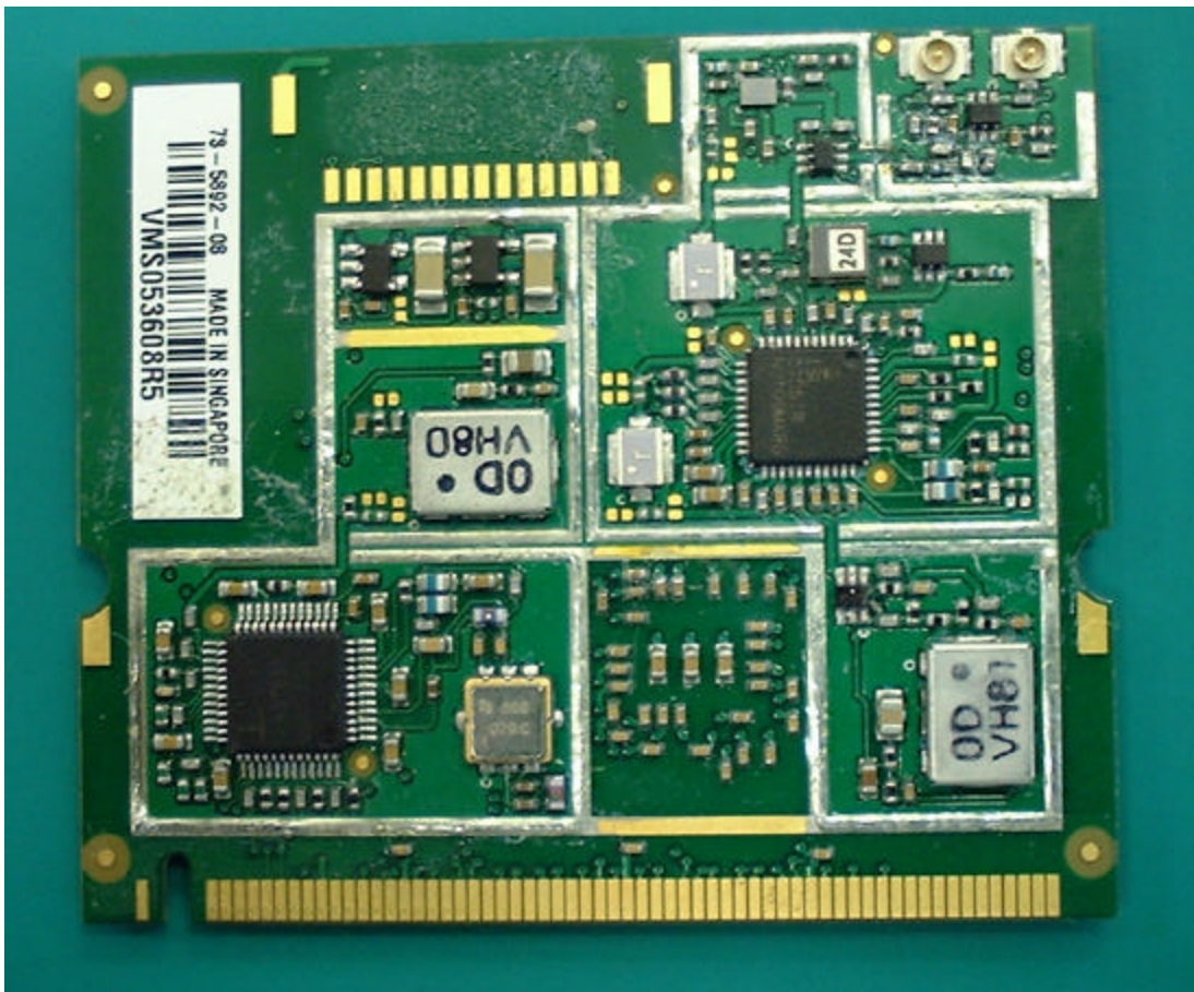
Internal photo of W-LAN Card (Front)
