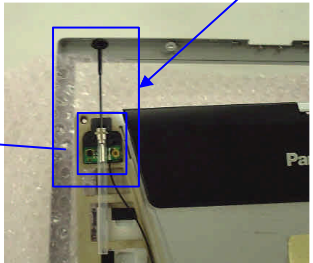
EGPRS whip Antenna
