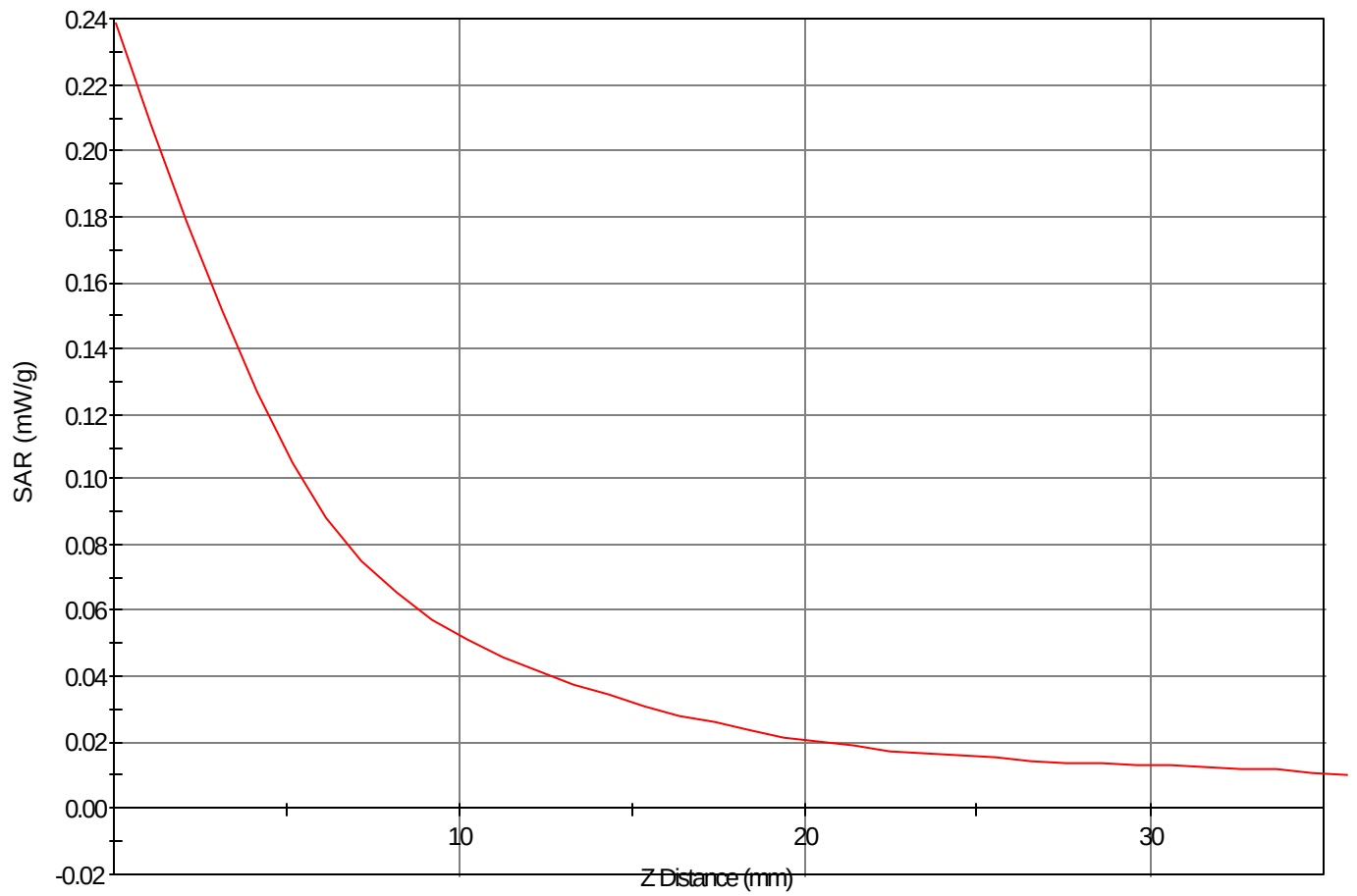
SAR - Z Axis at Hotspot x:-67.0 y:-3.0
