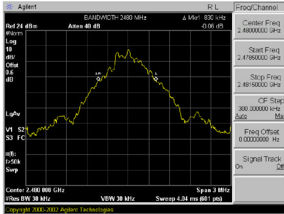
Plot A-3. 20dB Bandwidth Plot – Ch. 79
