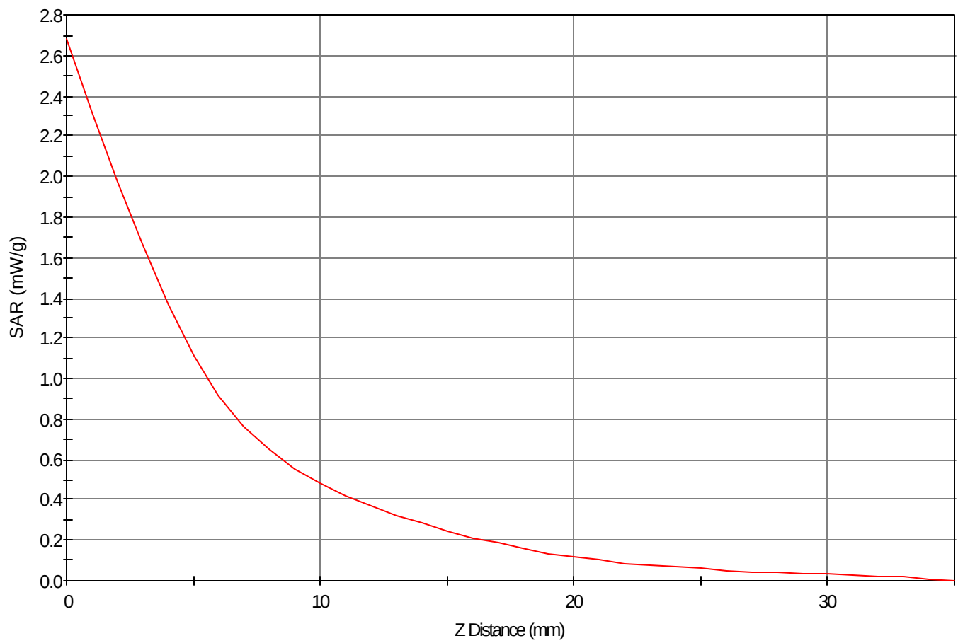
SAR - Z Axis at Hotspot x:0.0 y:3.0
