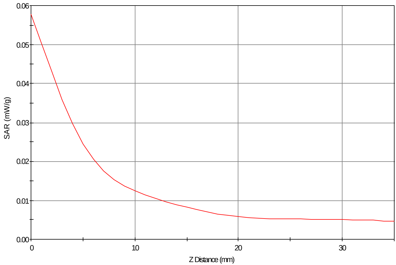
SAR - Z Axis at Hotspot x:-14.0 y:5.0
