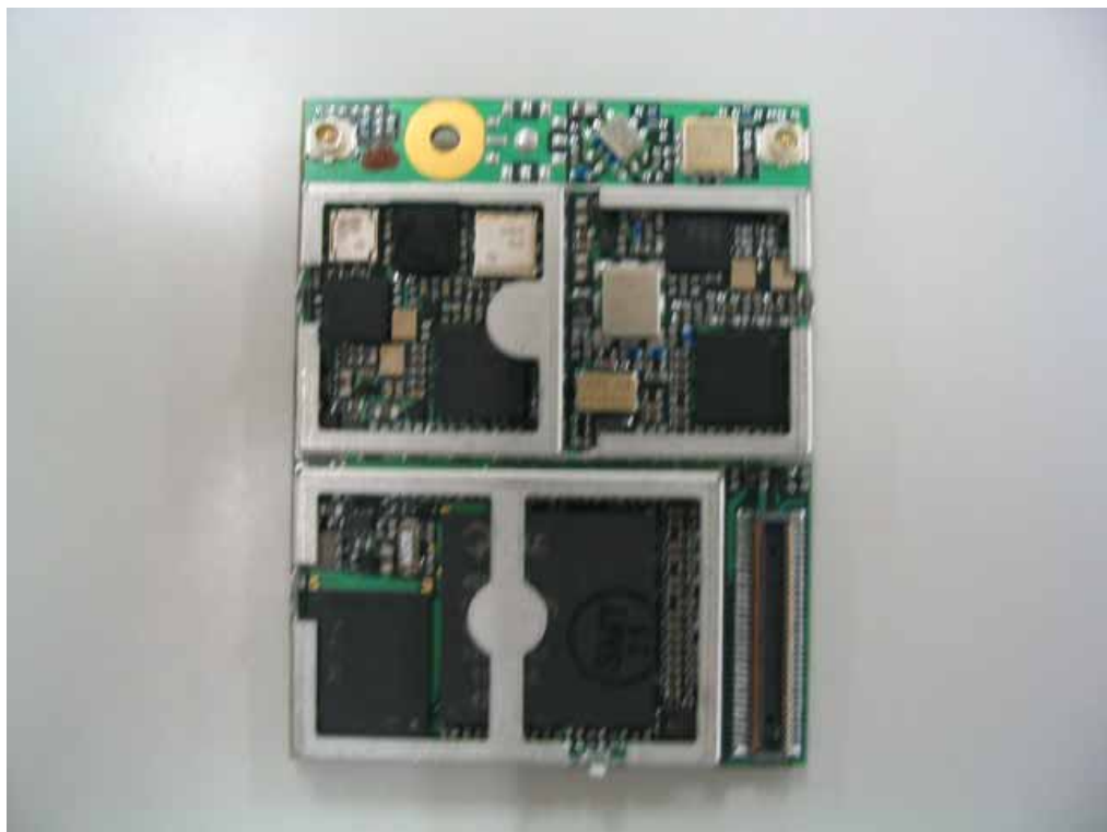
EM5625D Module Interior Bottom View
