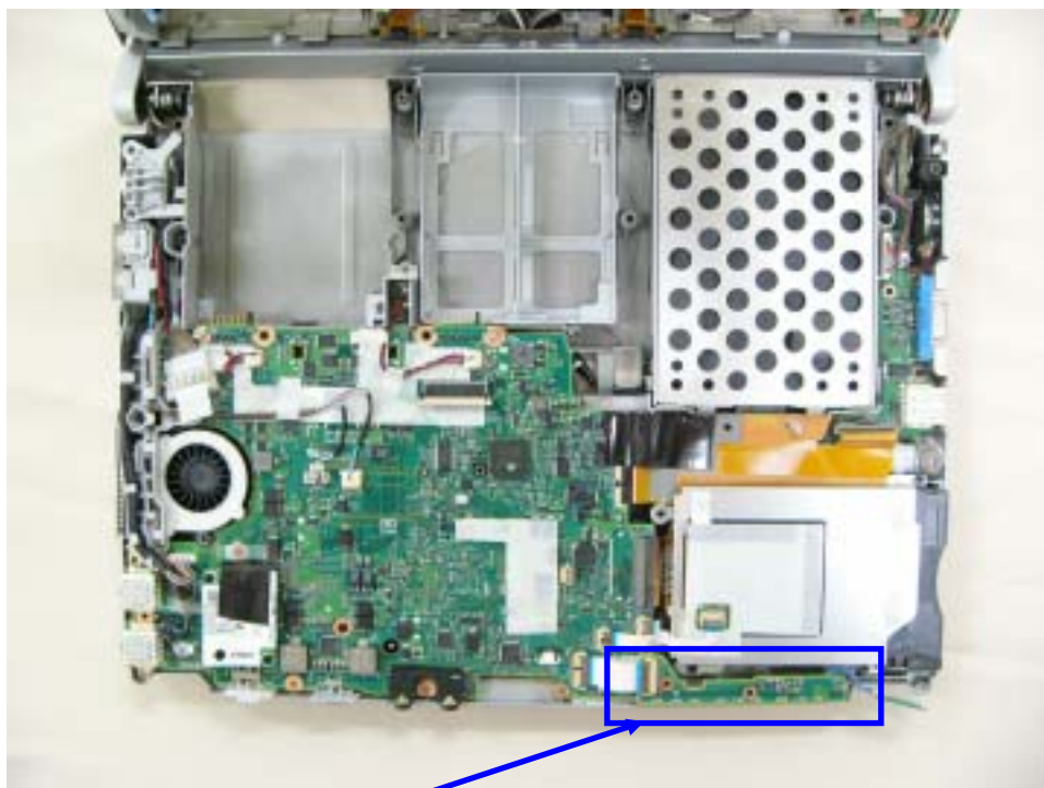
Bluetooth board
