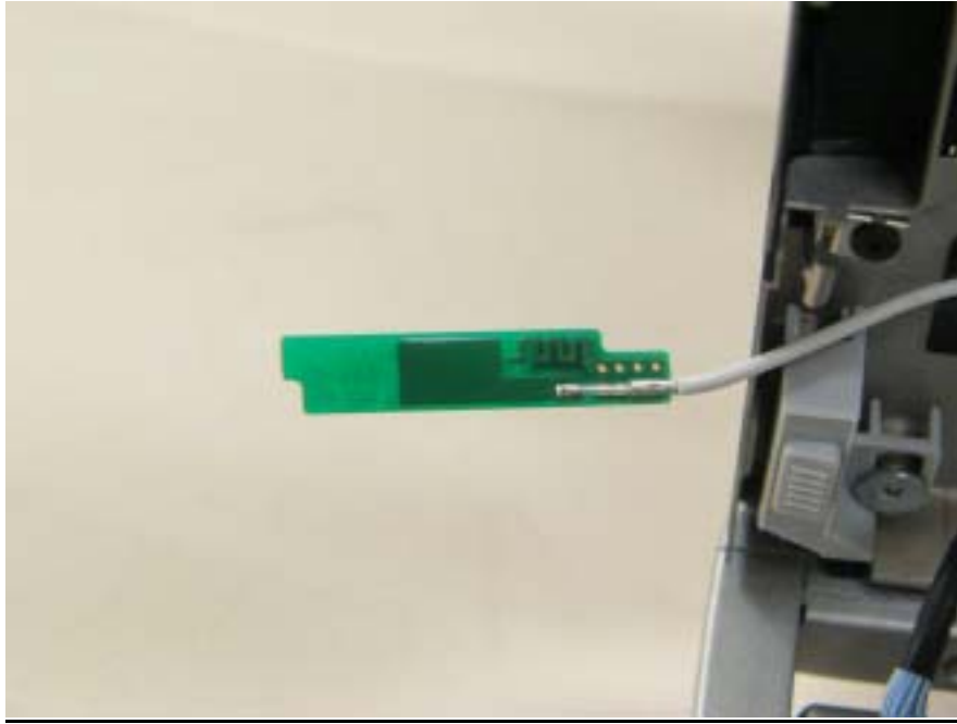
WLAN Aux TX/RX antenna magnified view (Bottom)
