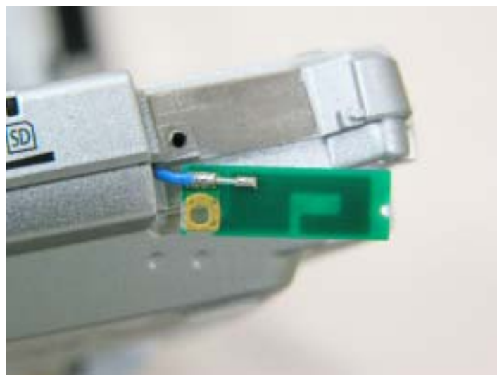
Bluetooth TX/RX Antenna (Bottom)
