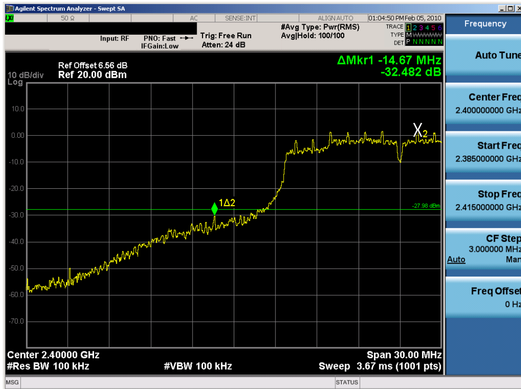
Plot 6-41. Band Edge Plot (802.11g- Ch. 1) – Chain B
