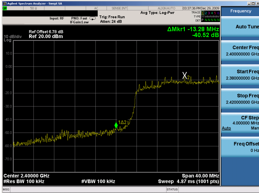
Plot 6-35. Band Edge Plot (802.11n (2.4GHz) – Ch. 3) – Chain A
