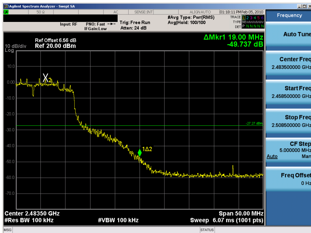
Plot 6-42. Band Edge Plot (802.11g – Ch. 11) – Chain B
