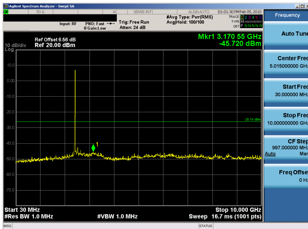
Plot 6-66. Conducted Spurious Plot (802.11b – Ch. 6) – Chain B
