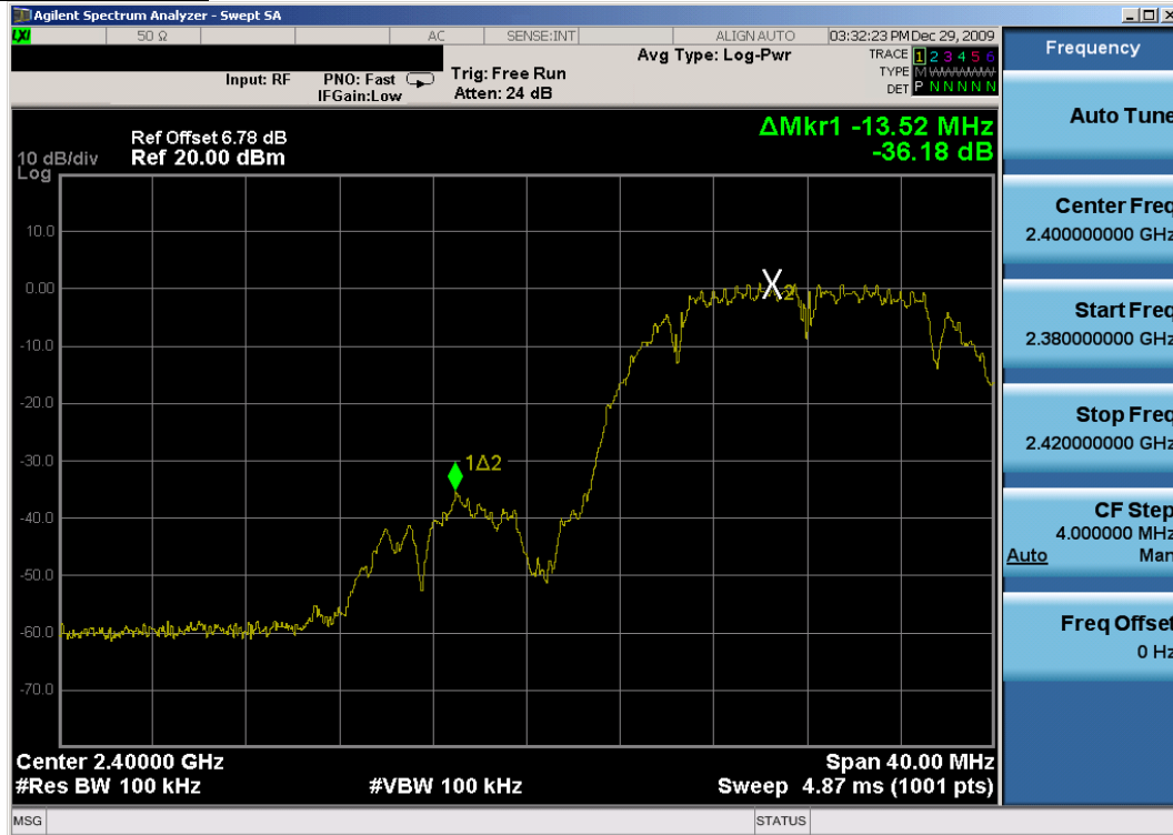
Plot 6-29. Band Edge Plot (802.11b – Ch. 1) – Chain A
