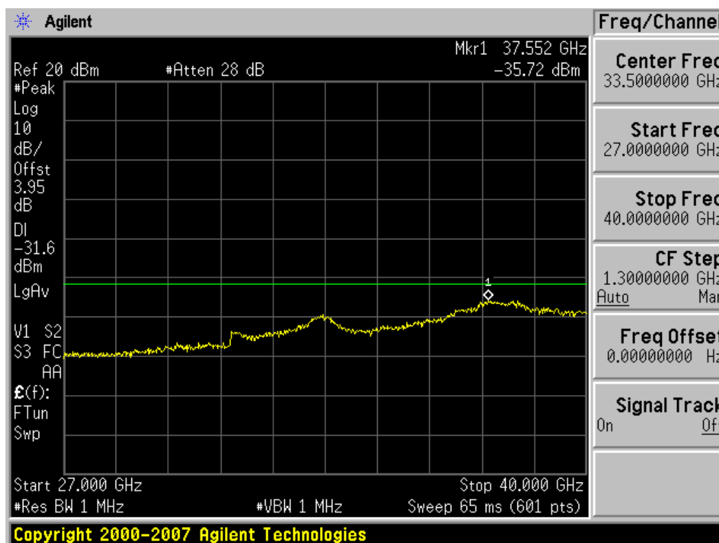
Plot 6-60. Conducted Spurious Plot (802.11a – Ch. 157) – Chain A
