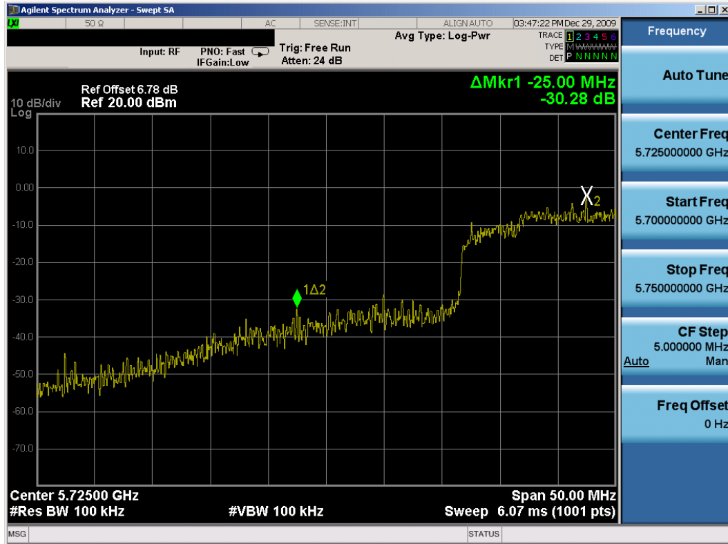
Plot 6-37. Band Edge Plot (802.11n (5.8GHz) – Ch. 151) – Chain A
