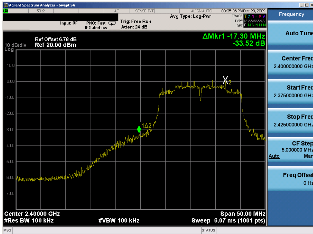
Plot 6-31. Band Edge Plot (802.11g– Ch. 1) – Chain A
