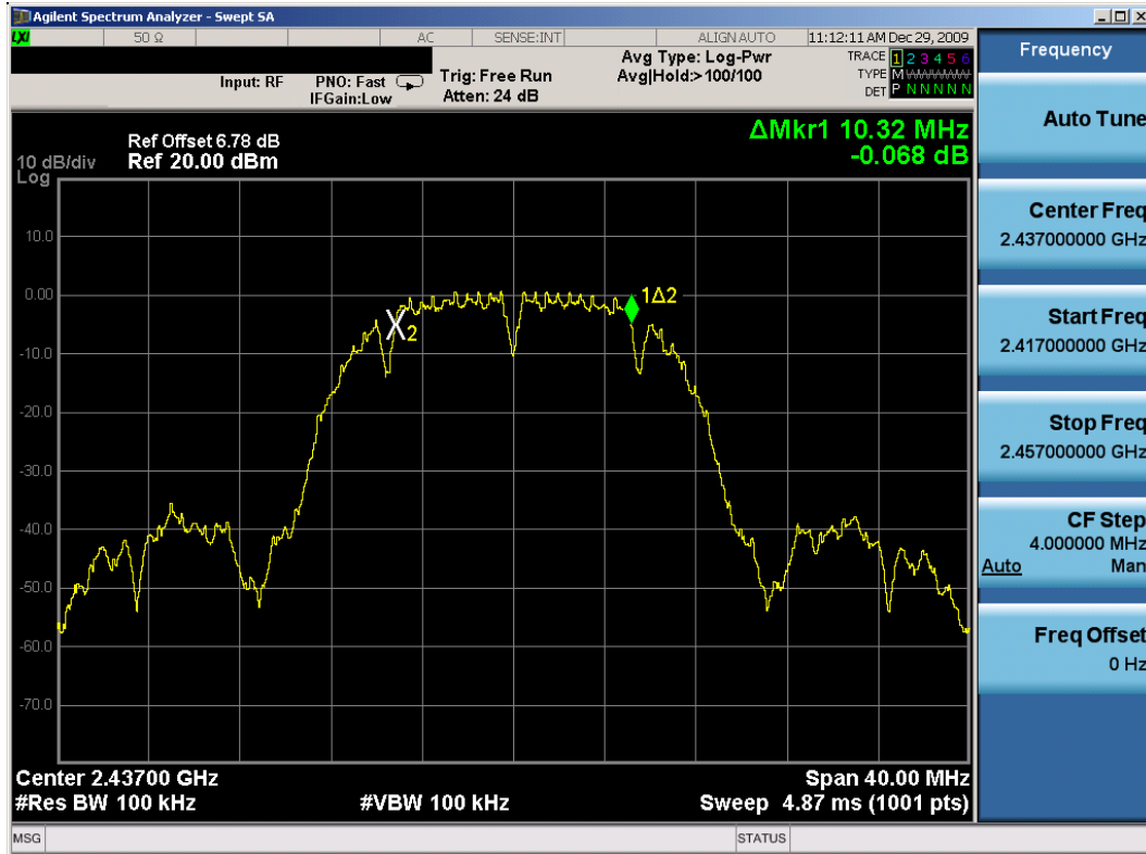
Plot 6-1. 6dB Bandwidth Plot (802.11b – Ch. 6) – Chain A
