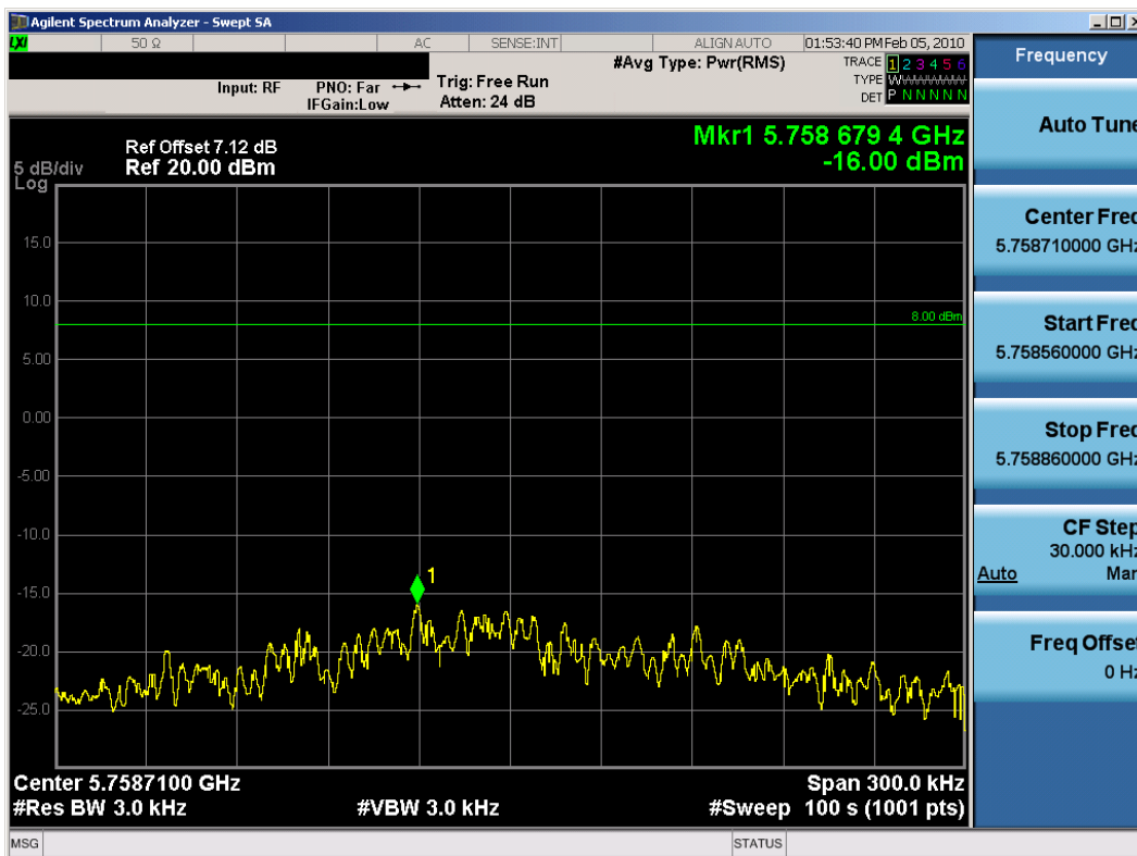
Plot 6-20. Power Spectral Density Plot (802.11n (5.8GHz) – Ch. 151) – Chain B
