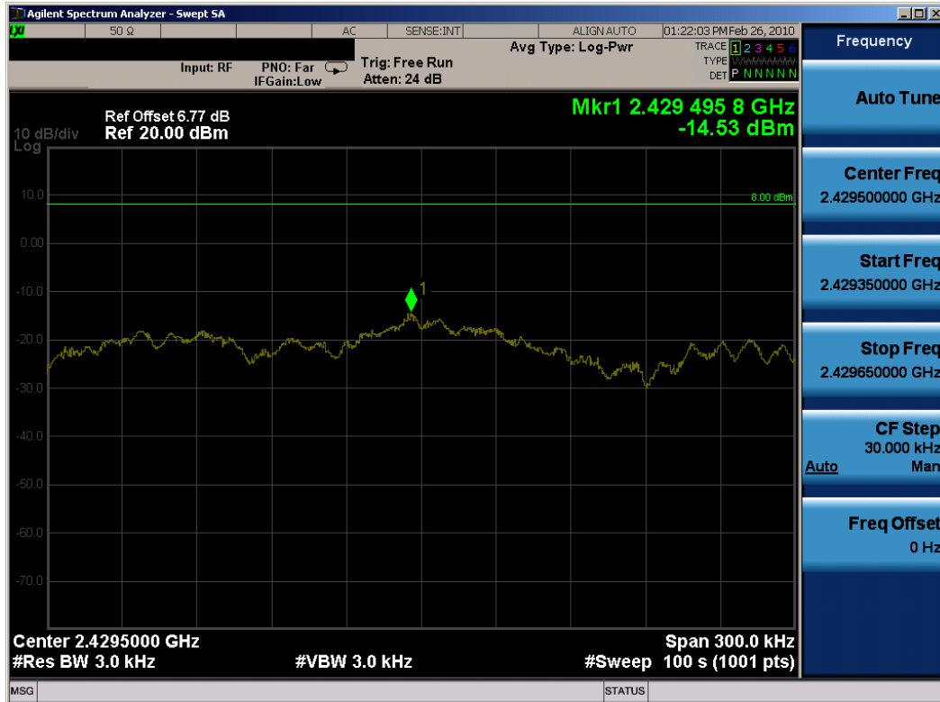
Plot 6-25. Power Spectral Density (802.11n (2.4GHz) Dual Transmit Mode – Ch. 6) – Chain A
