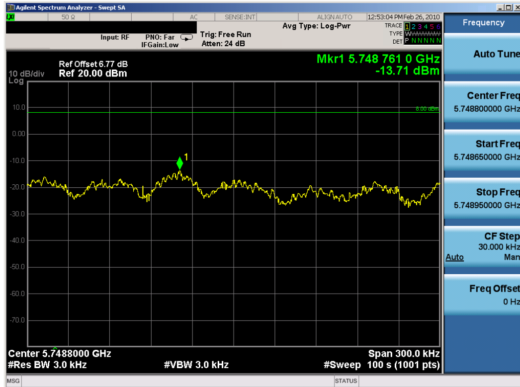
Plot 6-23. Power Spectral Density (802.11a Dual Transmit Mode – Ch. 149) – Chain A
