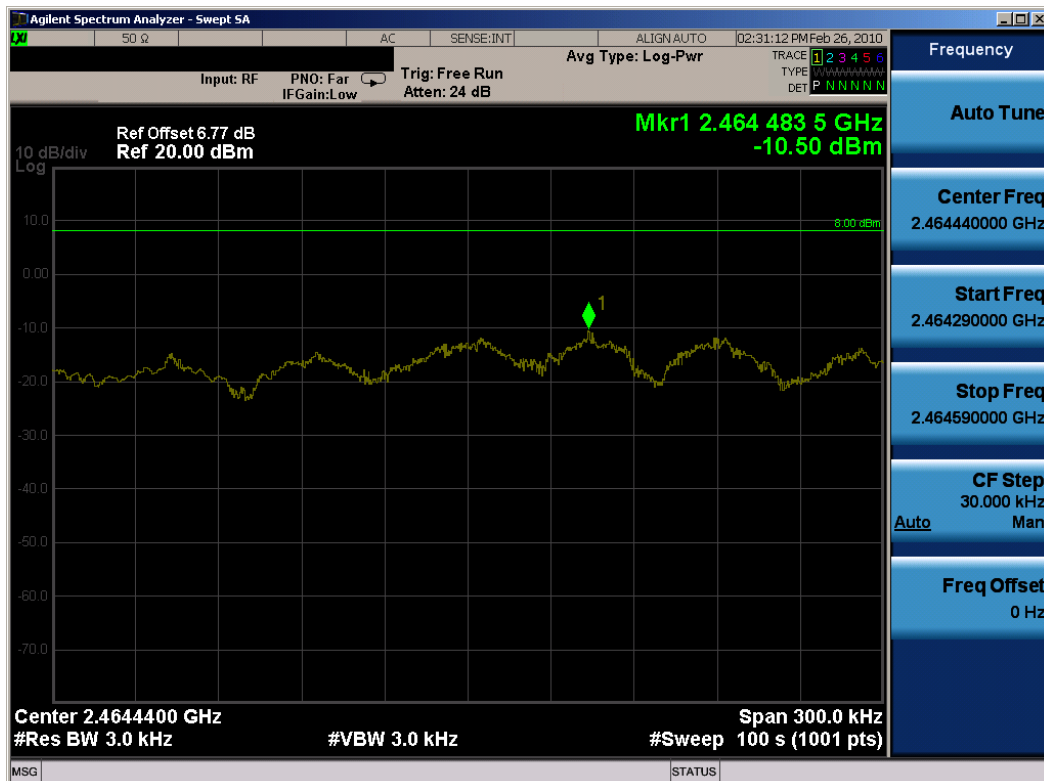
Plot 6-22. Power Spectral Density (802.11g Dual Transmit Mode – Ch. 11) – Chain B
