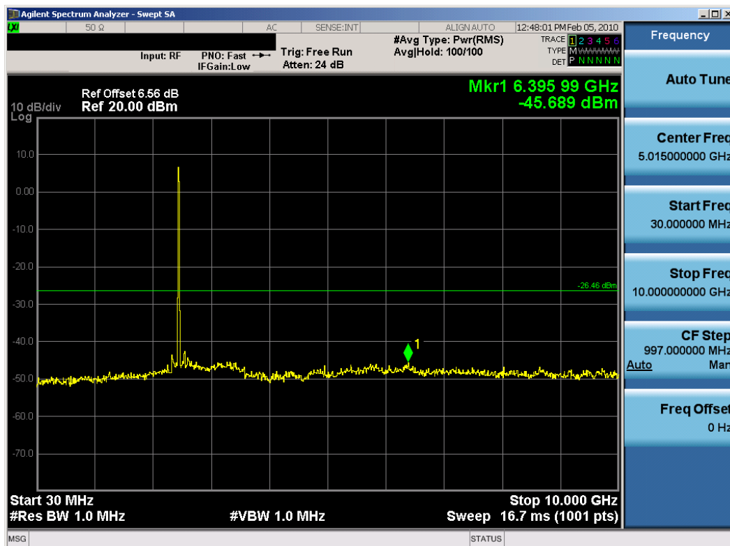
Plot 6-68. Conducted Spurious Plot (802.11b – Ch. 11) – Chain B
