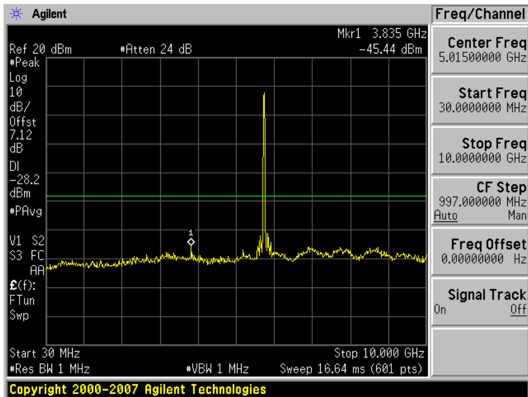
Plot 6-70. Conducted Spurious Plot (802.11a – Ch. 149) – Chain B
