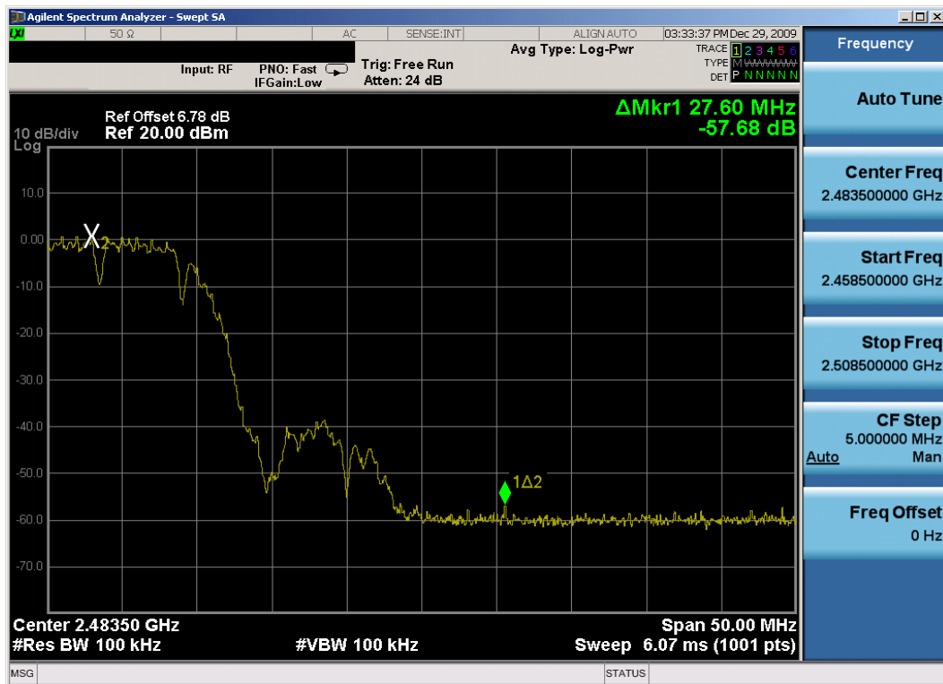
Plot 6-30. Band Edge Plot (802.11b – Ch. 11) – Chain A
