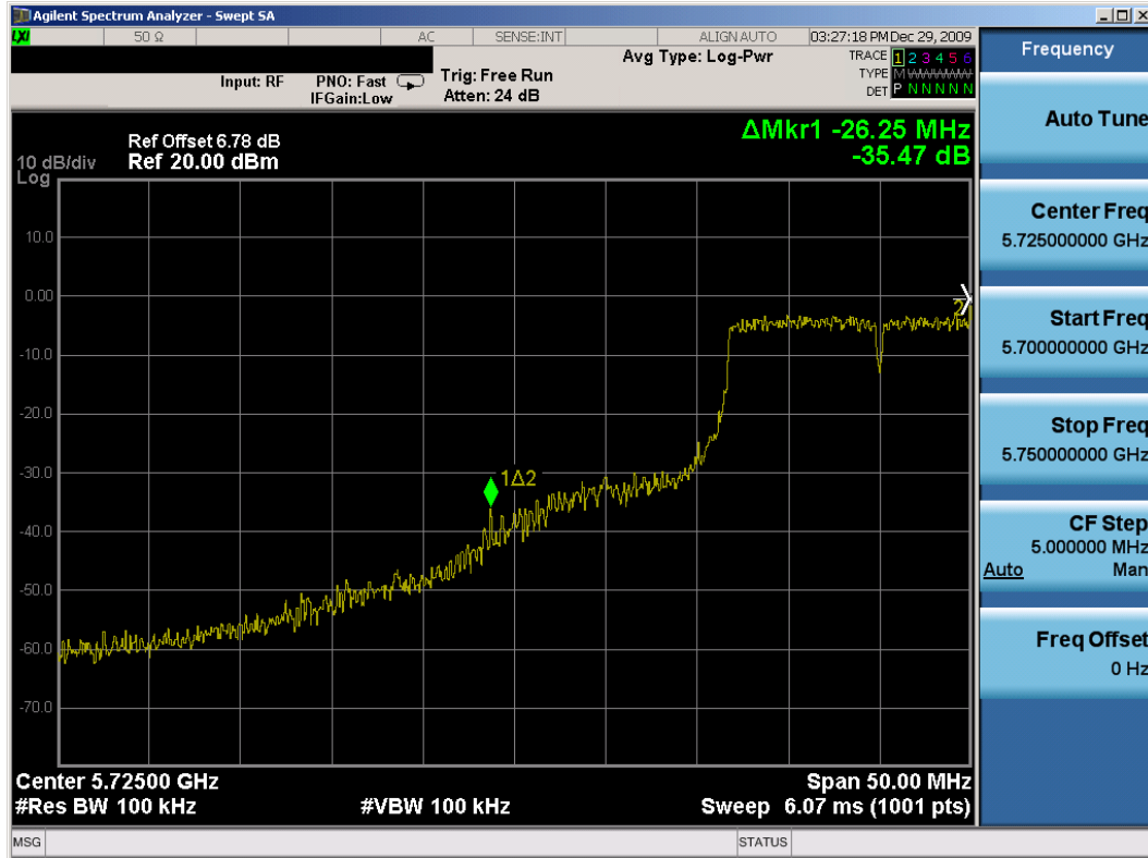
Plot 6-33. Band Edge Plot (802.11a – Ch. 149) – Chain A
