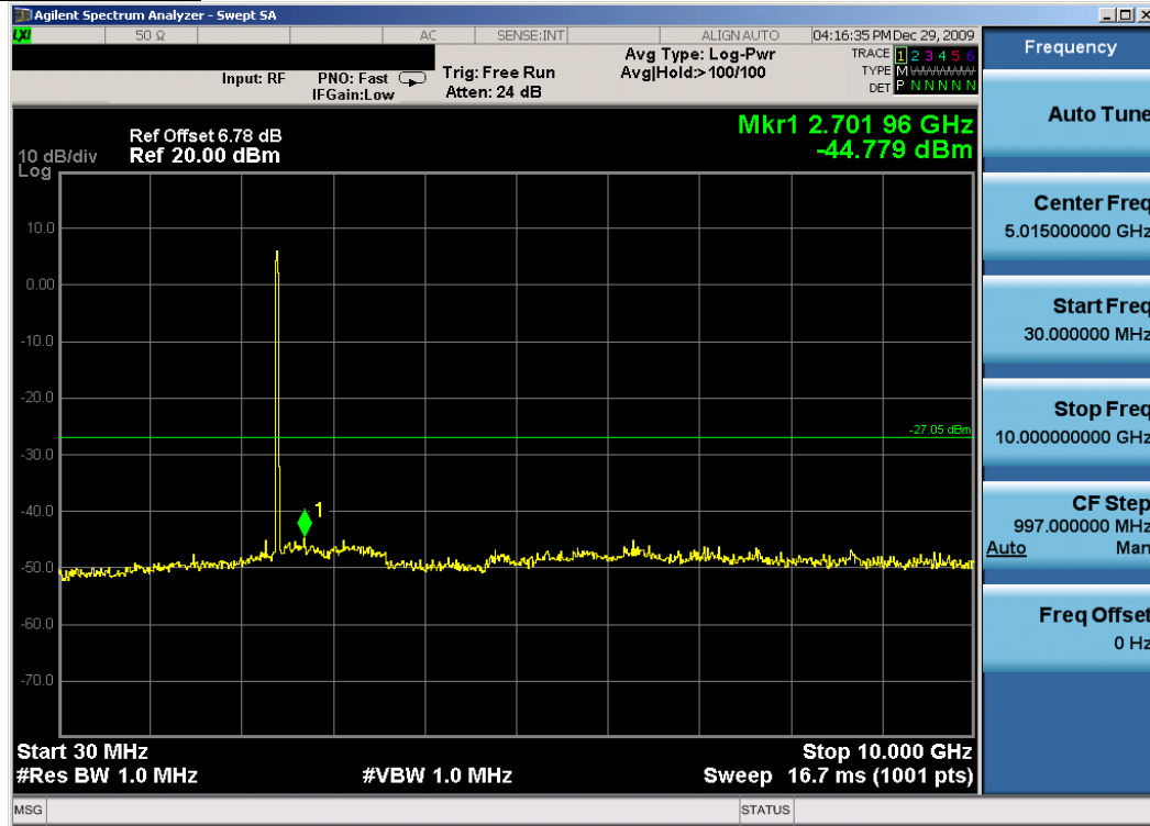
Plot 6-49. Conducted Spurious Plot (802.11b – Ch. 1) – Chain A
