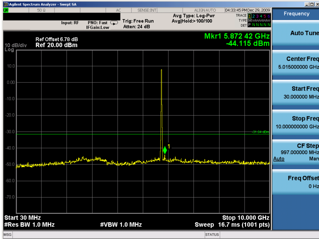
Plot 6-55. Conducted Spurious Plot (802.11a – Ch. 149) – Chain A
