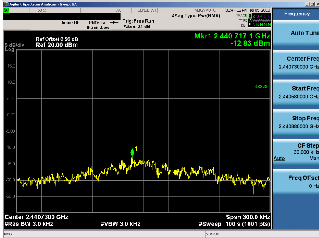
Plot 6-19. Power Spectral Density Plot (802.11n (2.4GHz) – Ch. 6) – Chain B
