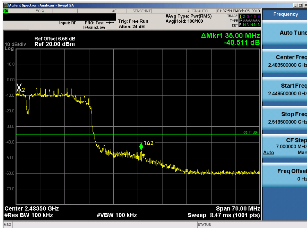
Plot 6-46. Band Edge Plot (802.11n (2.4GHz) – Ch. 9) – Chain B
