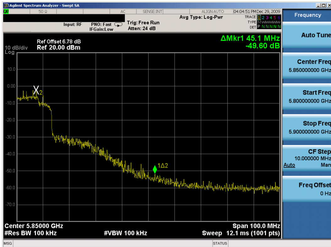
Plot 6-38. Band Edge Plot (802.11n (5.8GHz) – Ch. 159) – Chain A
