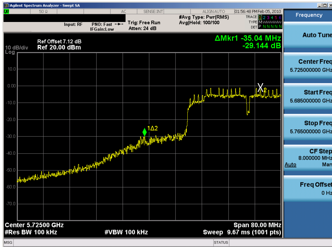
Plot 6-47. Band Edge Plot (802.11n (5.8GHz) – Ch. 151) – Chain B
