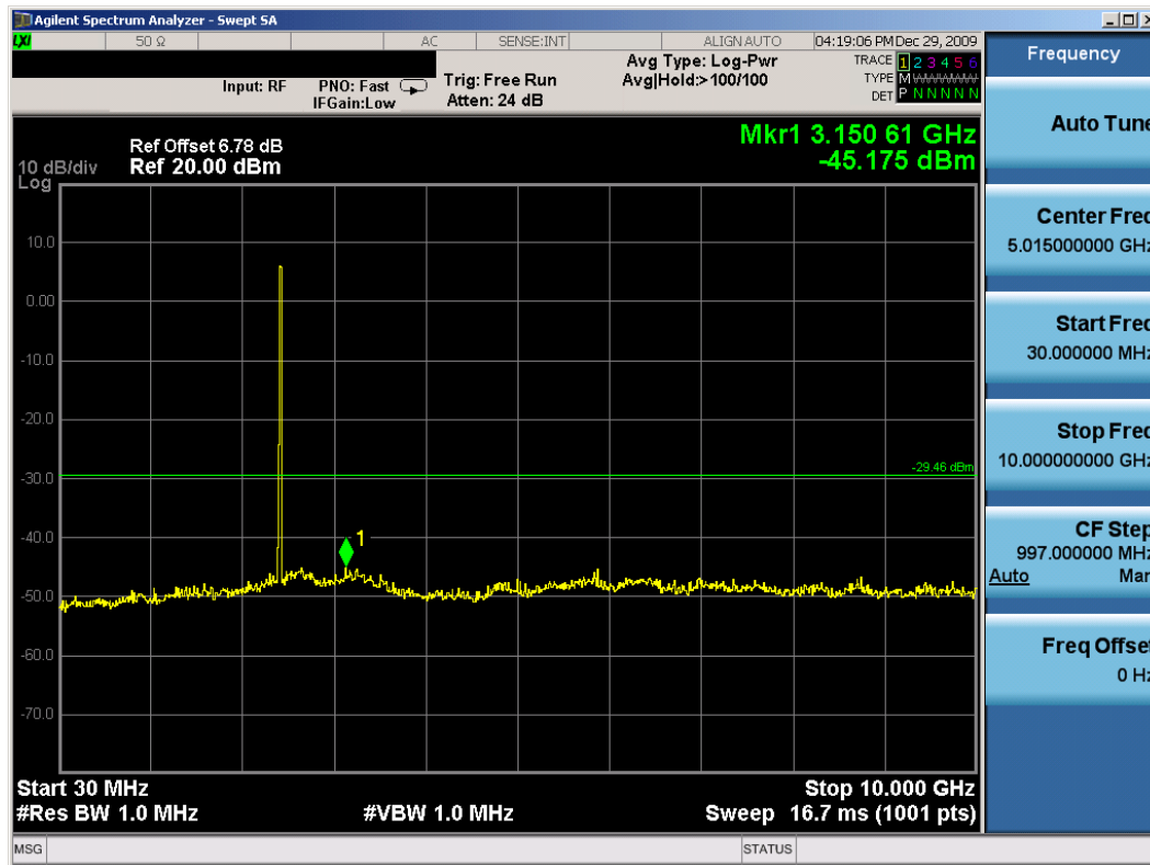
Plot 6-51. Conducted Spurious Plot (802.11b – Ch. 6) – Chain A
