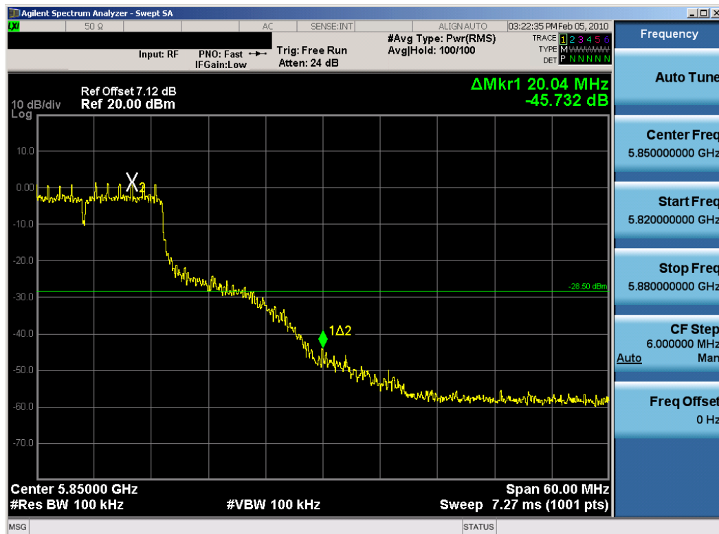
Plot 6-44. Band Edge Plot (802.11a – Ch. 165) – Chain B
