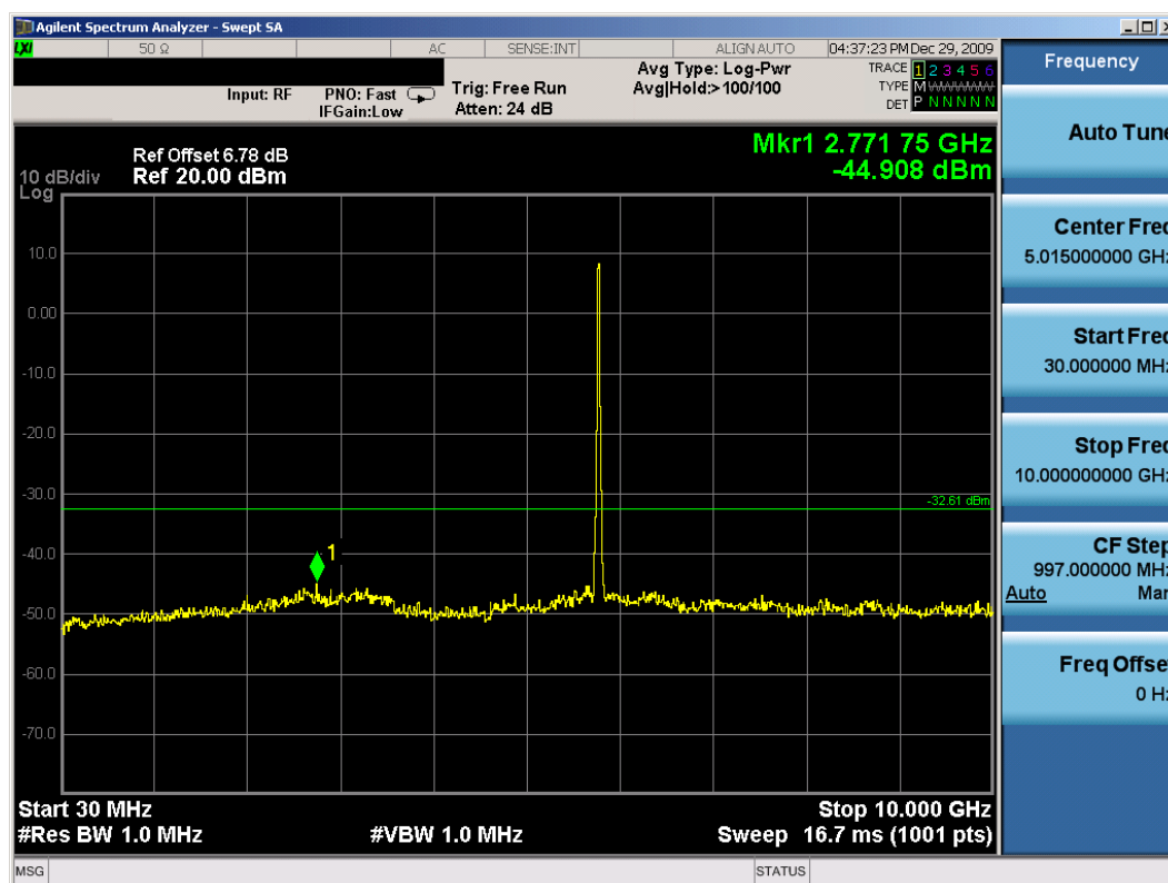
Plot 6-58. Conducted Spurious Plot (802.11a – Ch. 157) – Chain A
