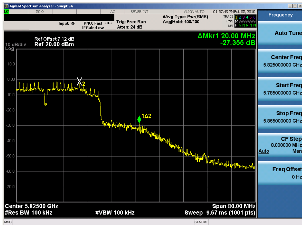
Plot 6-48. Band Edge Plot (802.11n (5.8GHz) – Ch. 159) – Chain B
