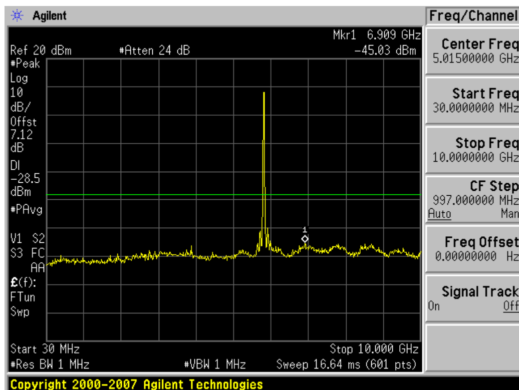
Plot 6-74. Conducted Spurious Plot (802.11a – Ch. 165) – Chain B
