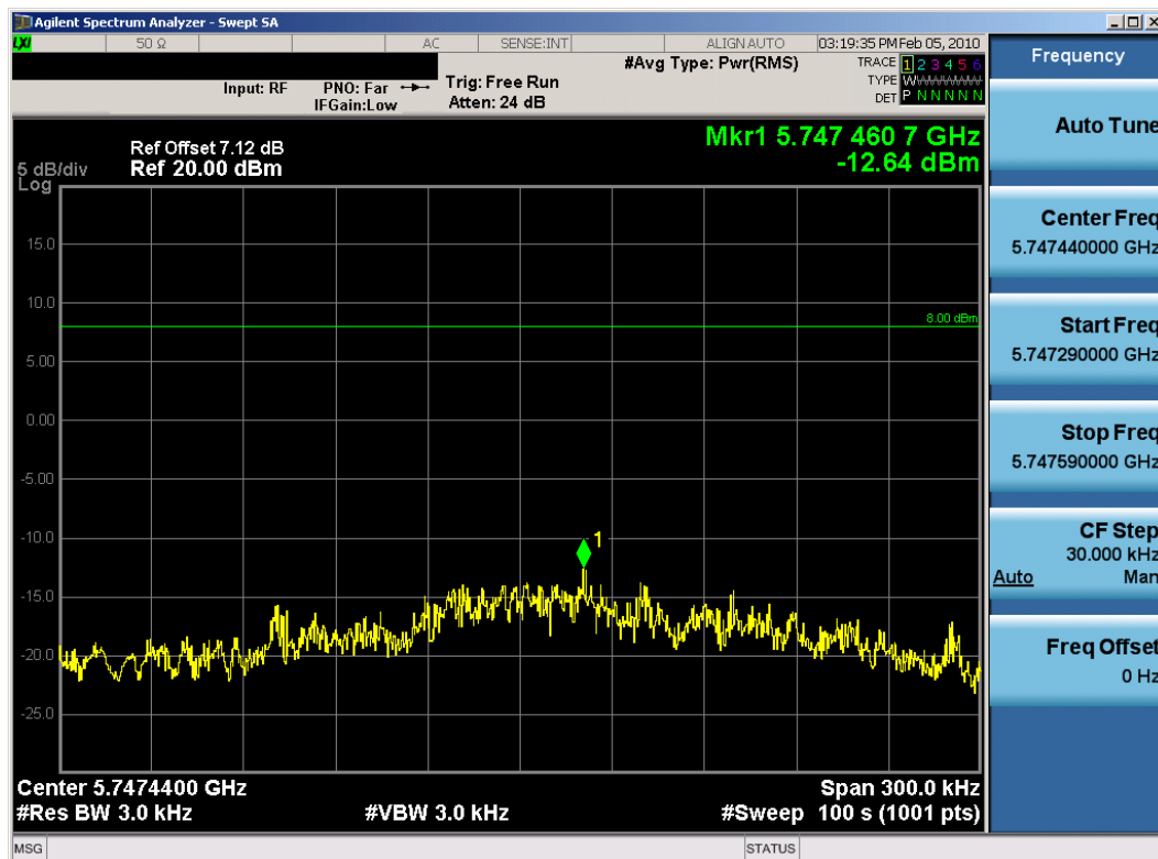
Plot 6-18. Power Spectral Density Plot (802.11a – Ch. 149) – Chain B
