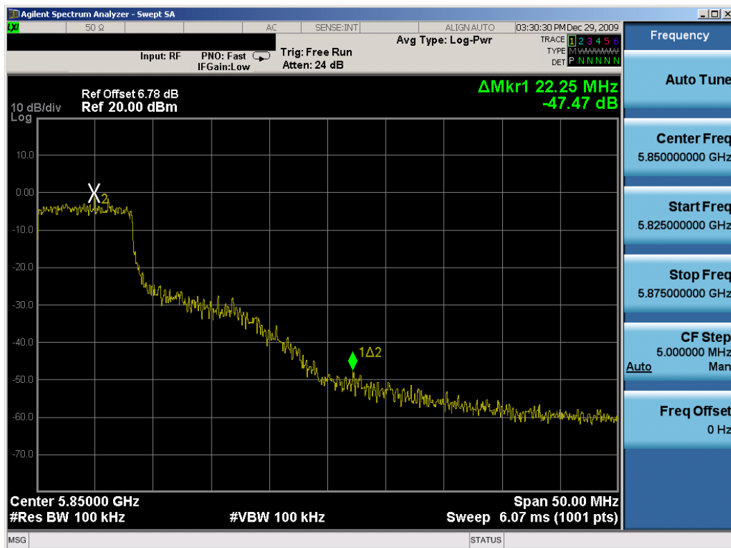
Plot 6-34. Band Edge Plot (802.11a – Ch. 165) – Chain A
