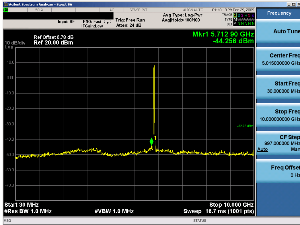
Plot 6-61. Conducted Spurious Plot (802.11a – Ch. 165) – Chain A
