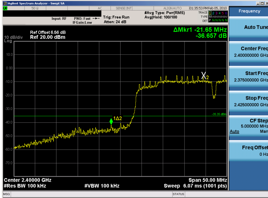
Plot 6-45. Band Edge Plot (802.11n (2.4GHz) – Ch. 3) – Chain B
