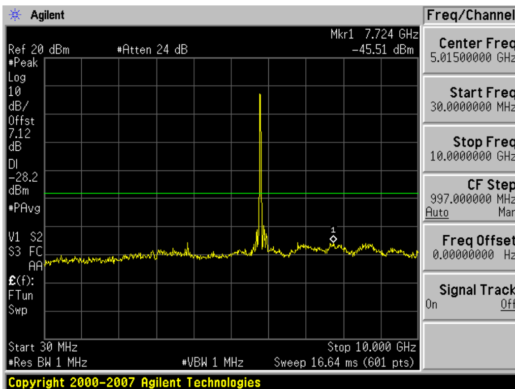
Plot 6-72. Conducted Spurious Plot (802.11a – Ch. 157) – Chain B
