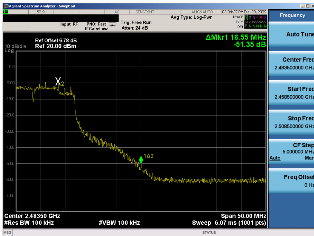
Plot 6-32. Band Edge Plot (802.11g – Ch. 11) – Chain A
