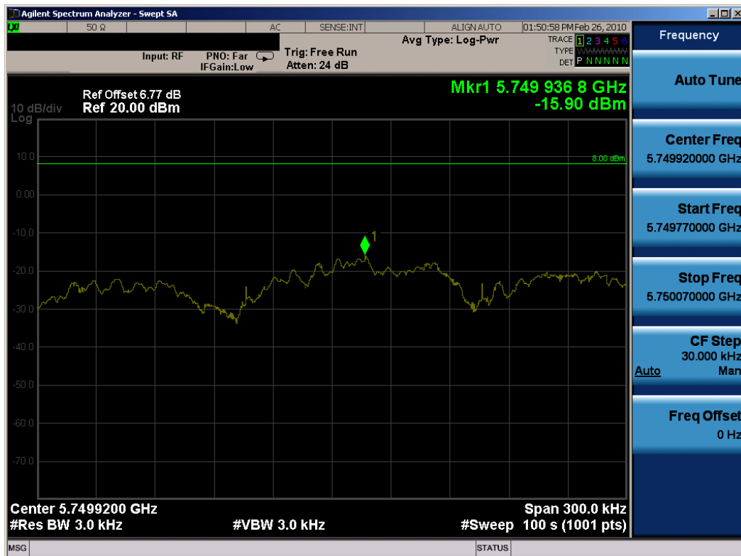
Plot 6-28. Power Spectral Density (802.11n (5.8GHz) Dual Transmit Mode – Ch. 151) – Chain B
