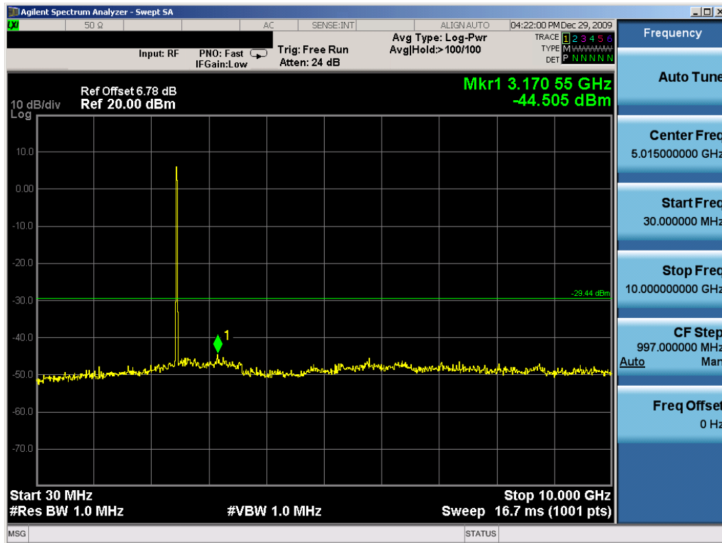
Plot 6-53. Conducted Spurious Plot (802.11b – Ch. 11) – Chain A
