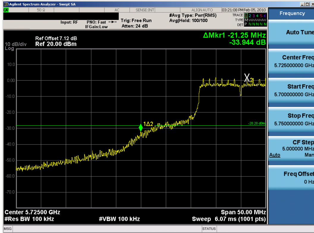
Plot 6-43. Band Edge Plot (802.11a – Ch. 149) – Chain B
