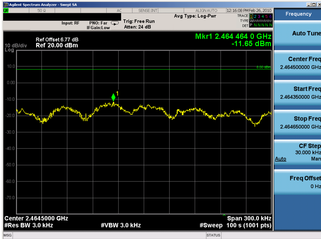
Plot 6-21. Power Spectral Density (802.11g Dual Transmit Mode – Ch. 11) – Chain A
