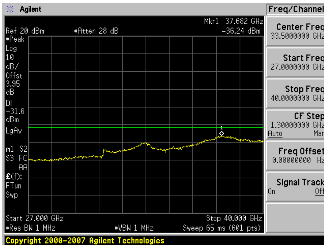
Plot 6-57. Conducted Spurious Plot (802.11a – Ch. 149) – Chain A
