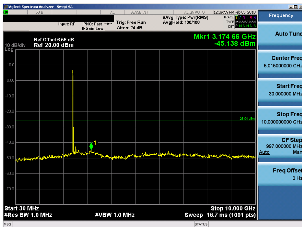
Plot 6-64. Conducted Spurious Plot (802.11b – Ch. 1) – Chain B
