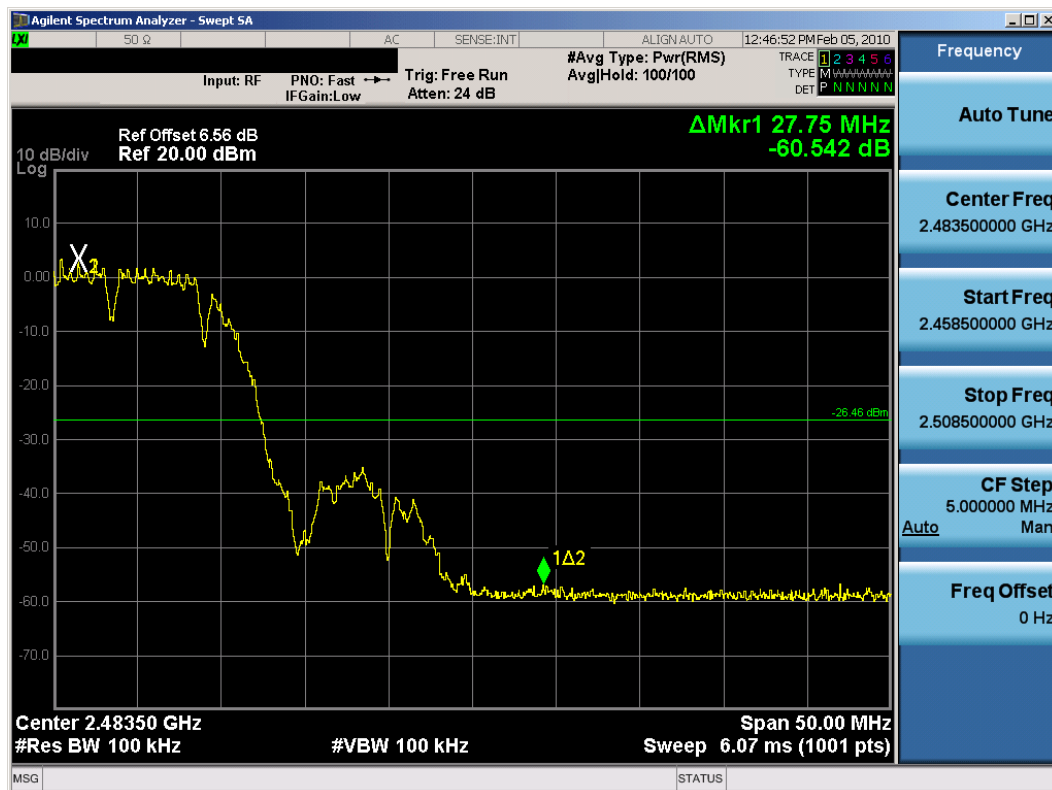
Plot 6-40. Band Edge Plot (802.11b – Ch. 11) – Chain B
