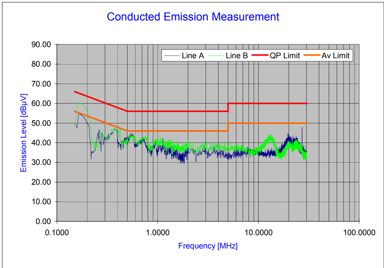
Plot 6-44. Line Conducted Plot with 802.11n (UNII Band II)
