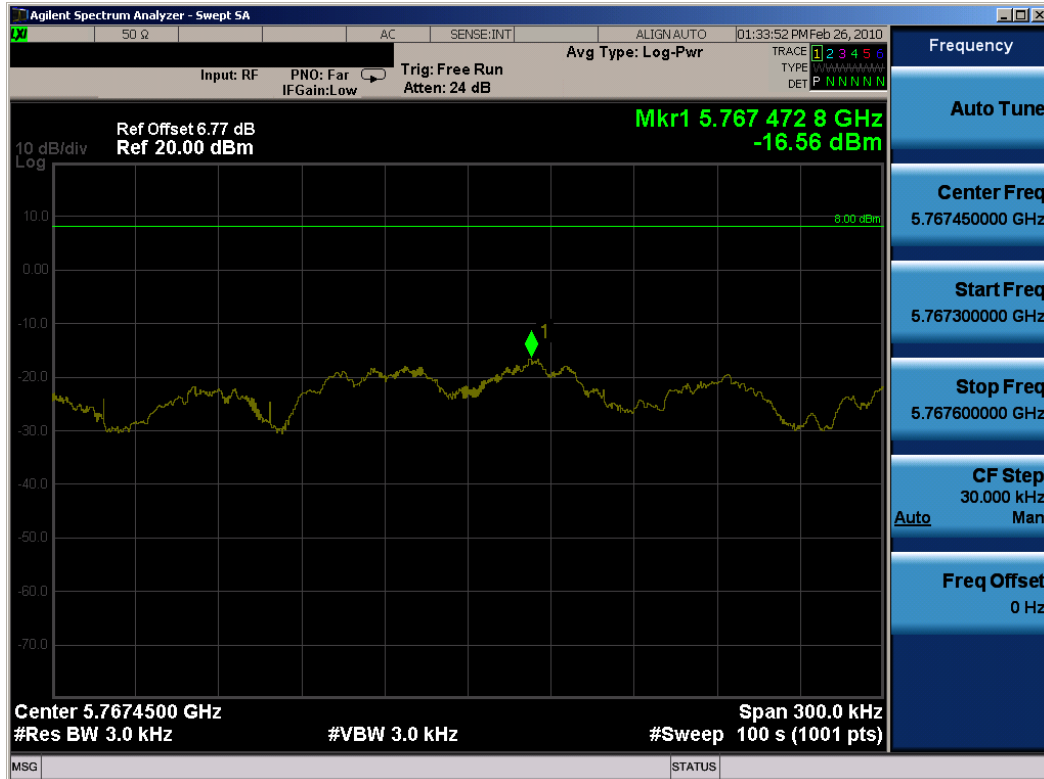
Plot 6-27. Power Spectral Density (802.11n (5.8GHz) Dual Transmit Mode – Ch. 151) – Chain A
