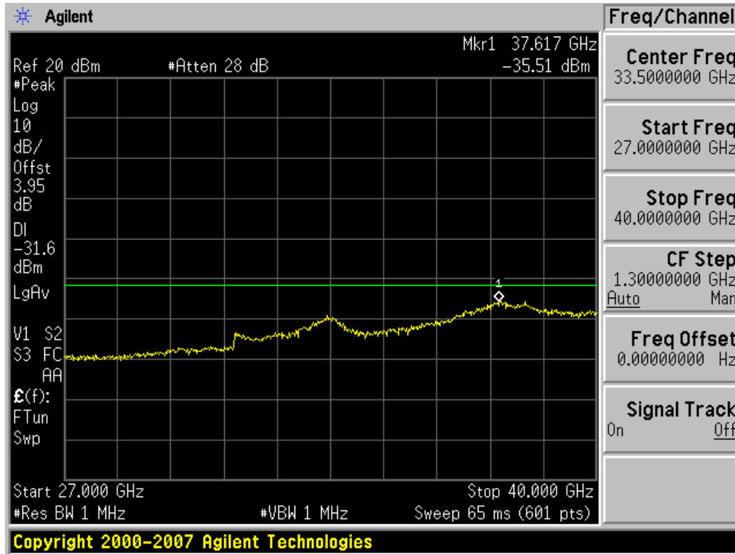
Plot 6-63. Conducted Spurious Plot (802.11a – Ch. 165) – Chain A
