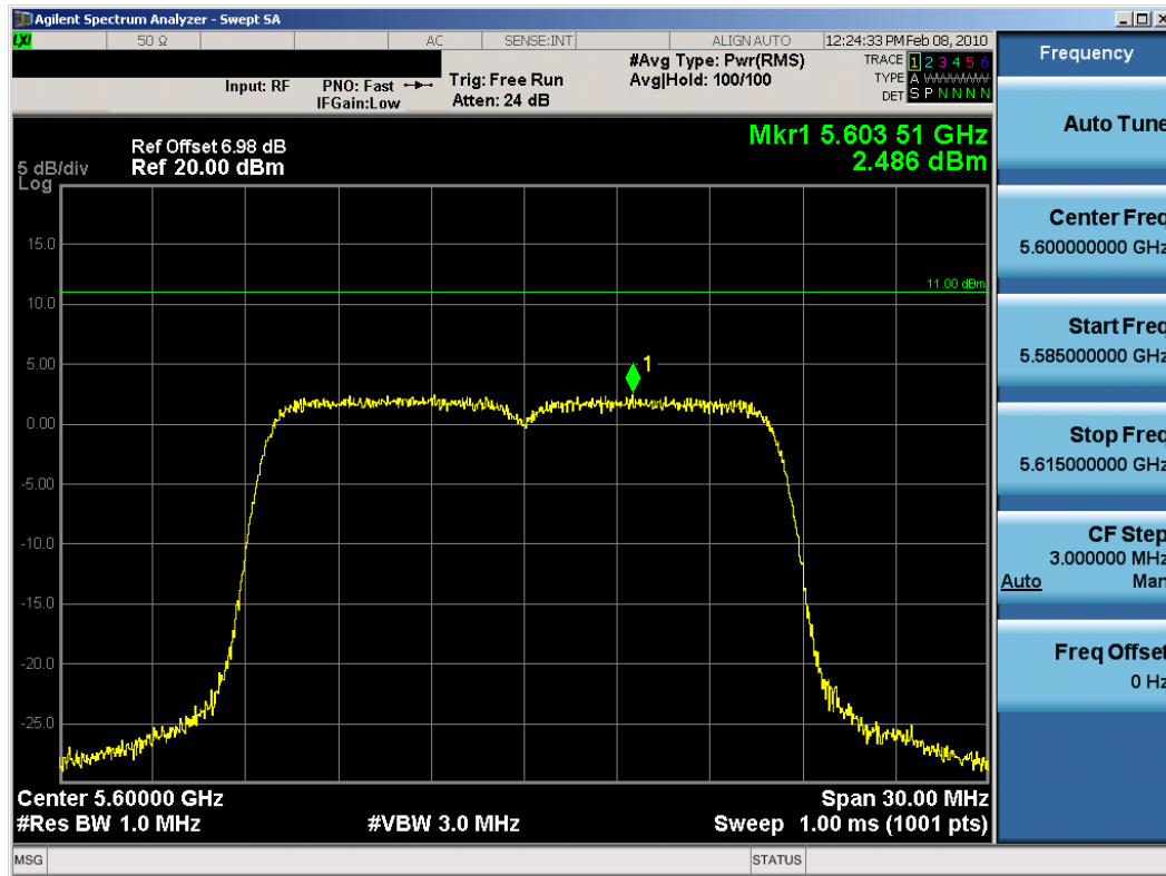
Plot 6-21. Peak Power Spectral Density Plot (802.11a (UNII) – Ch. 120) – Chain B
