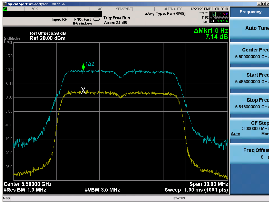
Plot 6-36. Peak Excursion Ratio Plot (802.11a (UNII) – Ch. 100) – Chain B
