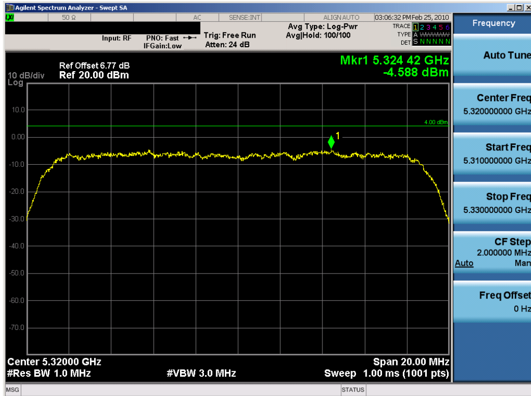
Plot 6-25. Peak Power Spectral Density (802.11a Dual Transmit Mode – Ch. 64) – Chain B
