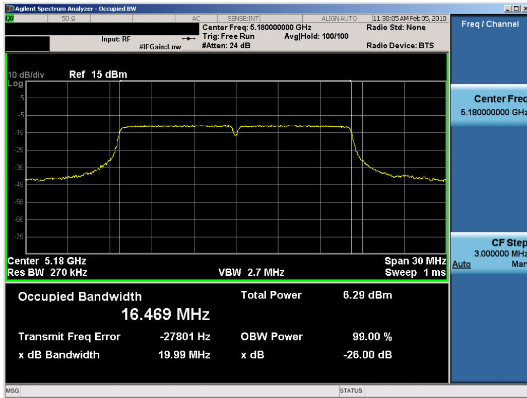
Plot 6-1. 26dB Bandwidth Plot (802.11a (UNII) – Ch. 36) – Chain A
