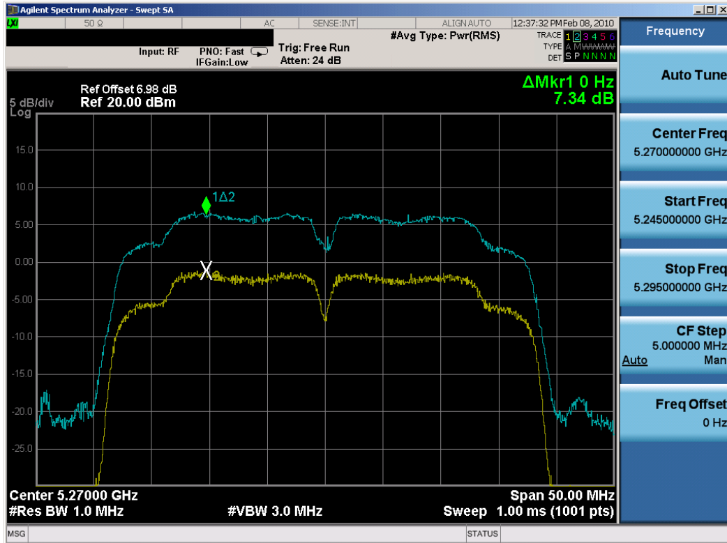
Plot 6-38. Peak Excursion Ratio Plot (802.11n (UNII) – Ch. 54) – Chain B
