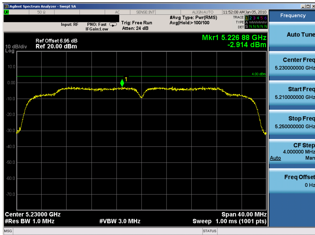
Plot 6-16. Peak Power Spectral Density Plot (802.11n (UNII) – Ch. 46) – Chain A
