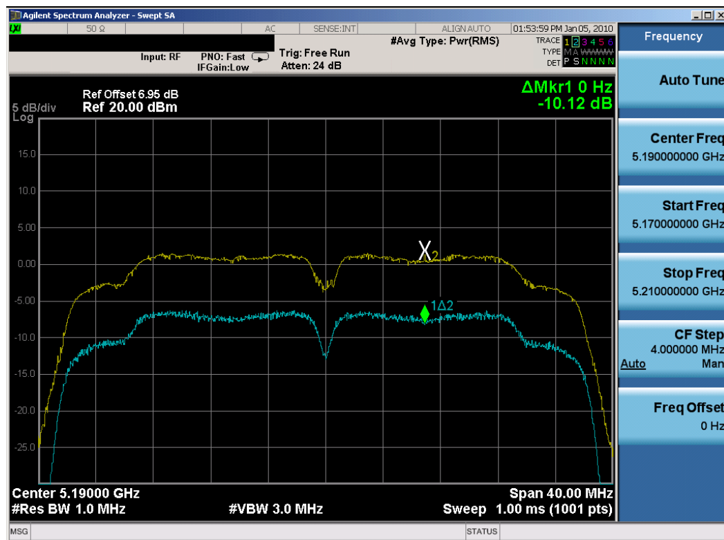
Plot 6-31. Peak Excursion Ratio Plot (802.11n (UNII) – Ch. 38) – Chain A
