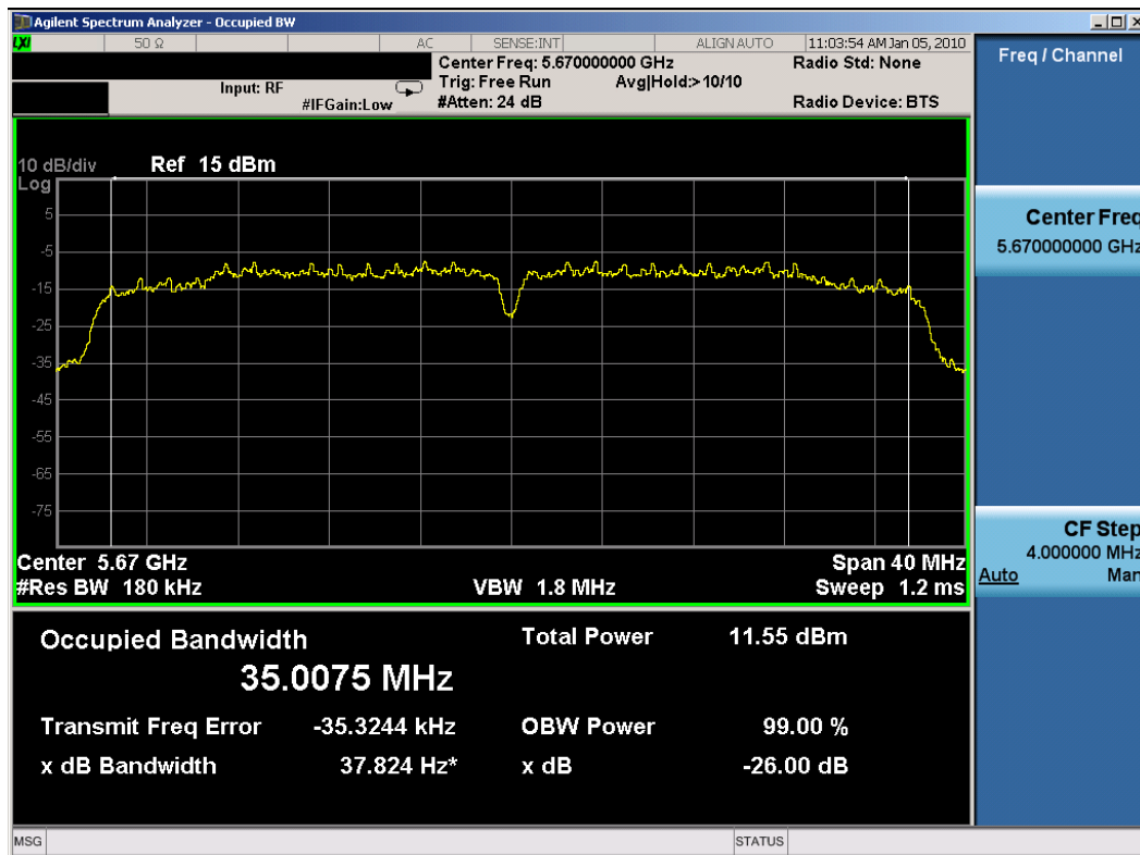
Plot 6-6. 26dB Bandwidth Plot (802.11n (UNII) – Ch. 134) - Chain A
