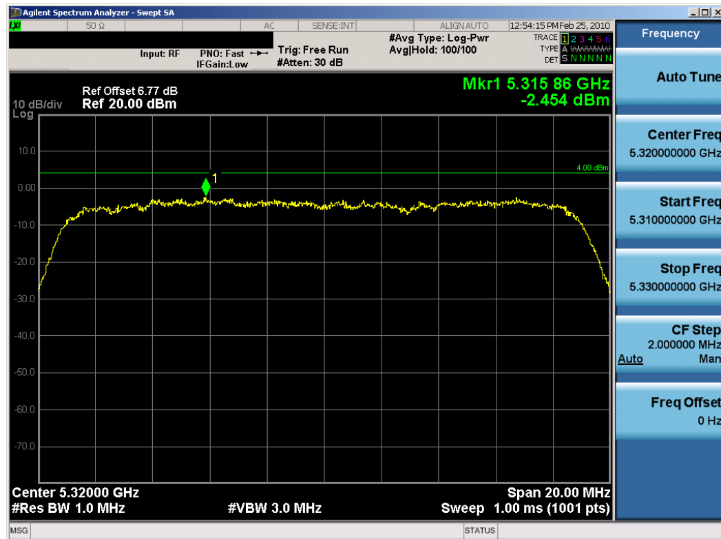
Plot 6-24. Peak Power Spectral Density (802.11a Dual Transmit Mode – Ch. 64) – Chain A
