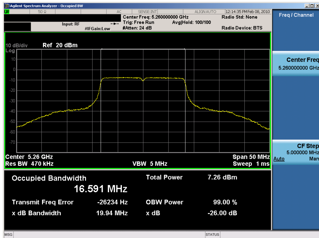
Plot 6-8. 26dB Bandwidth Plot (802.11a (UNII) – Ch. 52) – Chain B
