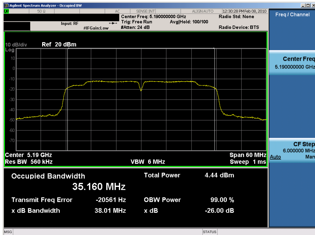
Plot 6-10. 26dB Bandwidth Plot (802.11n (UNII) – Ch. 38) – Chain B
