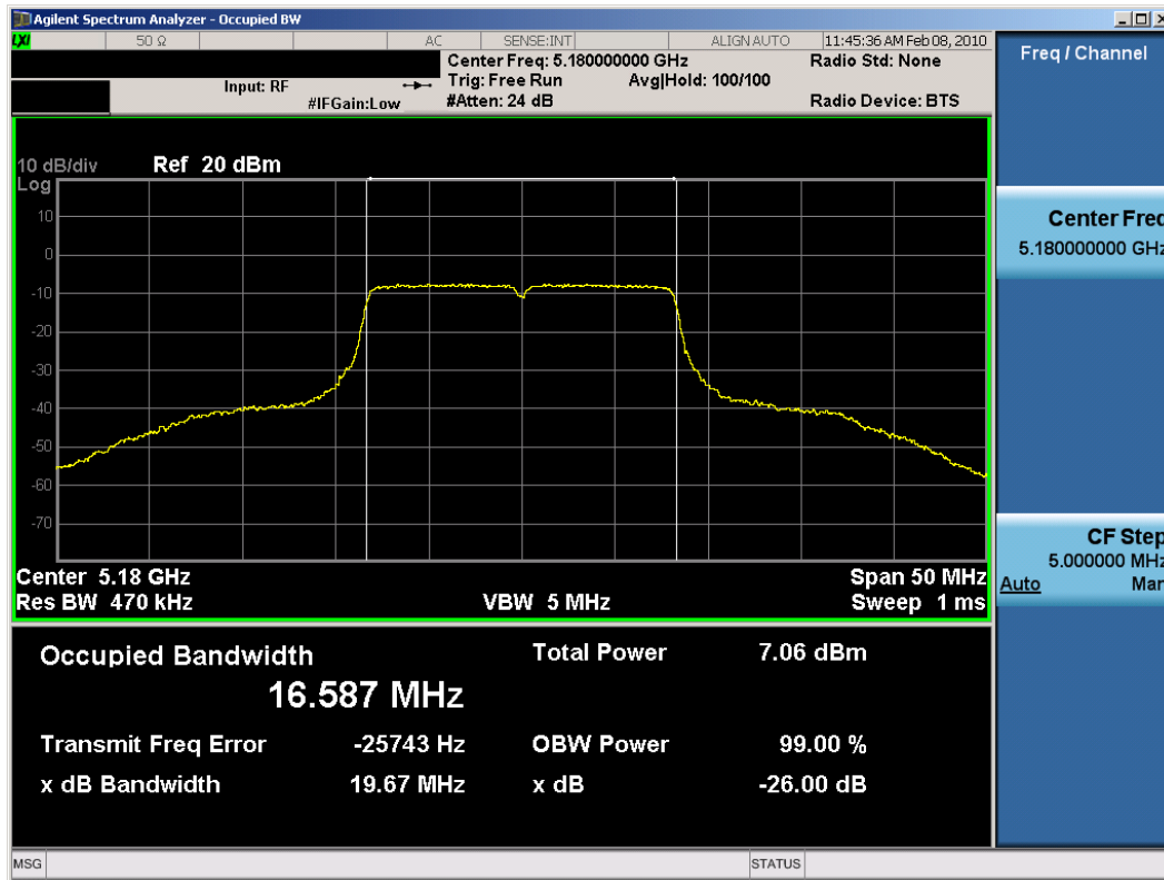
Plot 6-7. 26dB Bandwidth Plot (802.11a (UNII) – Ch. 36) – Chain B
