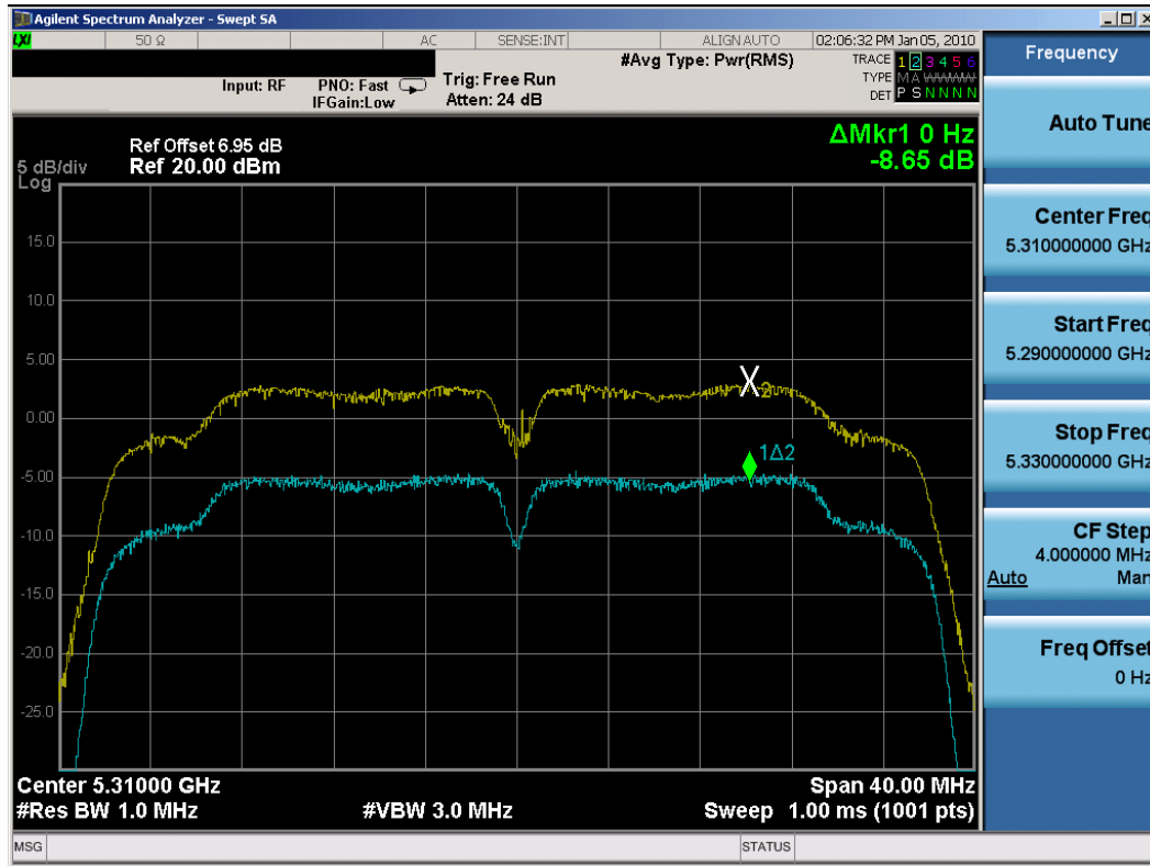
Plot 6-32. Peak Excursion Ratio Plot (802.11n (UNII) – Ch. 62) – Chain A
