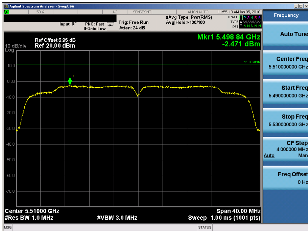
Plot 6-18. Peak Power Spectral Density Plot (802.11n (UNII) – Ch. 102) – Chain A
