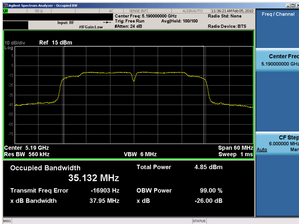
Plot 6-4. 26dB Bandwidth Plot (802.11n (UNII) – Ch. 38) – Chain A
