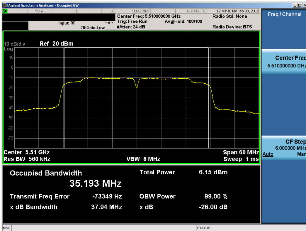
Plot 6-12. 26dB Bandwidth Plot (802.11n (UNII) – Ch. 102) – Chain B
