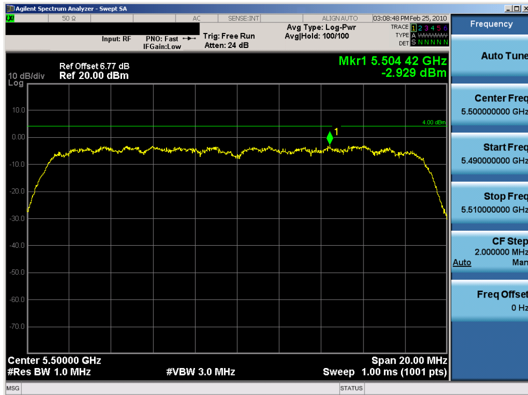
Plot 6-27. Peak Power Spectral Density (802.11a Dual Transmit Mode – Ch. 100) – Chain B
