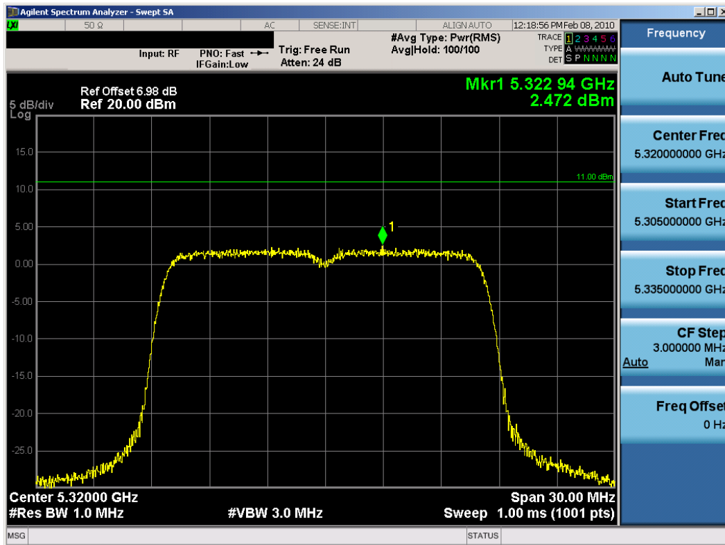
Plot 6-20. Peak Power Spectral Density Plot (802.11a (UNII) - Ch. 64) - Chain B
