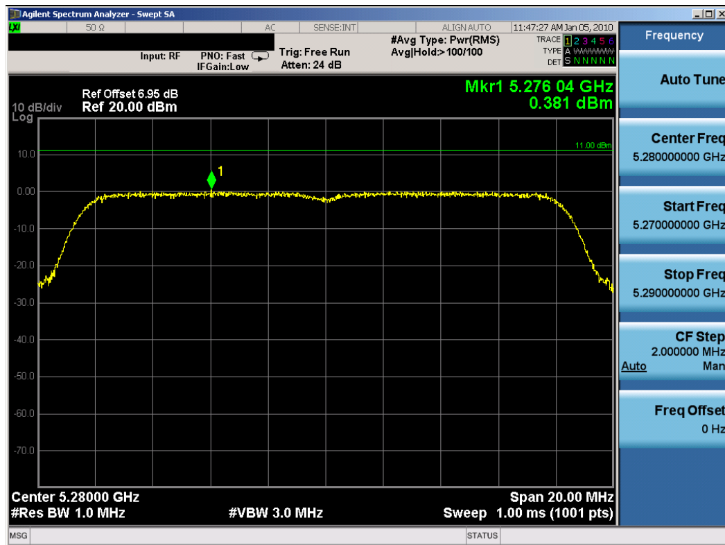
Plot 6-14. Peak Power Spectral Density Plot (802.11a (UNII) – Ch. 56) – Chain A
