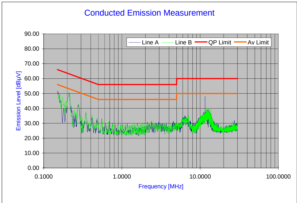
Plot 6-40. Line Conducted Plot with 802.11a (UNII Band I)
