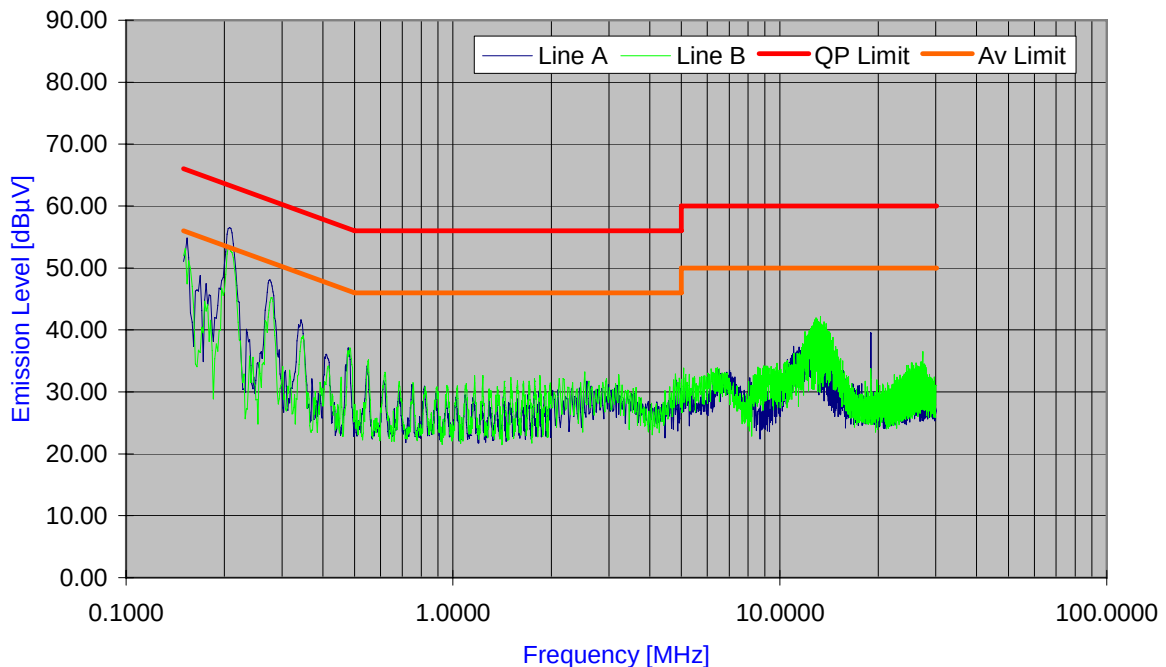
Plot 6-44. Line Conducted Plot with 802.11n (UNII Band II)
