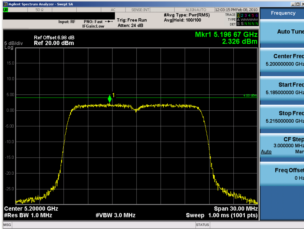
Plot 6-19. Peak Power Spectral Density Plot (802.11a (UNII) - Ch. 40) - Chain B
