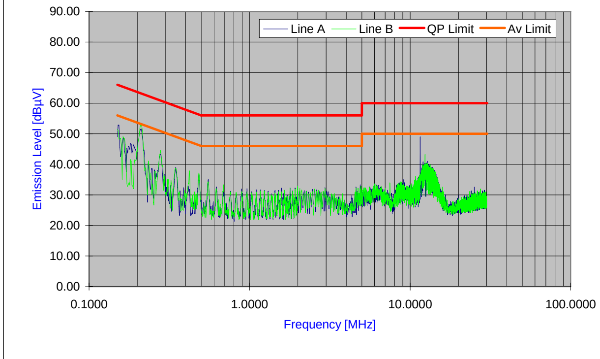
Plot 6-42. Line Conducted Plot with 802.11a (UNII Band III)
