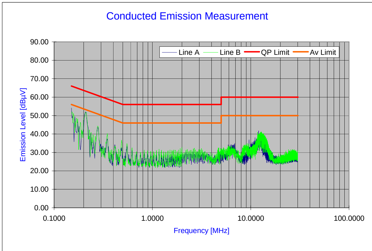
Plot 6-43. Line Conducted Plot with 802.11n (UNII Band I)
