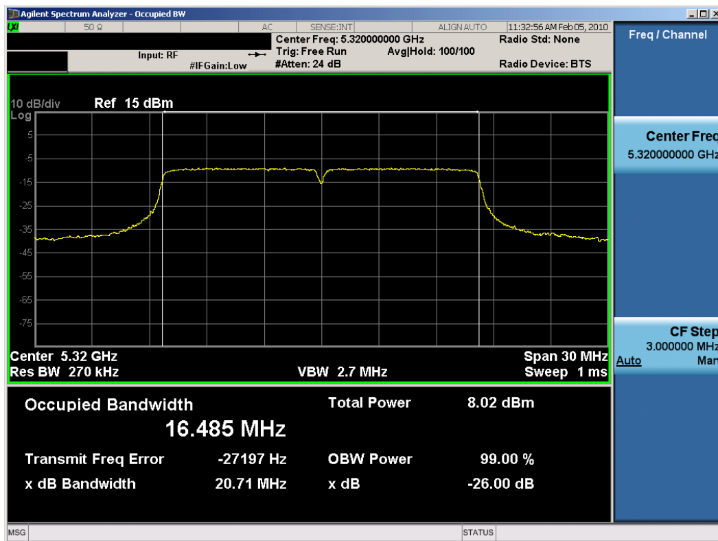
Plot 6-2. 26dB Bandwidth Plot (802.11a (UNII) – Ch. 64) – Chain A
