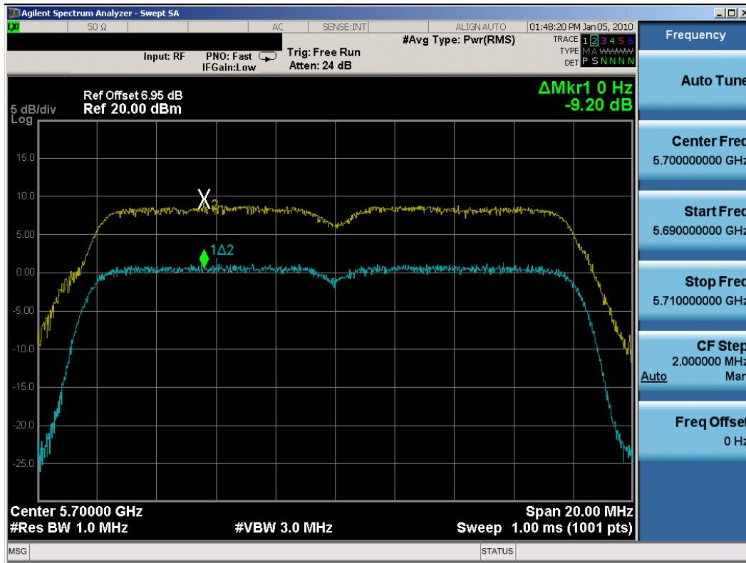
Plot 6-30. Peak Excursion Ratio Plot (802.11a (UNII) – Ch. 140) – Chain A
