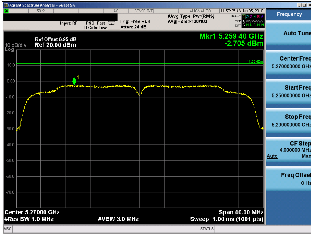
Plot 6-17. Peak Power Spectral Density Plot (802.11n (UNII) – Ch. 54) – Chain A
