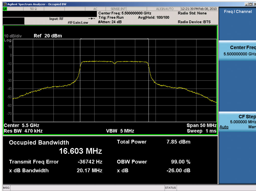
Plot 6-9. 26dB Bandwidth Plot (802.11a (UNII) – Ch. 100) – Chain B
