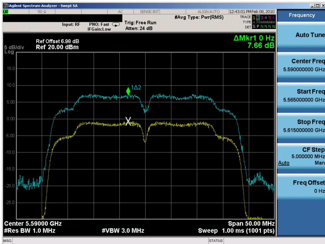
Plot 6-39. Peak Excursion Ratio Plot (802.11n (UNII) – Ch. 118) – Chain B
