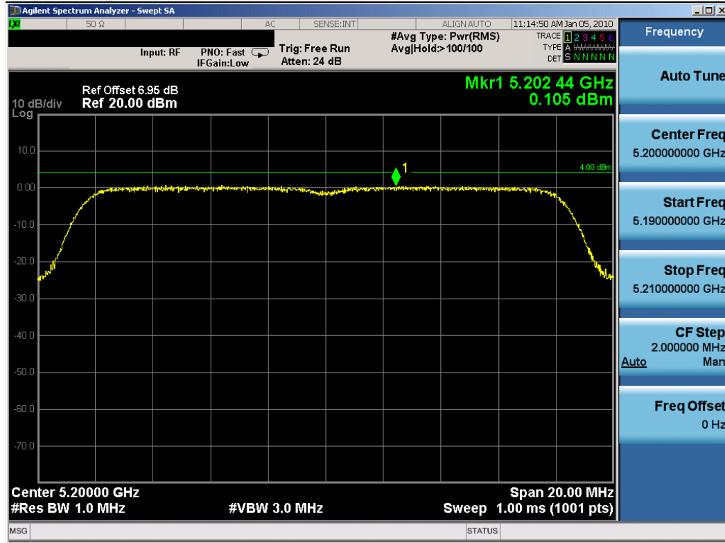
Plot 6-13. Peak Power Spectral Density Plot (802.11a (UNII) – Ch. 40) – Chain A
