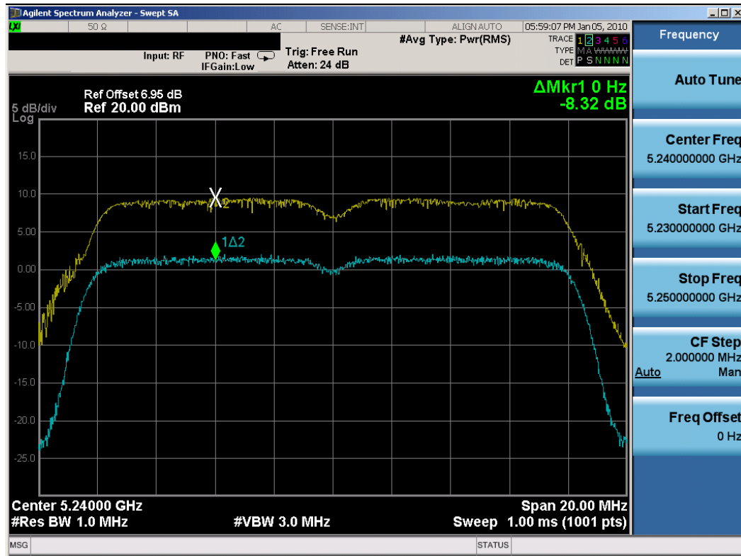
Plot 6-28. Peak Excursion Ratio Plot (802.11a (UNII) – Ch. 48) – Chain A
