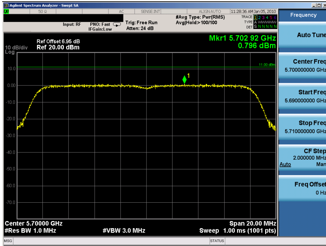
Plot 6-15. Peak Power Spectral Density Plot (802.11a (UNII) – Ch. 140) – Chain A
