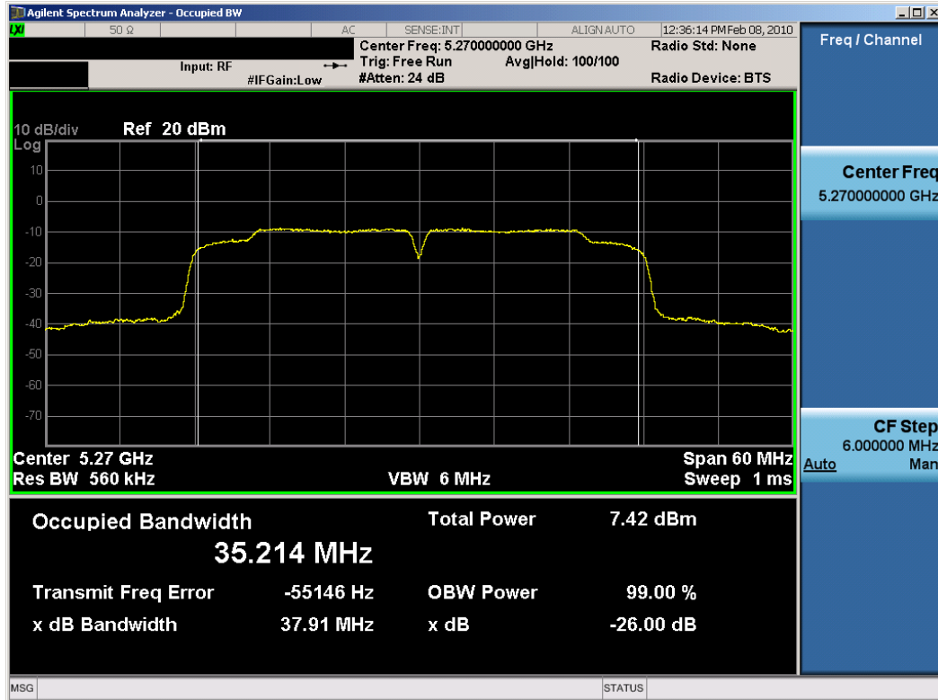
Plot 6-11. 26dB Bandwidth Plot (802.11n (UNII) – Ch. 54) – Chain B
