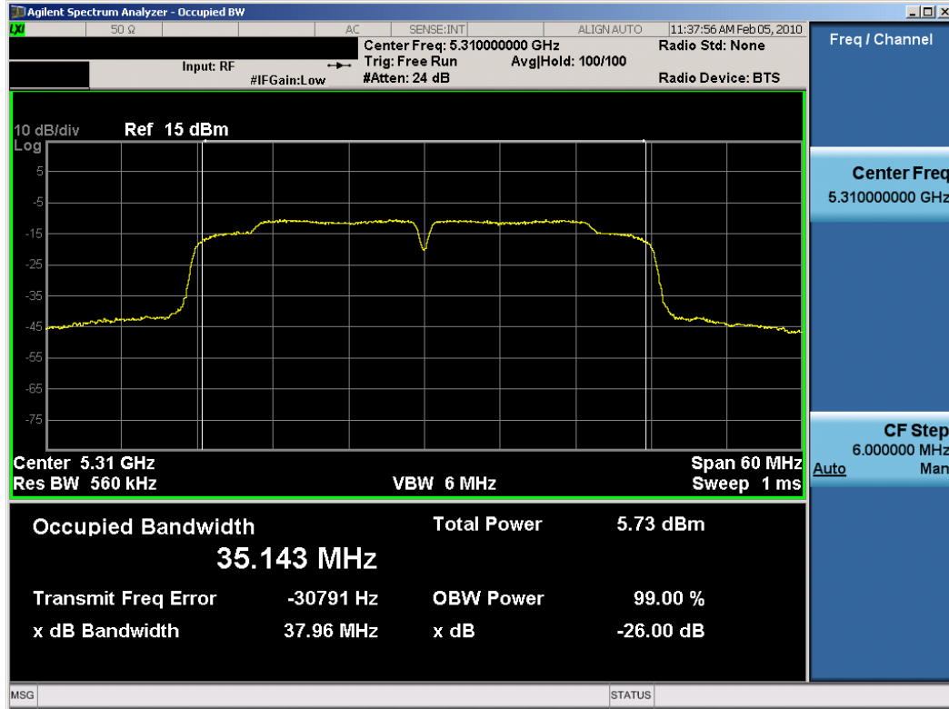
Plot 6-5. 26dB Bandwidth Plot (802.11n (UNII) – Ch. 62) – Chain A
