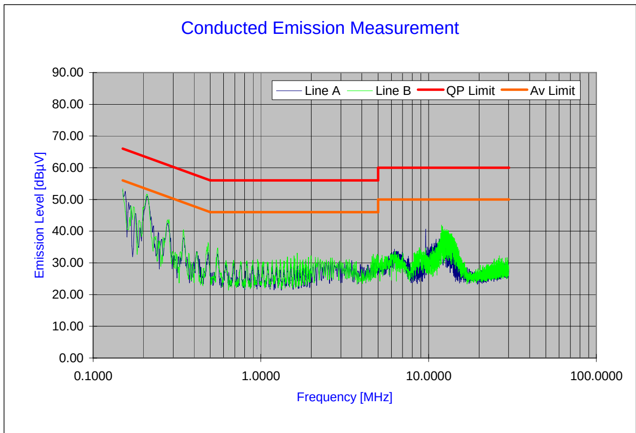
Plot 6-41. Line Conducted Plot with 802.11a (UNII Band II)
