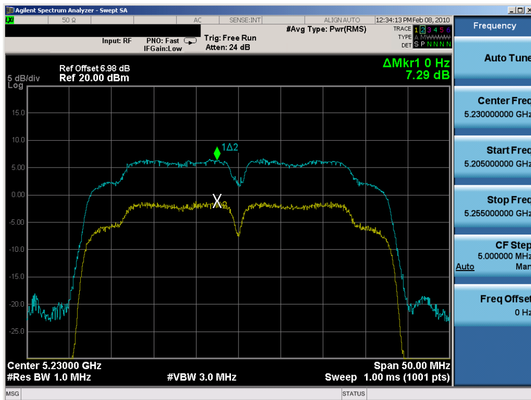
Plot 6-37. Peak Excursion Ratio Plot (802.11n (UNII) – Ch. 46) – Chain B
