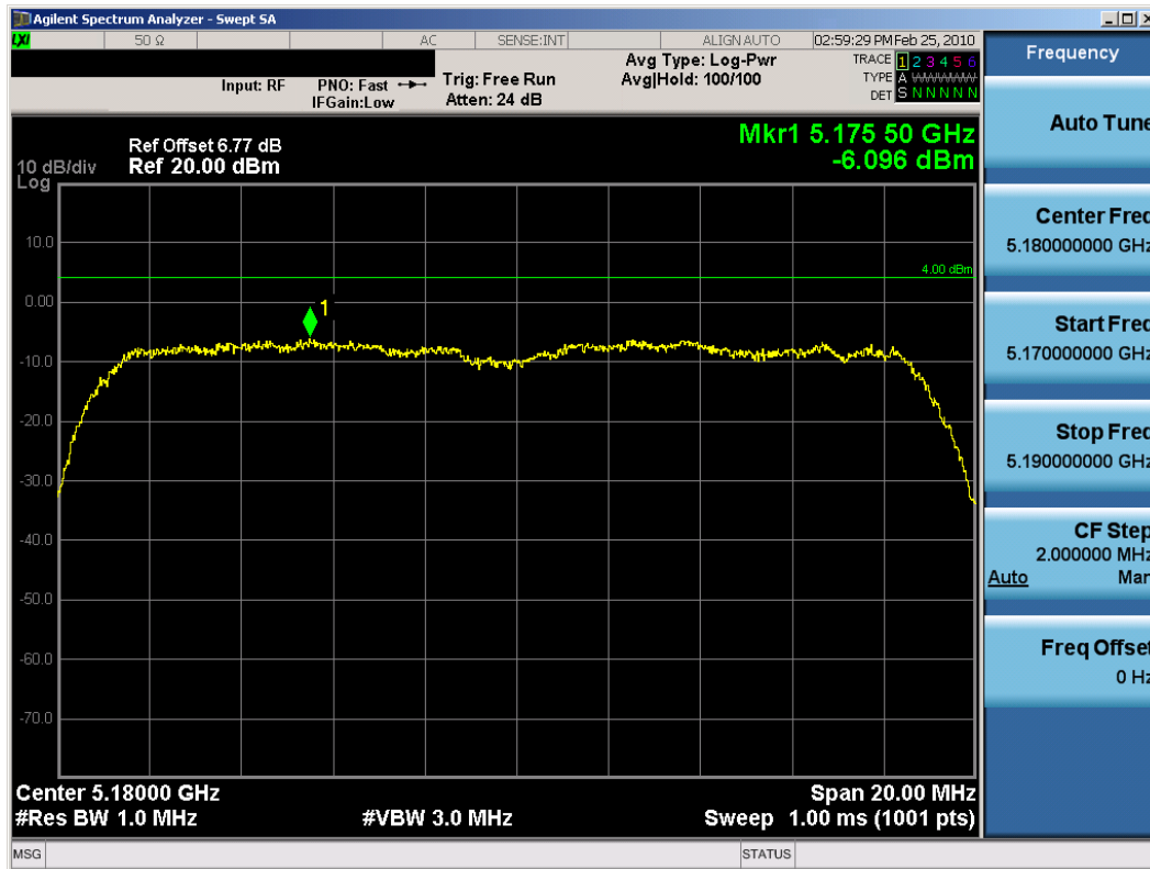
Plot 6-23. Peak Power Spectral Density (802.11a Dual Transmit Mode – Ch. 36) – Chain B
