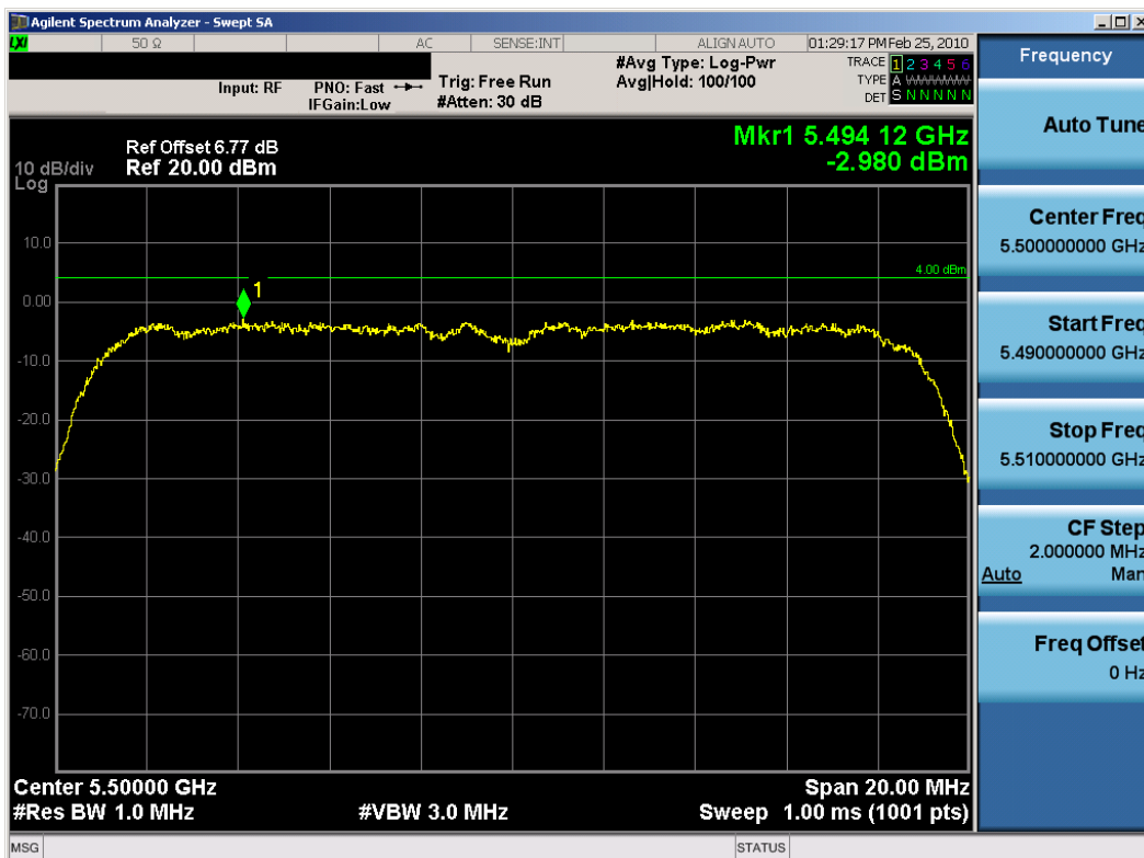
Plot 6-26. Peak Power Spectral Density (802.11a Dual Transmit Mode – Ch. 100) – Chain A
