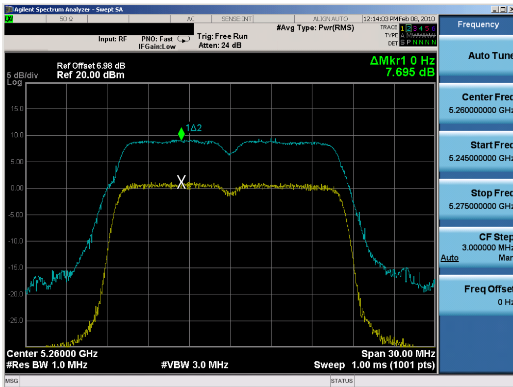
Plot 6-35. Peak Excursion Ratio Plot (802.11a (UNII) - Ch. 52) - Chain B
