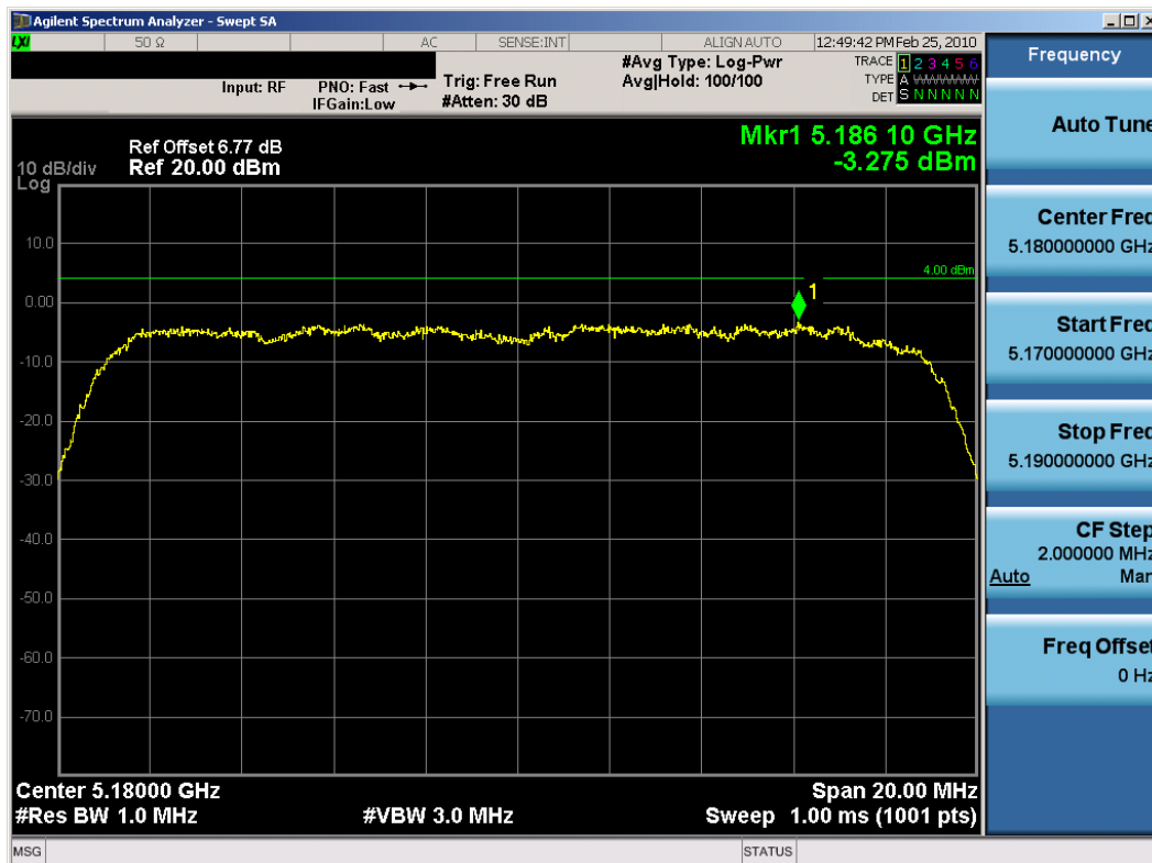
Plot 6-22. Peak Power Spectral Density (802.11a Dual Transmit Mode – Ch. 36) – Chain A
