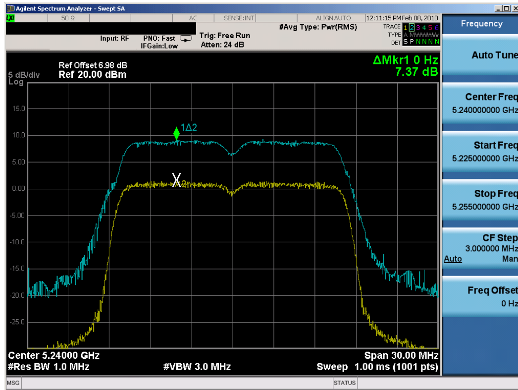
Plot 6-34. Peak Excursion Ratio Plot (802.11a (UNII) - Ch. 48) - Chain B
