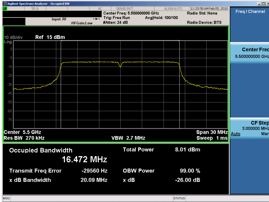
Plot 6-3. 26dB Bandwidth Plot (802.11a (UNII) – Ch. 100) – Chain A
