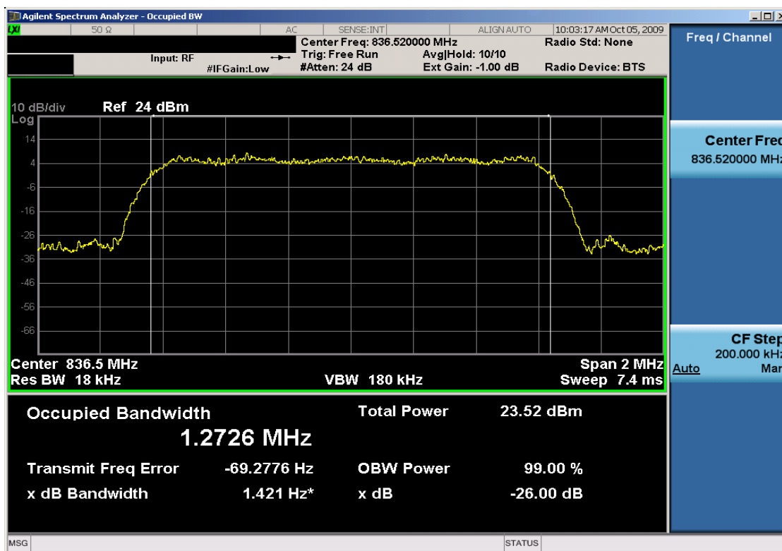
Plot 7-52. Occupied Bandwidth Plot (Cellular CDMA Mode – Ch. 384)
