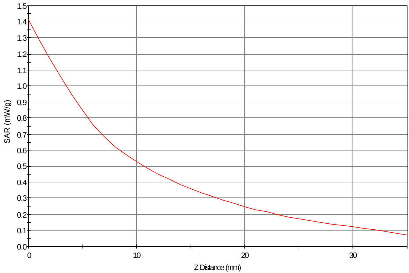
SAR - Z Axis at Hotspot x:-14.0 y:-24.0
