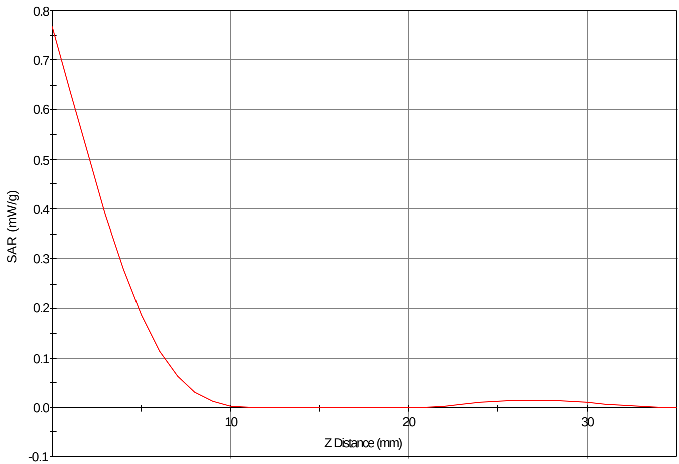
SAR - Z Axis at Hotspot x:-27.0 y:-18.0
