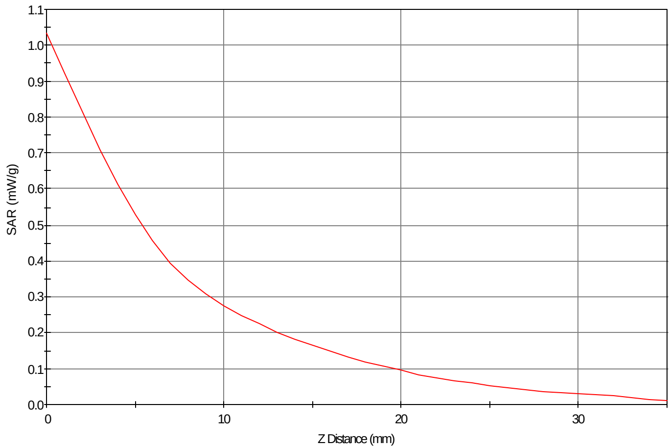
SAR - Z Axis at Hotspot x:-3.0 y:-32.0
