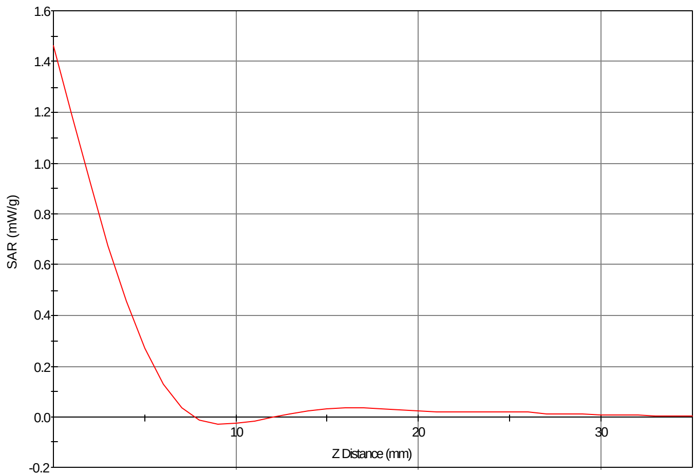
SAR - Z Axis at Hotspot x:-20.0 y:-24.0
