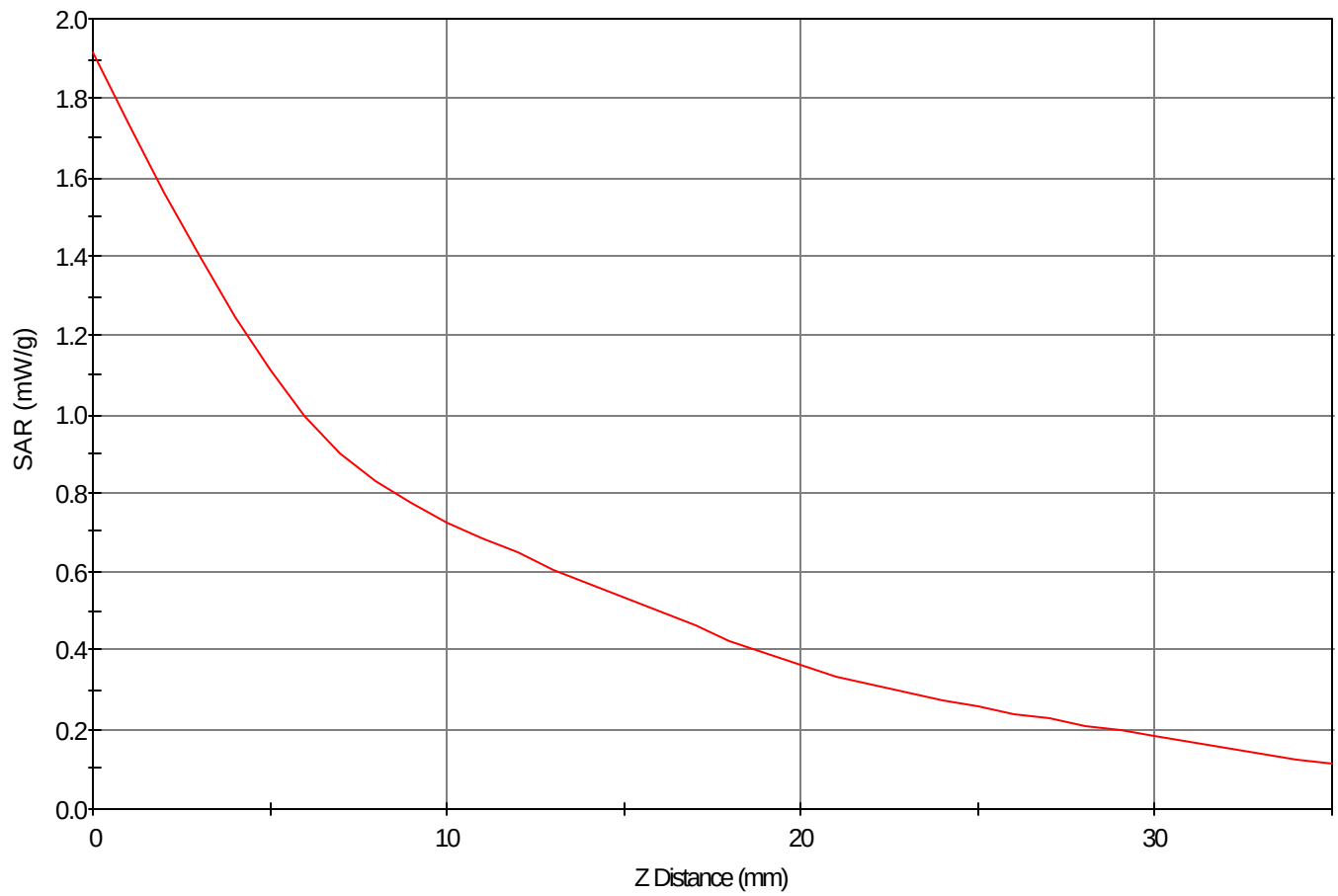
SAR - Z Axis at Hotspot x:-3.0 y:-25.0
