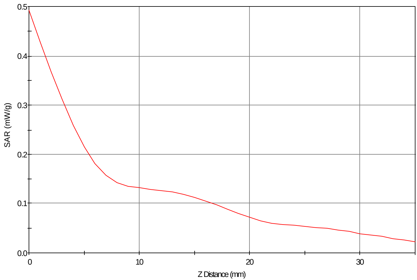
SAR - Z Axis at Hotspot x:13.0 y:40.0
