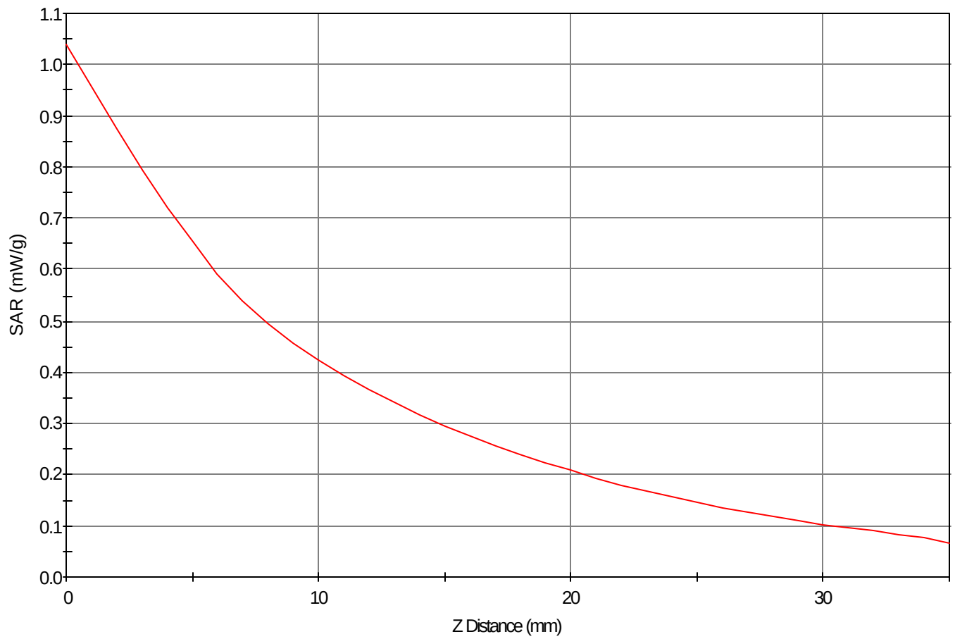
SAR - Z Axis at Hotspot x:-5.0 y:-22.0
