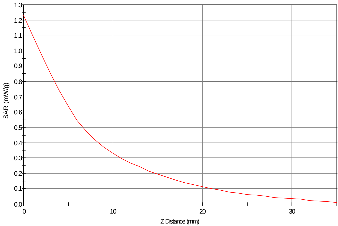
SAR - Z Axis at Hotspot x:-4.0 y:-31.0
