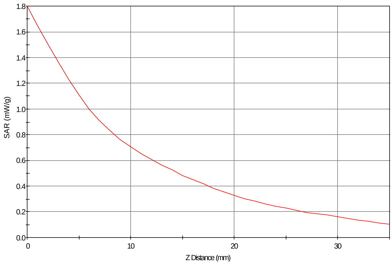
SAR - Z Axis at Hotspot x:13.0 y:69.0
