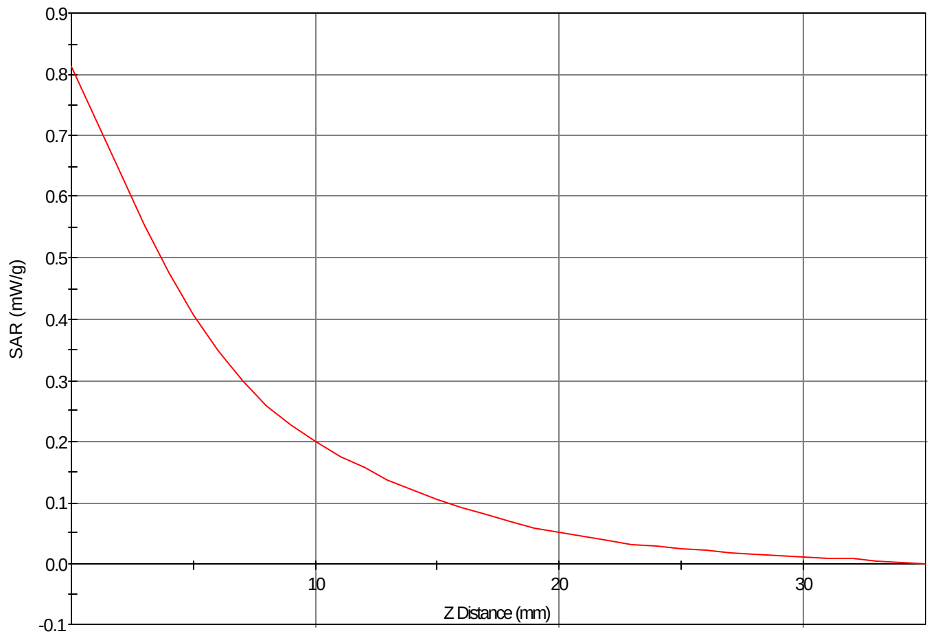
SAR - Z Axis at Hotspot x:13.0 y:43.0
