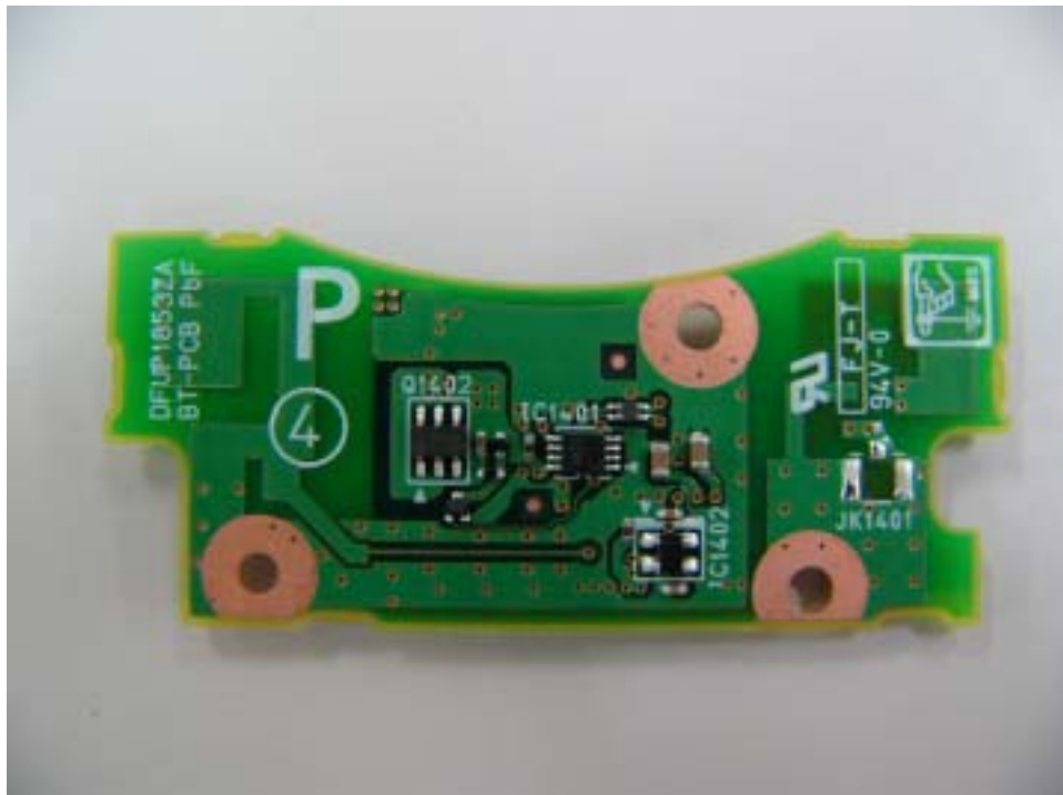
Bluetooth Card inside Top View
