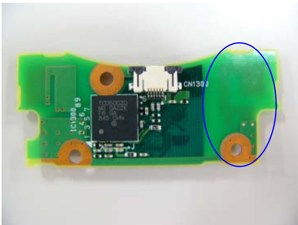
Bluetooth TX/RX Antenna (separated type: Bottom)
