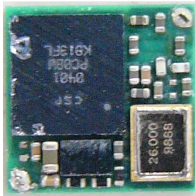
Bluetooth chip inside Top View
