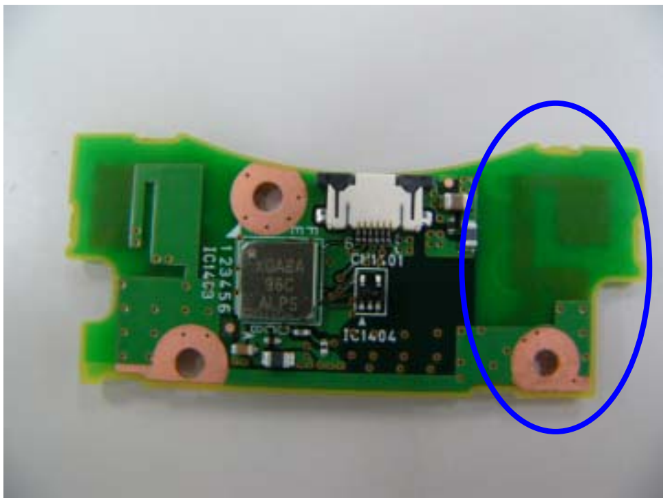
Bluetooth TX/RX Antenna (integrated type: Bottom)
