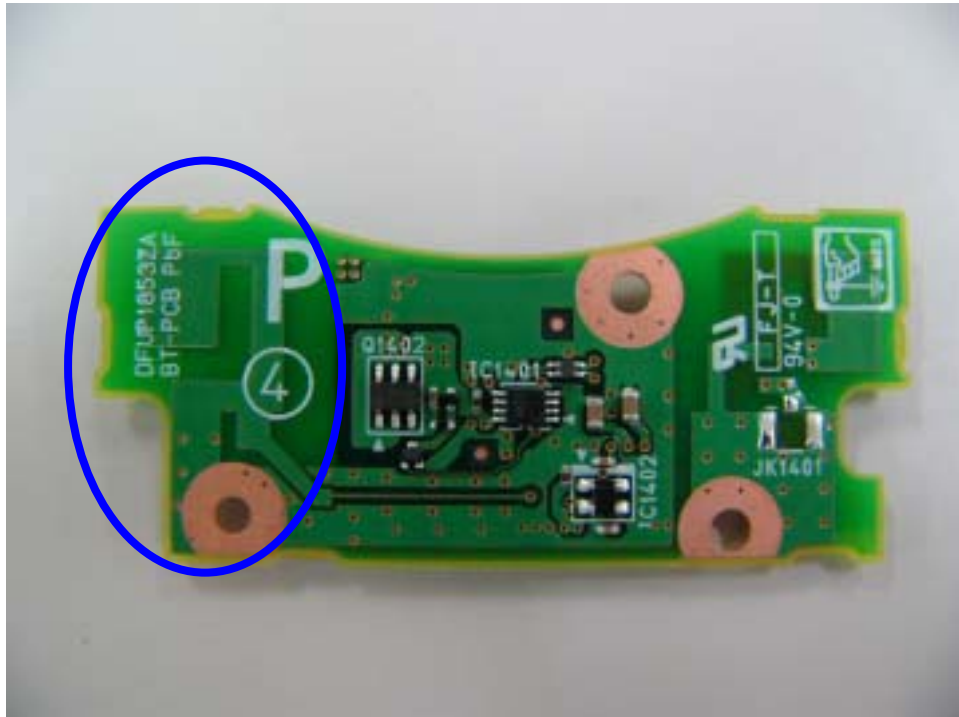
Bluetooth TX/RX Antenna(integrated type: Top )
