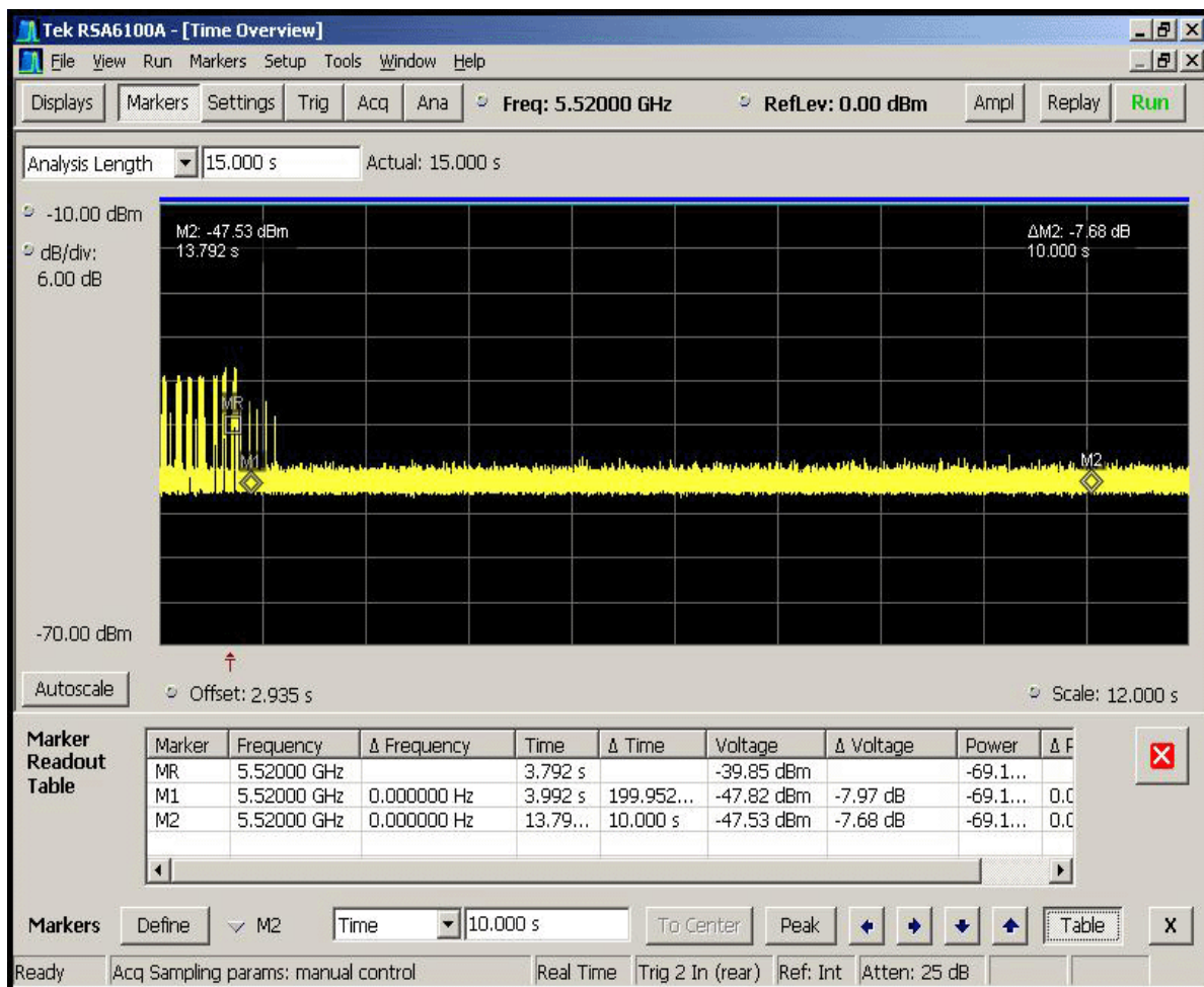
Figure 6-4. Channel Move Time (< 10sec)
