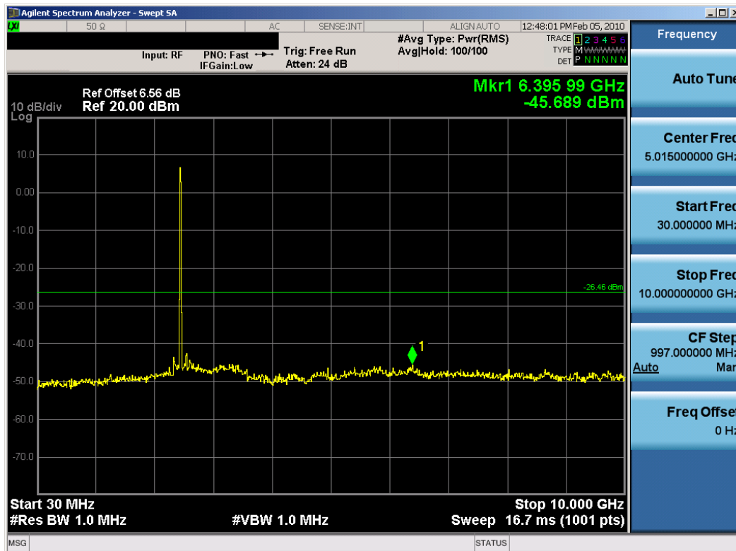
Plot 6-68. Conducted Spurious Plot (802.11g – Ch. 11) – Chain B
