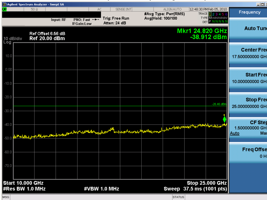
Plot 6-69. Conducted Spurious Plot (802.11g – Ch. 11) – Chain B
