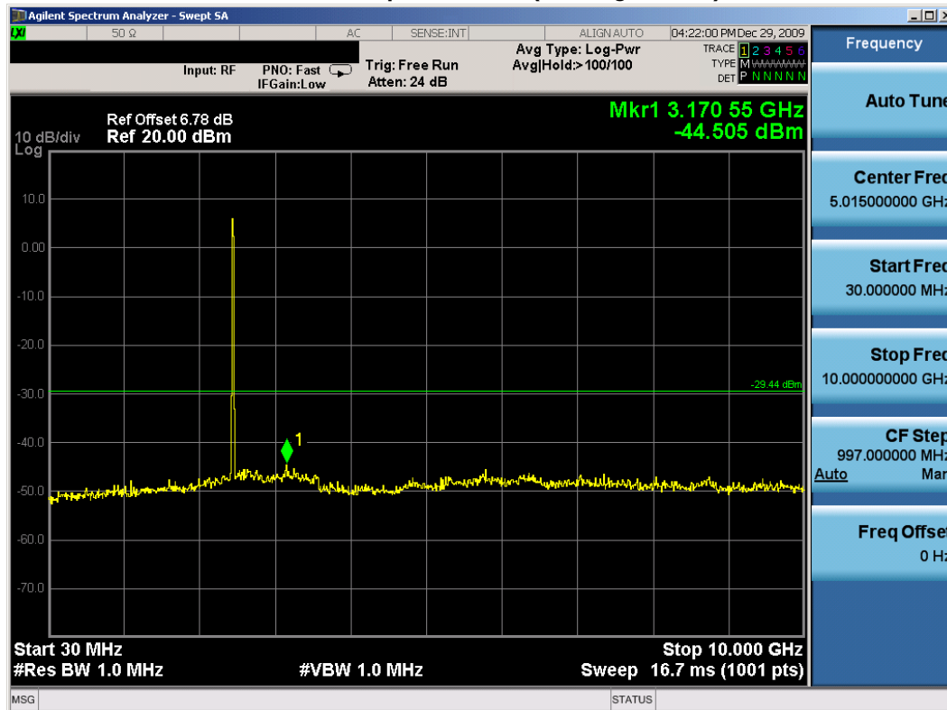
Plot 6-53. Conducted Spurious Plot (802.11g – Ch. 11) – Chain A
