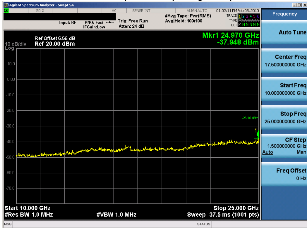
Plot 6-67. Conducted Spurious Plot (802.11g – Ch. 6) – Chain B
