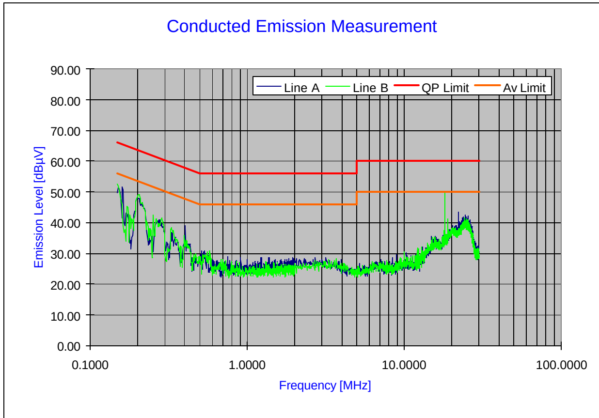
Plot 6-79. Line Conducted Plot with 802.11n
