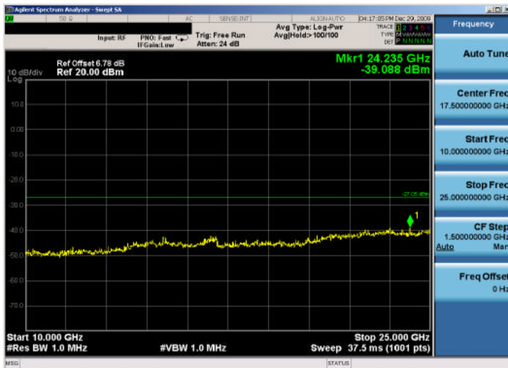
Plot 6-50. Conducted Spurious Plot (802.11g – Ch. 1) – Chain A
