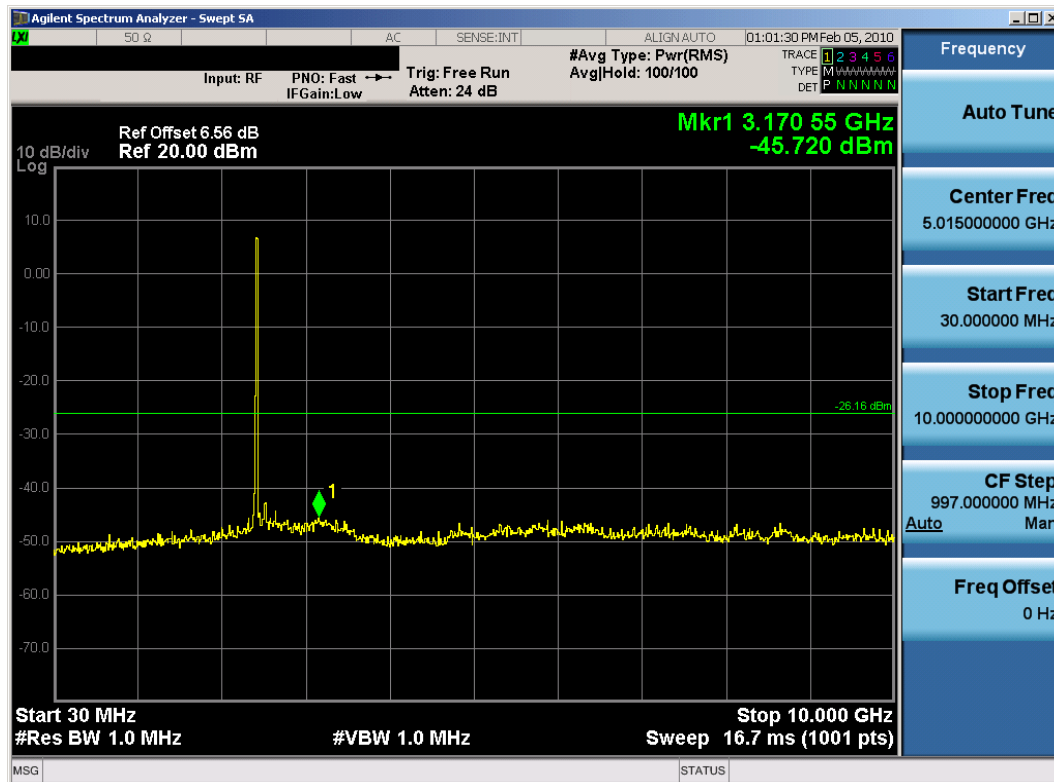
Plot 6-66. Conducted Spurious Plot (802.11g – Ch. 6) – Chain B
