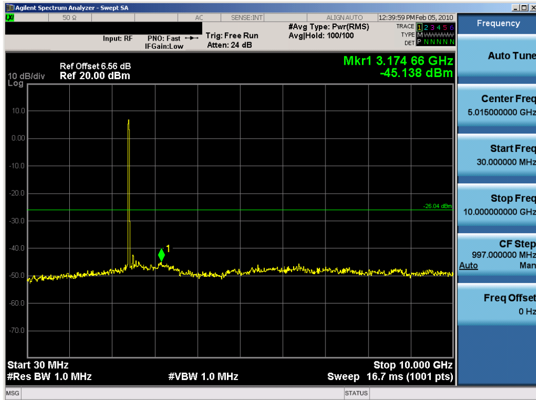
Plot 6-64. Conducted Spurious Plot (802.11g - Ch. 1) - Chain B
