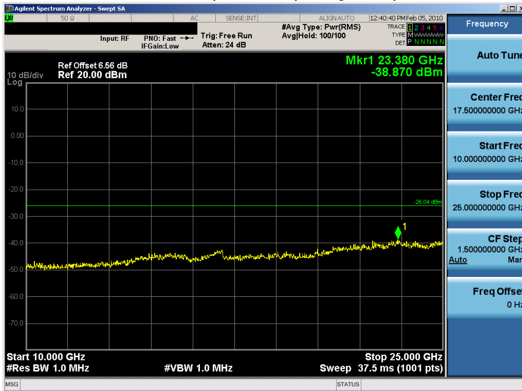
Plot 6-65. Conducted Spurious Plot (802.11g - Ch. 1) - Chain B
