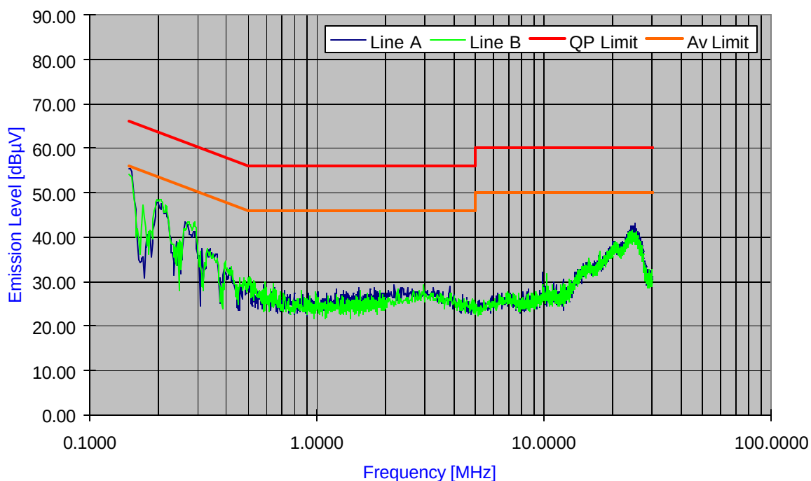
Plot 6-76. Line Conducted Plot with 802.11b
