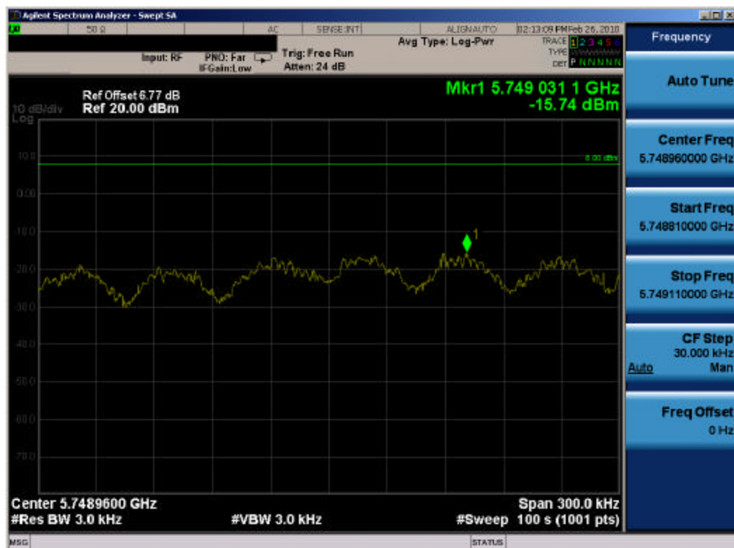
Plot 6-24. Power Spectral Density (802.11a Dual Transmit Mode – Ch. 149) – Chain B
