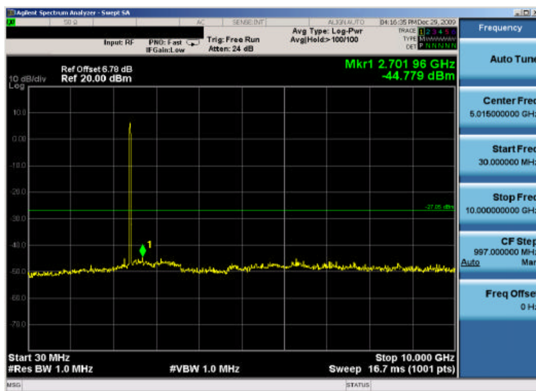
Plot 6-49. Conducted Spurious Plot (802.11g – Ch. 1) – Chain A
