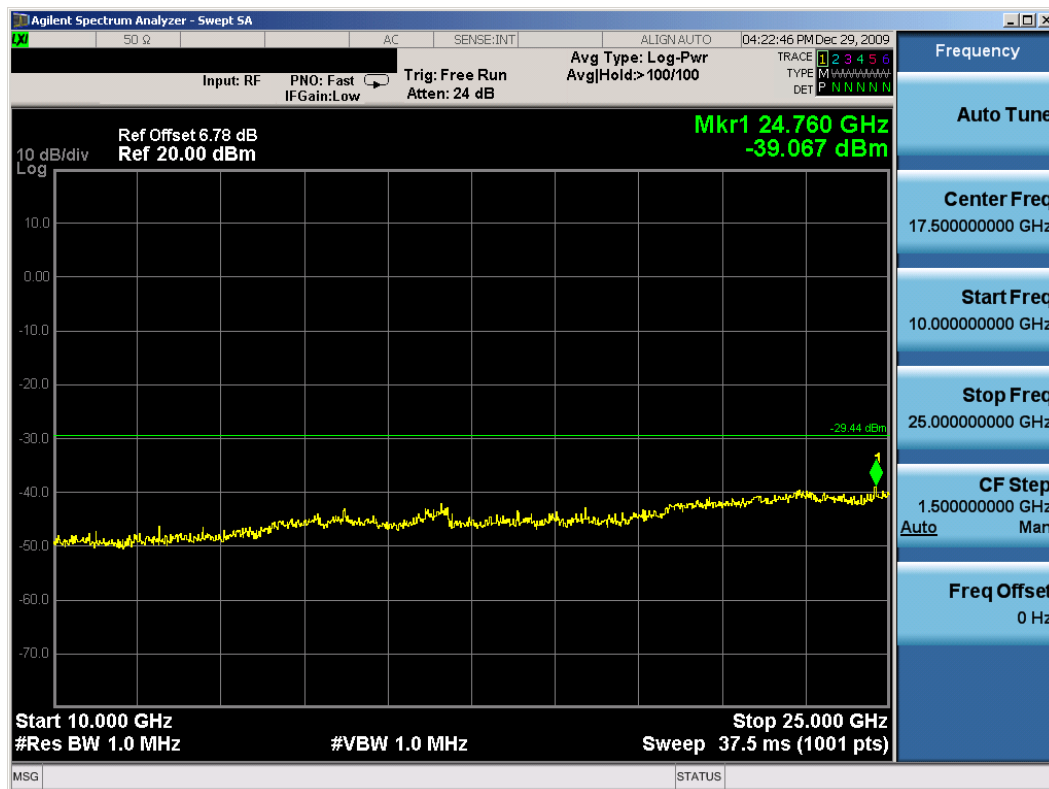
Plot 6-54. Conducted Spurious Plot (802.11g – Ch. 11) – Chain A
