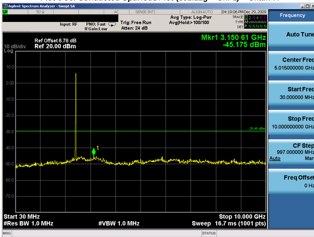
Plot 6-51. Conducted Spurious Plot (802.11g – Ch. 6) – Chain A
