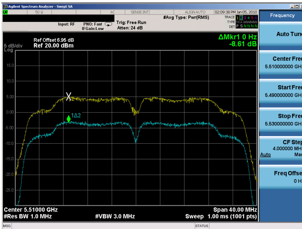
Plot 6-33. Peak Excursion Ratio Plot (802.11n (UNII) – Ch. 102) – Chain A
