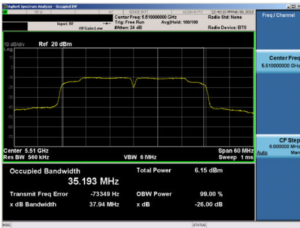
Plot 6-12. 26dB Bandwidth Plot (802.11a/n (UNII) - Ch. 102) - Chain B
