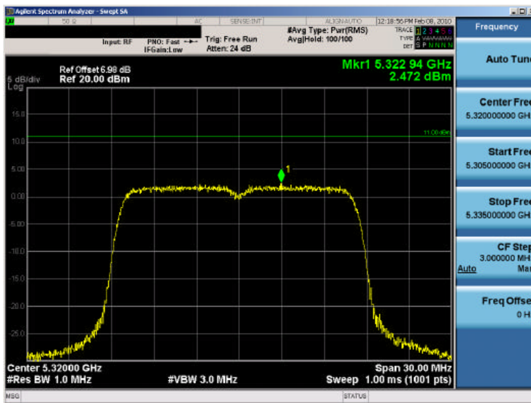
Plot 6-20. Peak Power Spectral Density Plot (802.11a (UNII) – Ch. 64) – Chain B
